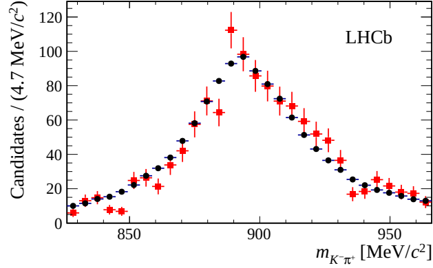
Figure 4: Efficiency corrected m_{K^-\pi^+} distribution for B_s^0 shown in squares (red) and \bar{B}^0 shown in circles (black) using sWeights computed from the maximum likelihood fit to the J/\psi K^-\pi^+ invariant mass spectrum.
