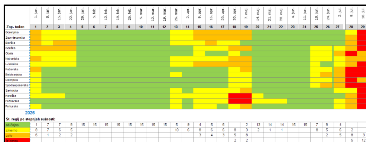
Figure A4.4.1: Timeline of weekly published early warnings for drought in the topsoil layer between January and mid-July 2026 (ARSO, 2026).
