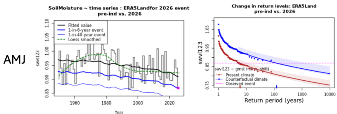
Figure 2.5: Left - Annual time series of Apr-Jun soil moisture in ERA5 for the Western Domain. The ERA5 event is shown with the pink box. The loess-smoothed trend is shown with the green dashed line and the fitted statistical model that varies with GMST is shown with the black and blue lines, showing the event (black line), and the 1-in-6 (bold blue) and 1-in-40-year (lighter blue) return period event magnitudes. Right - Statistical fits to Apr-Jun soil moisture in ERA5-Land for the Western Domain. The probability curve for the current climate is shown in red, and for the past 1.4°C climate in blue, with the shaded band showing the 95% confidence interval. The magnitude of the studied event is highlighted with a horizontal pink line. Red and blue markers on the return-period axis mark the return period for an event of the 2026 magnitude in the current and past climate respectively.
