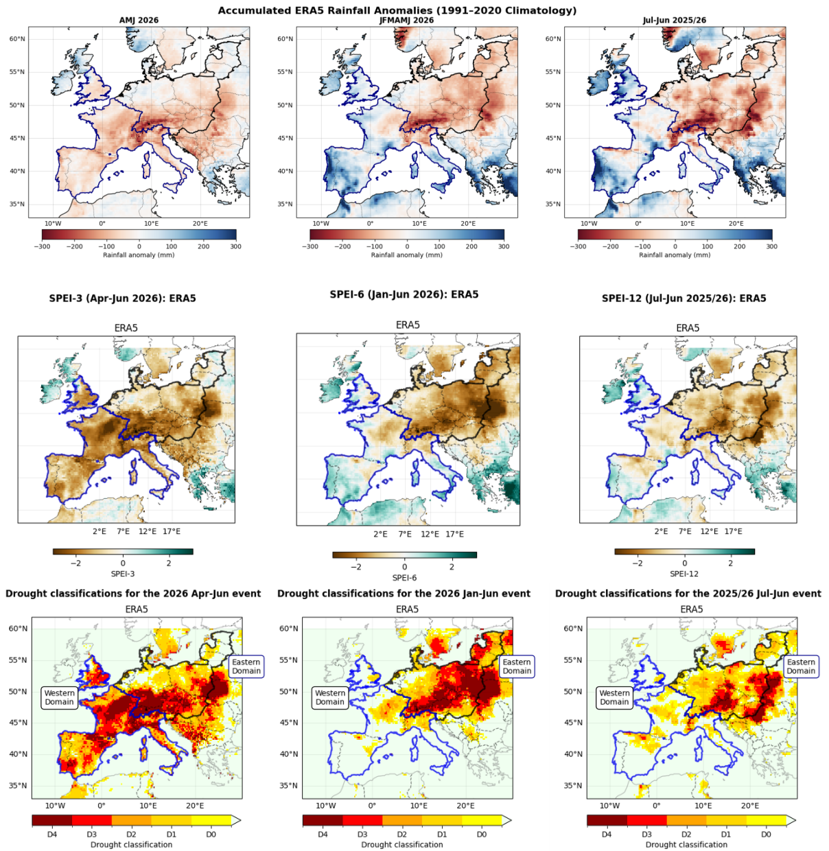
Figure 1.3 Top: Precipitation anomalies wrt 1991-2020 for 3-, 6- and 12-month accumulated precipitation ending in June 2026. Middle: SPEI maps for 3-, 6- and 12- month accumulation periods ending in June 2026 over the region 33-60°N, 15°W-30°E. The Western Domain is highlighted in blue and the Eastern Domain is highlighted in black. Bottom: Drought classification maps categorised according to the US Drought Monitor (USDM) system. The categories are based on the n -month SPEI values in June 2026, calculated from ERA5 using the Hargreaves scheme for PET.
