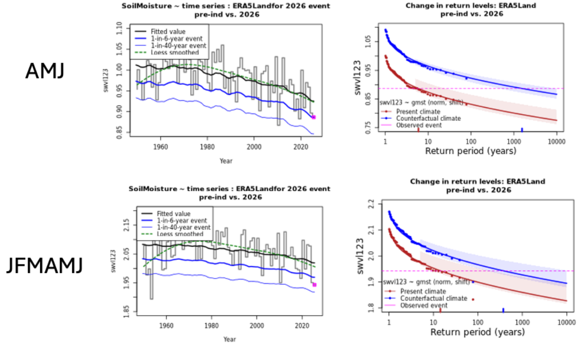
Figure 2.6: Same as for Fig. 2.5 but for the Eastern Domain for AMJ (top row) and JFAMJ seasons (bottom row).
