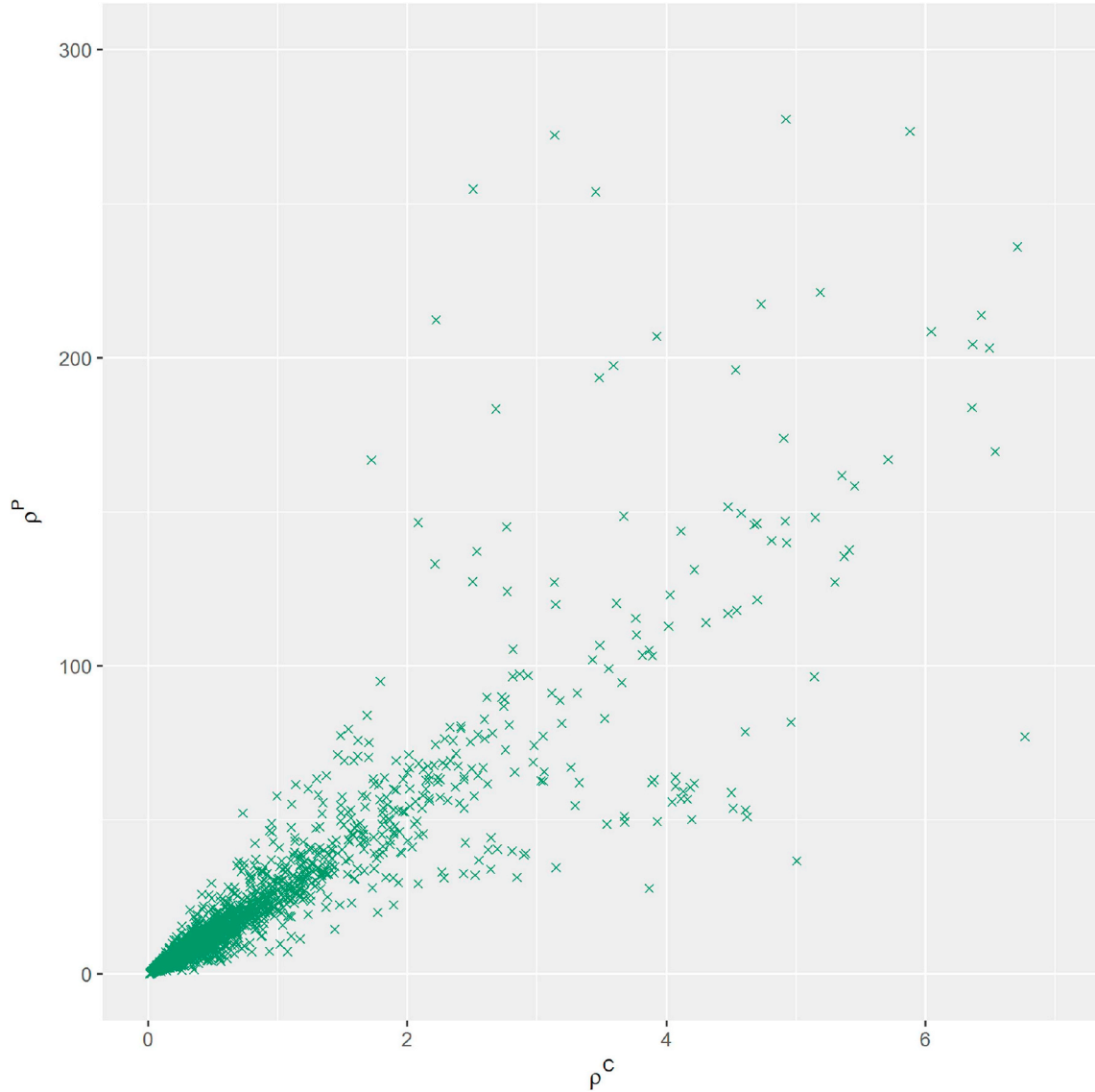
Fig. 8. Scatterplot of MED values for TfL zones with impedance measured by highway GC ( \rho^C ) and public transport GC ( \rho^P ).
