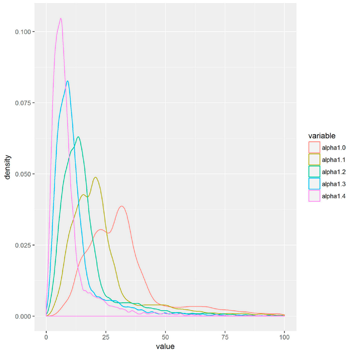
Fig. 10. Densities for distance based MED with different distance decay values.
