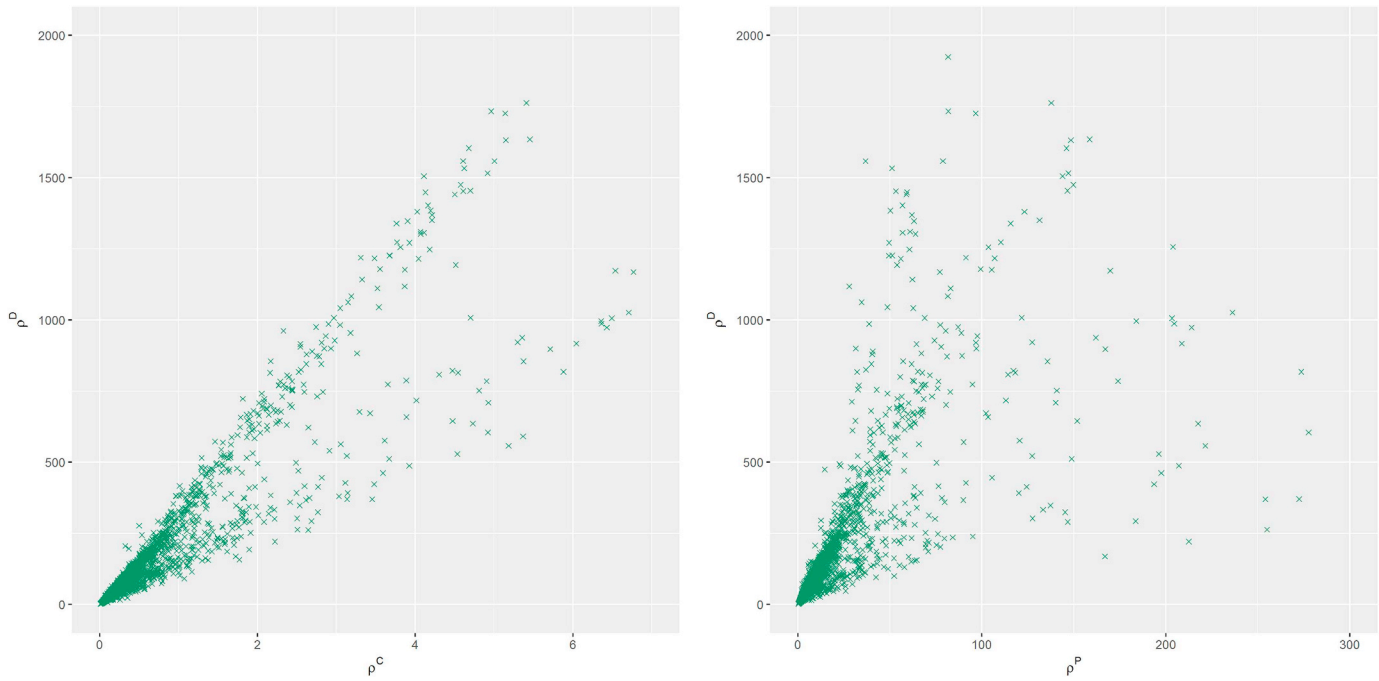
Fig. 9. Scatterplots of MED values for TfL zones with impedance measured by highway GC ( \rho^C ) and public transport GC ( \rho^P ) against distance ( \rho^D ).
