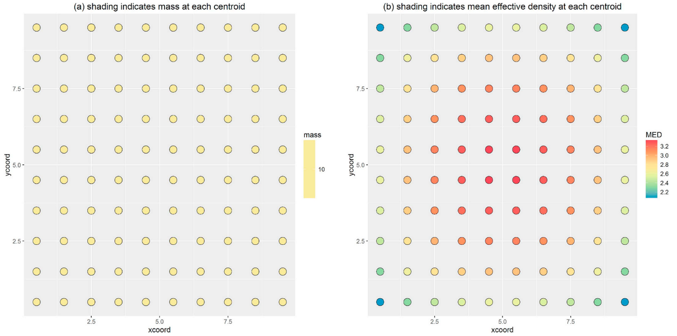
Fig. 3. MED values for zones of a constant size formed as a uniform grid.
