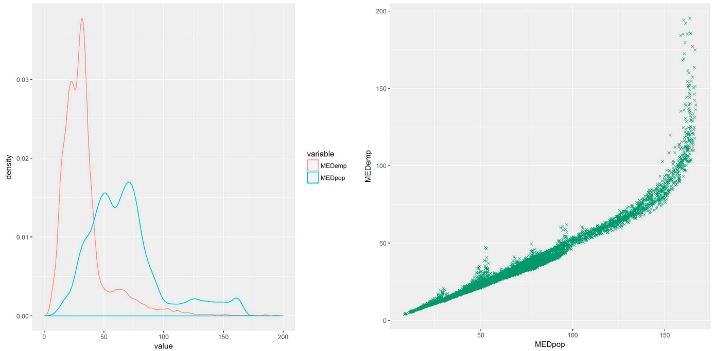
Fig. 7. Densities and a scatterplot of MED values for Britain with mass measured by population and employment.
