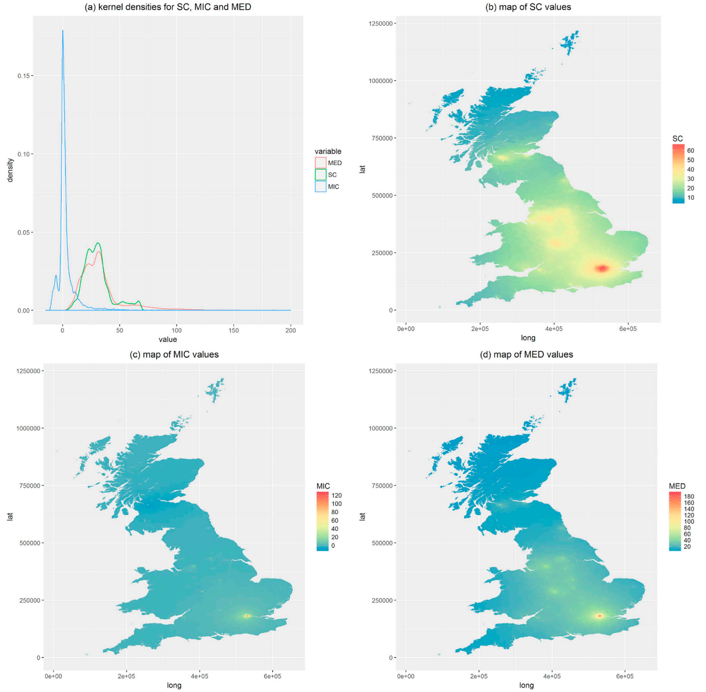
Fig. 6. Components of MED values for Britain with total employment as mass.
