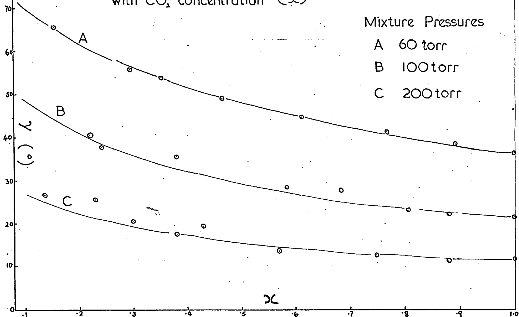
FIG. 30 Results for \text{CO}_2 —Ne Mixtures ( 4.3\mu band) Variation of Relaxation Phase Shift ( \gamma ) with \text{CO}_2 concentration ( x )
