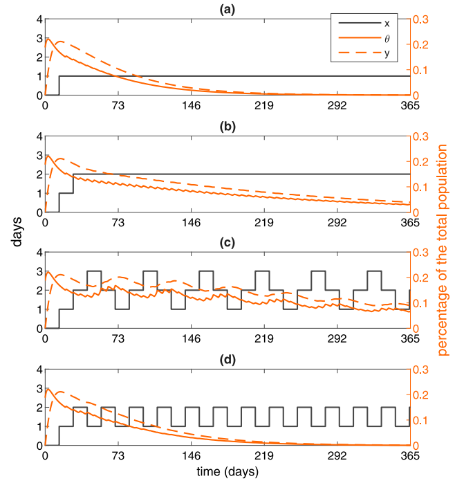
Fig. 3. Time series of the decision variable x , the observed variable y and the controlled variable \theta obtained with \varepsilon^1 = \varepsilon^l = 0 and with (a) (a^1, a^l) = (0.3, 0.3) , (b) (a^1, a^l) = (0.3, 0.9) , (c) (a^1, a^l) = (0.3, 2.7) , and (d) (a^1, a^l) = (0.9, 2.1) .
