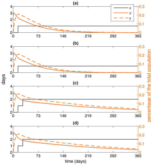
Fig. 4. Time series of the decision variable x , the observed variable y and the controlled variable \theta obtained with \epsilon^\dagger = \epsilon^\downarrow = 10^{-4} and with (a) (a^\dagger, a^\downarrow) = (0.3, 0.3) , (b) (a^\dagger, a^\downarrow) = (0.3, 0.9) , (c) (a^\dagger, a^\downarrow) = (0.3, 2.7) , and (d) (a^\dagger, a^\downarrow) = (0.9, 2.1) .
