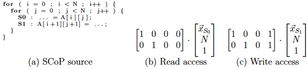
Figure 3.6: Example showing how array access functions are captured by the polyhedral model
