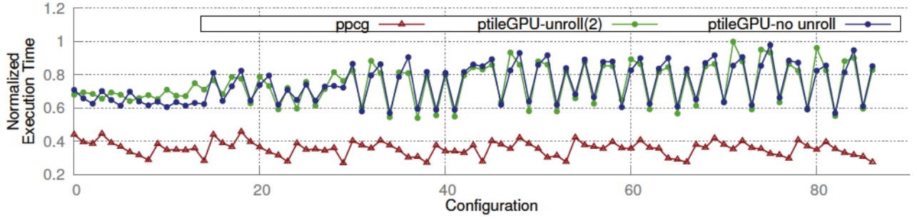
(f) With local memory and unrolling optimization. Worst execution time 0.759sec.
