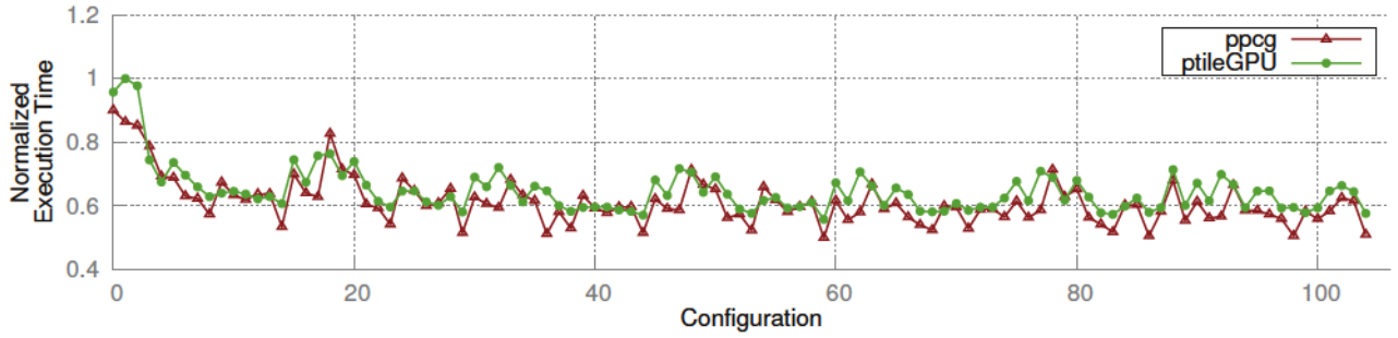
(c) With local memory. Worst execution time 0.234sec.
