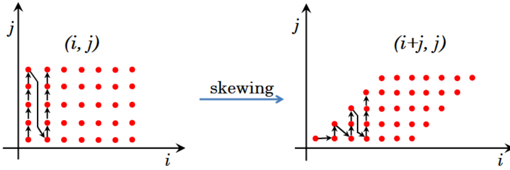
Figure 3.4: Loop skewing in the polyhedral model.
