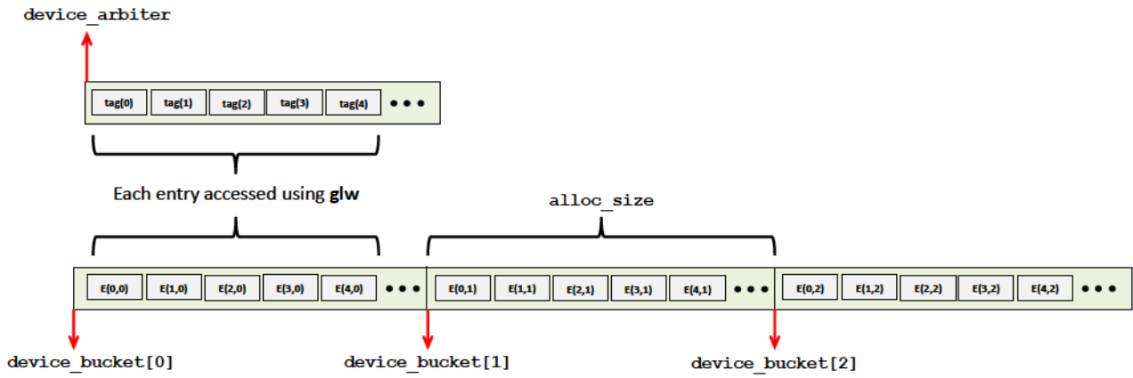
Figure 7.3: Storage layout of a tile bucket.
