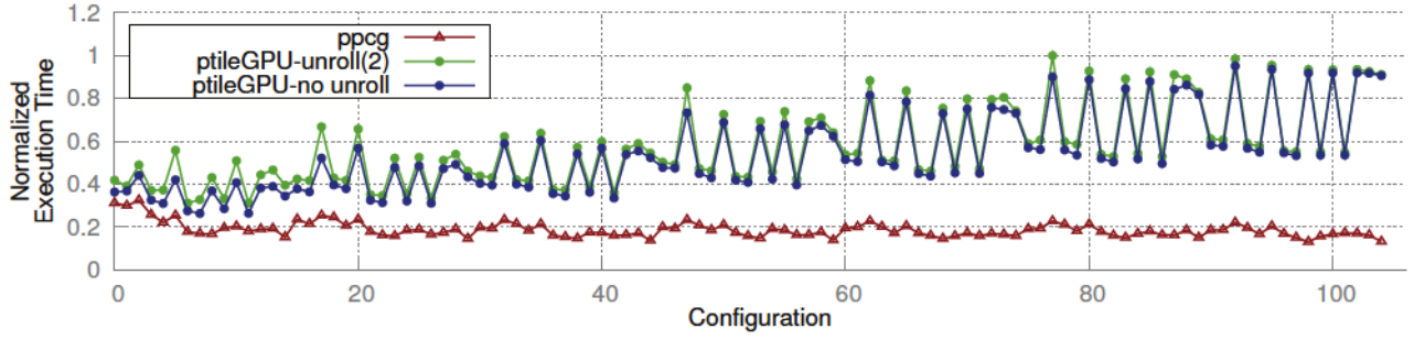
(f) With local memory and unrolling optimization. Worst execution time 0.558sec.
