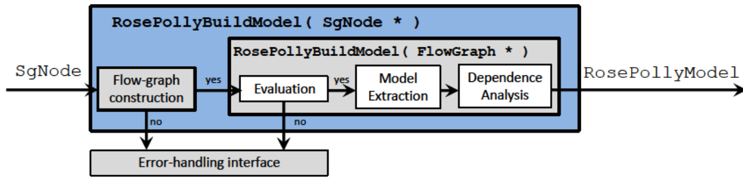
Figure 5.3: The structure of the RosePolly model-extraction function.
