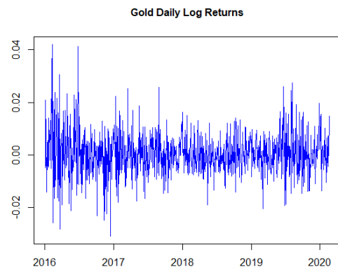
Figure 7.5: Gold log-returns
