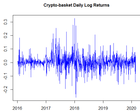
Figure 7.4: Crypto-basket log-returns
