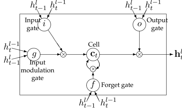
Fig. 14.3 A graphical representation of LSTM memory cells (there are minor differences in comparison to Graves [71]).
