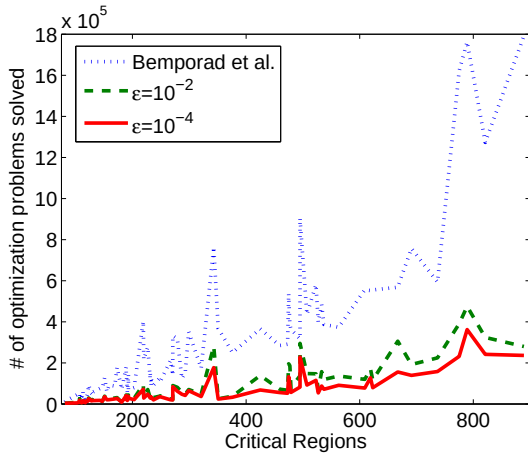
Fig. 3. Comparison of the number of optimization problems solved by the algorithm, that is, the sum of LP 1 , LP 2 and QP.
