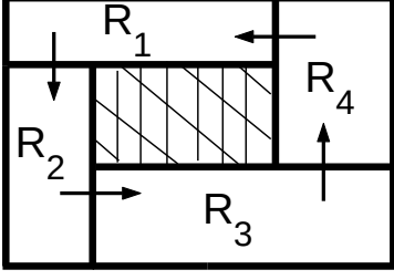
Fig. 1. Illustration that Algorithm 1 may fail to identify all the critical regions if the facet-to-facet property does not hold, the strategies in Section 3.1 or 3.2 are employed at step 7 of Algorithm 1 and no additional assumptions on the problem are given. The shaded region is unexplored.
