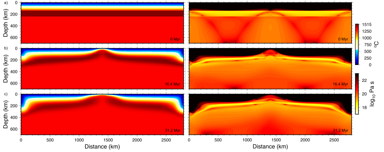
Figure S9: A comparison of the model at different timesteps in terms of evolving temperature and viscosity. There is a 200^{\circ}\text{C} hot layer, with a lithosphere thickness of 140 km and spreading rate of 12\text{ mm yr}^{-1} . (a) Represents the model at 0 Myr, similar to Fig. 5. (b) Represents the model at 16.4 Myr, during the syn-rift stage and approximately matching peak melt thickness, and (c) represents the model at 31.2 Myr, in the post-rift phase. In parts (b) and (c) the zone of partial melting is observed at the centre top of the model. The reflective boundaries can be seen in (b) and (c), and are considered far enough not to affect melt thickness production.
