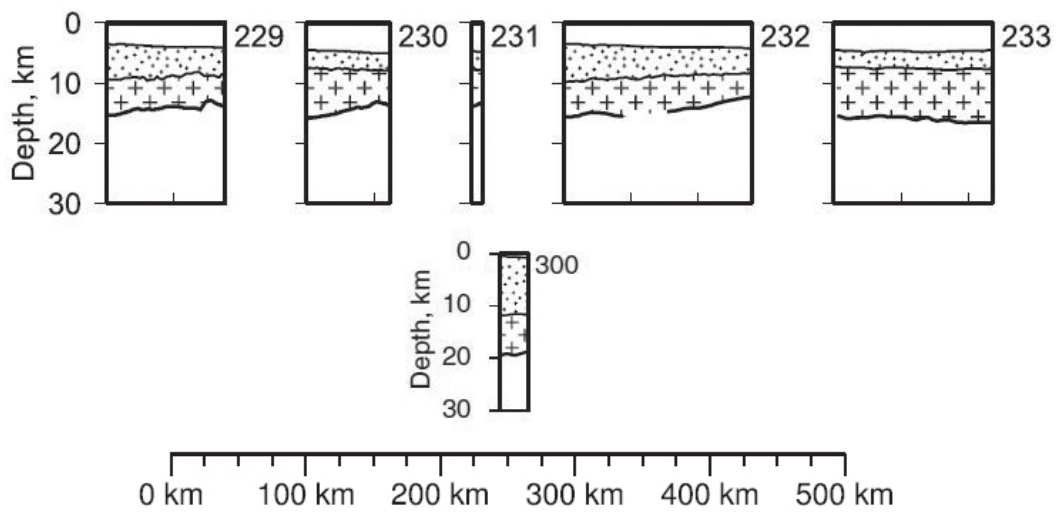
Figure S7: Crustal thickness measurement at the LaLOC locations for Winterbourne et al. (2014) data. Ocean crust depicted by '+', and sediment by dots.
