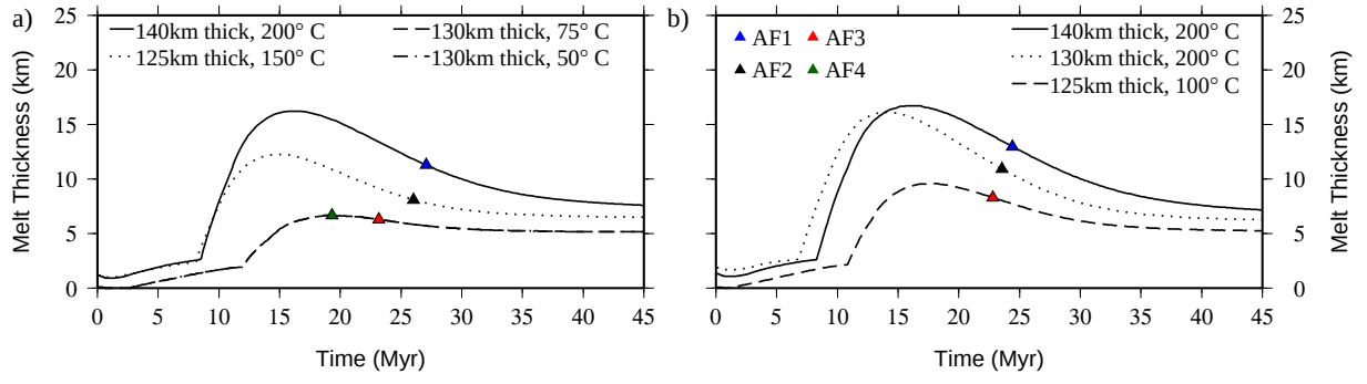
Figure S11: Models run with asthenosphere temperature of 1315^{\circ}\text{C} and spreading rate of 12\text{ mm yr}^{-1} for maximum and minimum ranges of the African wide-angle profiles. Panel (a) uses the minimum error range of initial ocean crustal thicknesses, however this results in the same hot layer temperature matches as in Fig. 12a. Panel (b) uses the maximum error range of initial ocean crustal thickness. AF4 is not included here due to its larger error range. Although hotter layers are required for AF2 and AF3, we still see a decrease in temperature along-strike.
