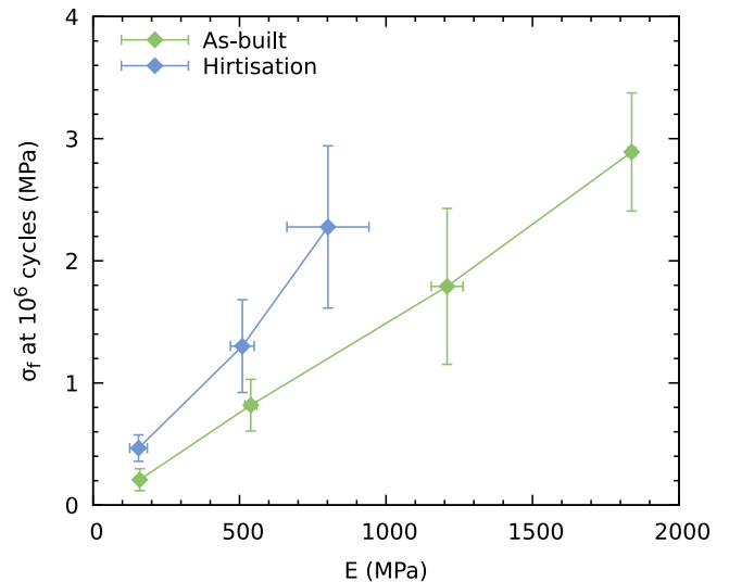
Fig. 10. Ashby plot showing the high cycle ( 10^6 cycles) fatigue strength vs. modulus E for the as-built condition and after hirtisation - a crucial comparison for maximising the fatigue resistance of stiffness-matched medical implant materials.
