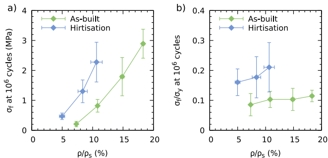
Fig. 9. Ashby plots showing (a) the high cycle ( 10^6 cycles) fatigue strength vs. \rho/\rho_s , and (b) high cycle fatigue strength normalised to \sigma_y vs. \rho/\rho_s , for both the as-built condition and after hirtisation.
