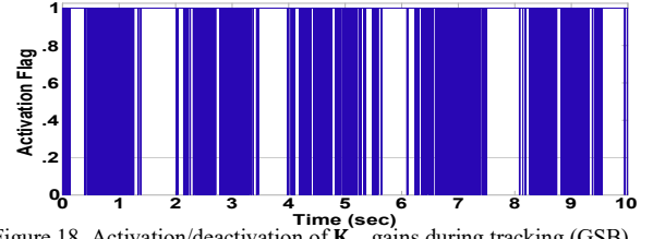
Figure 18. Activation/deactivation of K_{p_i} gains during tracking (GSB).
