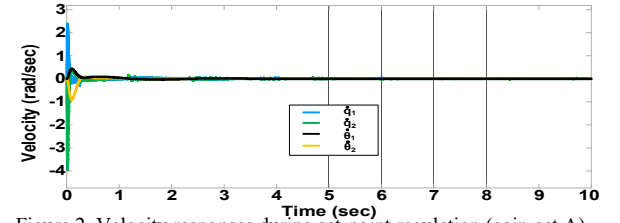
Figure 2. Velocity responses during set-point regulation (gain-set A).
