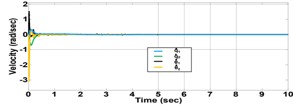
Figure 7. Velocity responses during set-point regulation (GSB).
