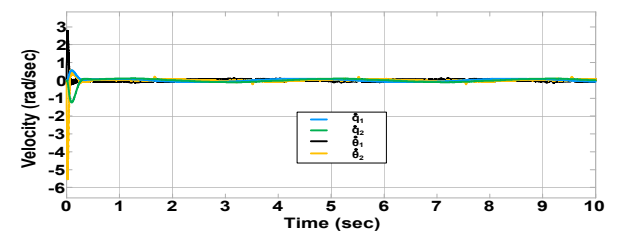
Figure 12. Velocity responses during trajectory tracking (GSA).
