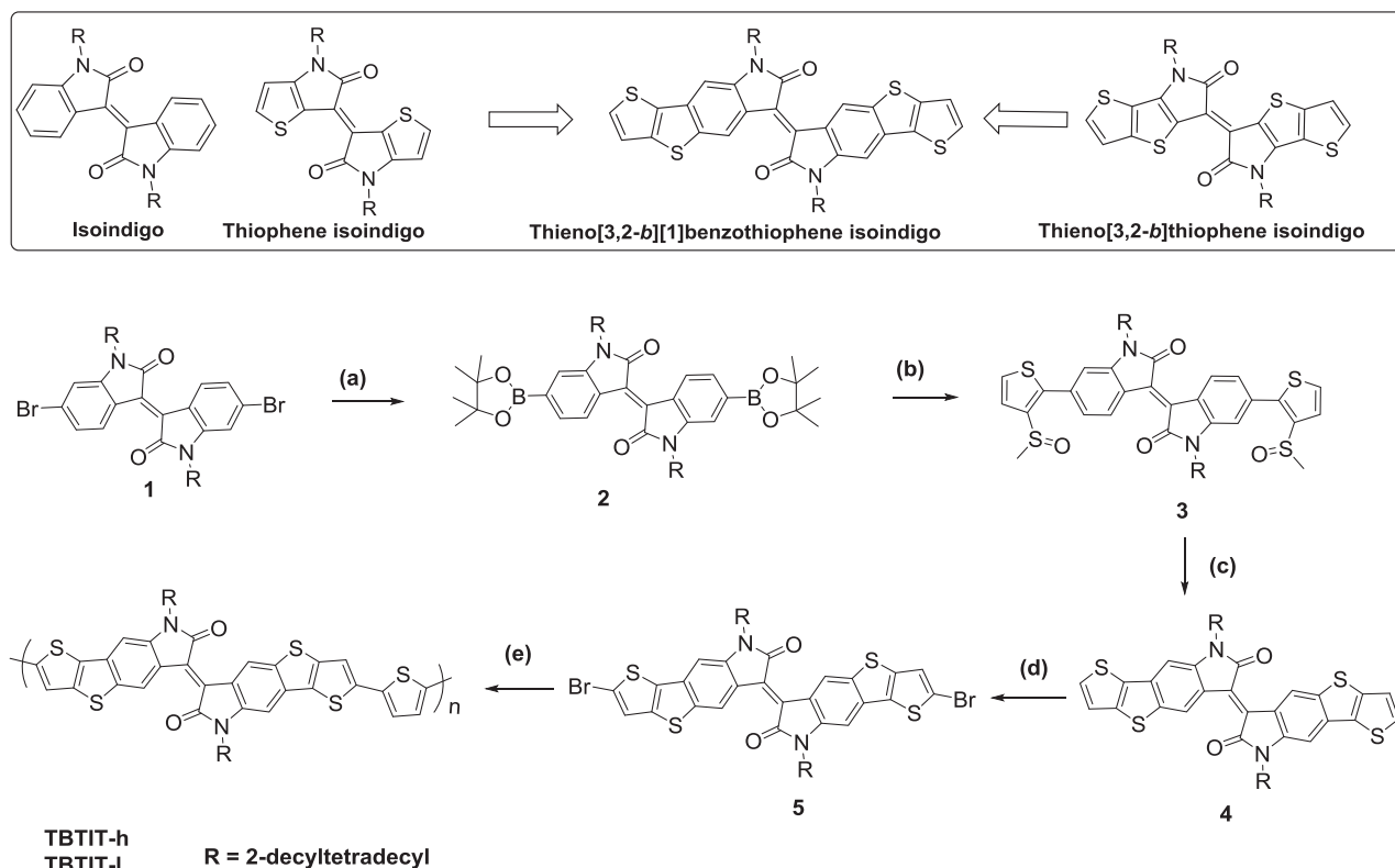
Figure 1. Structures of isoidindigo derivatives and synthesis route of monomer and polymer. a) Bis(pinacolato)diboron, \text{Pd}(\text{PPh}_3)_2\text{Cl}_2 , AcOK, anhydrous toluene, reflux, 16 h; b) bromo-3-methylsulfinylthiophene, \text{Pd}_2(\text{dba})_3 , \text{P}(\text{o-tol})_3 , aq. \text{K}_3\text{PO}_4 , toluene, reflux, 18 h; c) Eaton's reagent, rt, 3 d, then pyridine, reflux, overnight; d) NBS, \text{CHCl}_3/\text{AcOH} , reflux, 5 h; e) bis(trimethylstannyl)thiophene, \text{Pd}_2(\text{dba})_3 , \text{P}(\text{o-tol})_3 , chlorobenzene, \mu\text{W} .
