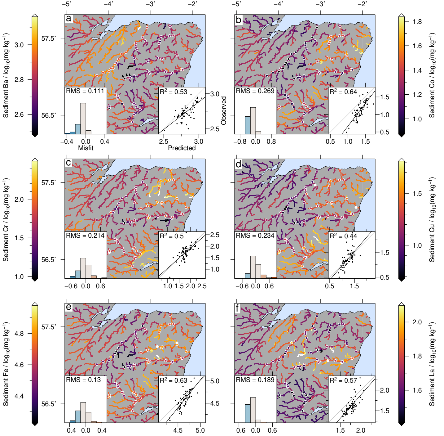
Figure 6. Comparison of observations and predictions for elements modelled by our approach. (a) Observed Barium concentrations (coloured circles) overlain on predictions (coloured curves). Note logarithmic colour scale. Right inset shows cross plot of observations and predictions; grey line is 1:1 relationship; black line is linear fit to points; annotation shows R^2 value. Left inset shows histogram of misfit between observations and predictions; bin width is equal to RMS misfit; blue/red indicate over-/under-prediction. (b) Cobalt. (c) Chromium. (d) Copper. (e) Iron. (f) Lanthanum. Results for all other elements are shown in Figures 4, 5, 8 and 7.
