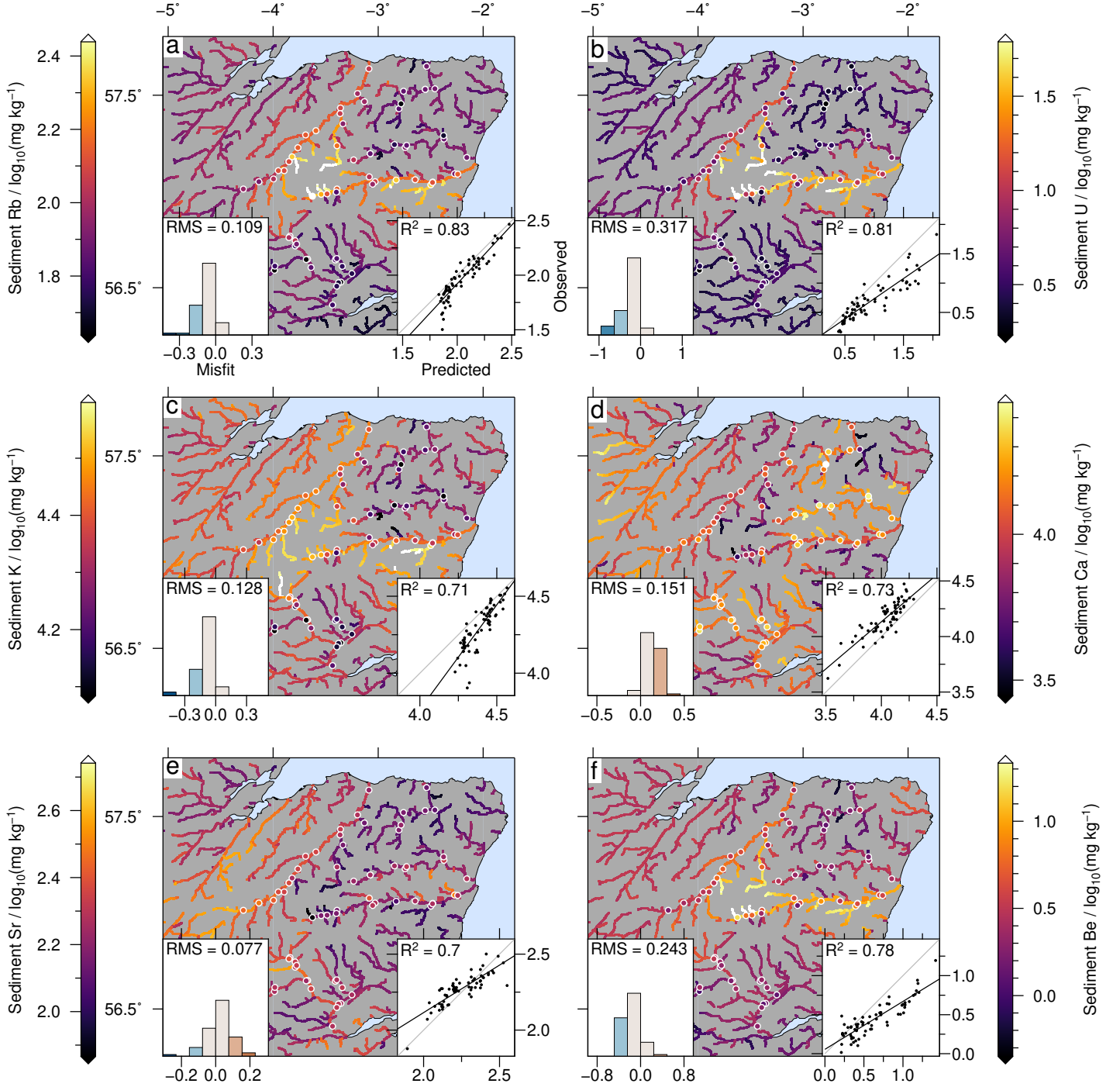
Figure 5. Comparison of observations and most accurate predictions. (a) Observed Rubidium concentrations (coloured circles) overlain on model predictions (coloured curves). Note logarithmic colour scale. Right inset shows cross plot of observations and predictions; grey line is 1:1 relationship; black line is linear fit to points; annotation shows R^2 value. Left inset is histogram of misfits; bin width is equal to RMS misfit; blue/red indicate over-/under-prediction. (b) Uranium. (c) Potassium. (d) Calcium. (e) Strontium. (f) Beryllium. Results for elements with less accurate predictions are shown in Figure 8. Results for all other elements are shown in Figures 4, 6 and 7.
