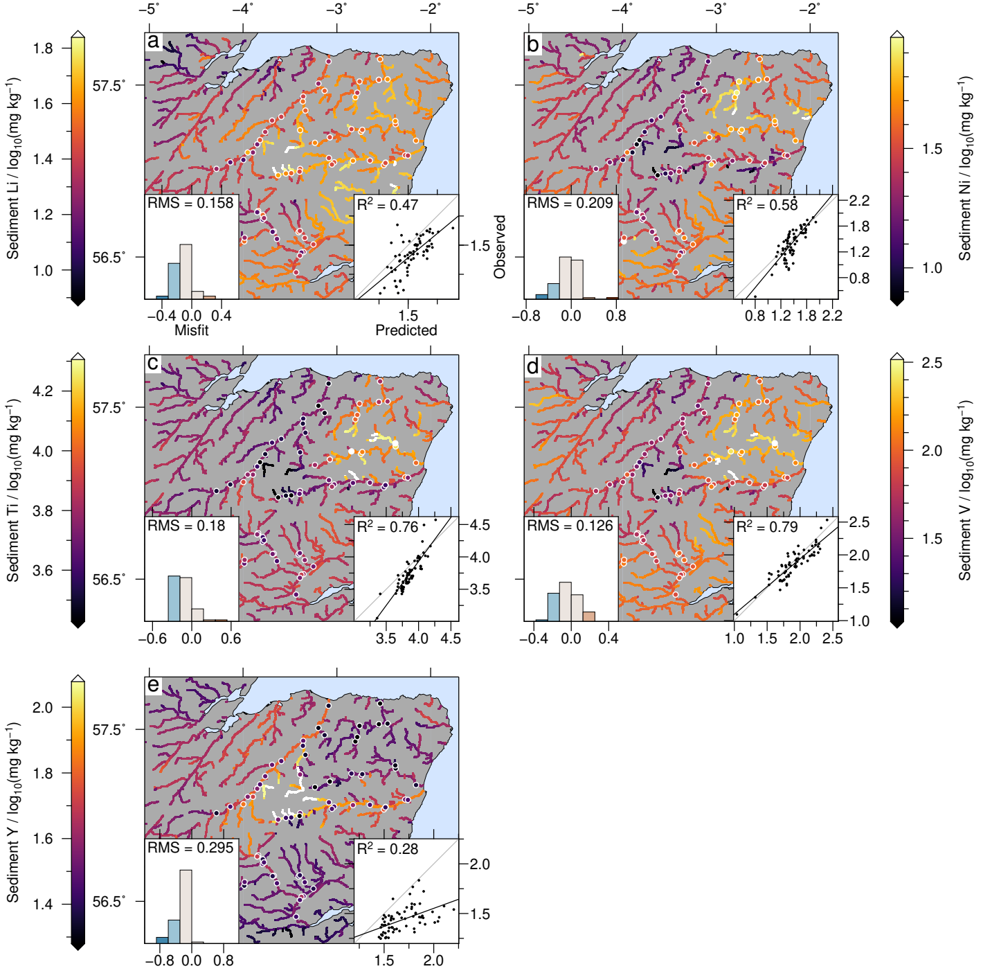
Figure 7. Comparison of observations and predictions for elements modelled by our approach. (a) Observed Lithium concentrations (coloured circles) overlain on predictions (coloured curves). Note logarithmic colour scale. Right inset shows cross plot of observations and predictions; grey line is 1:1 relationship; black line is linear fit to points; annotation shows R^2 value. Left inset shows histogram of misfit between observations and predictions; bin width is equal to RMS misfit; blue/red indicate over-/under-prediction. (b) Nickel. (c) Titanium. (d) Vanadium. (e) Yttrium. Results for other elements modelled by our approach. Results for all other elements are shown in Figures 4, 5, 8 and 6.
