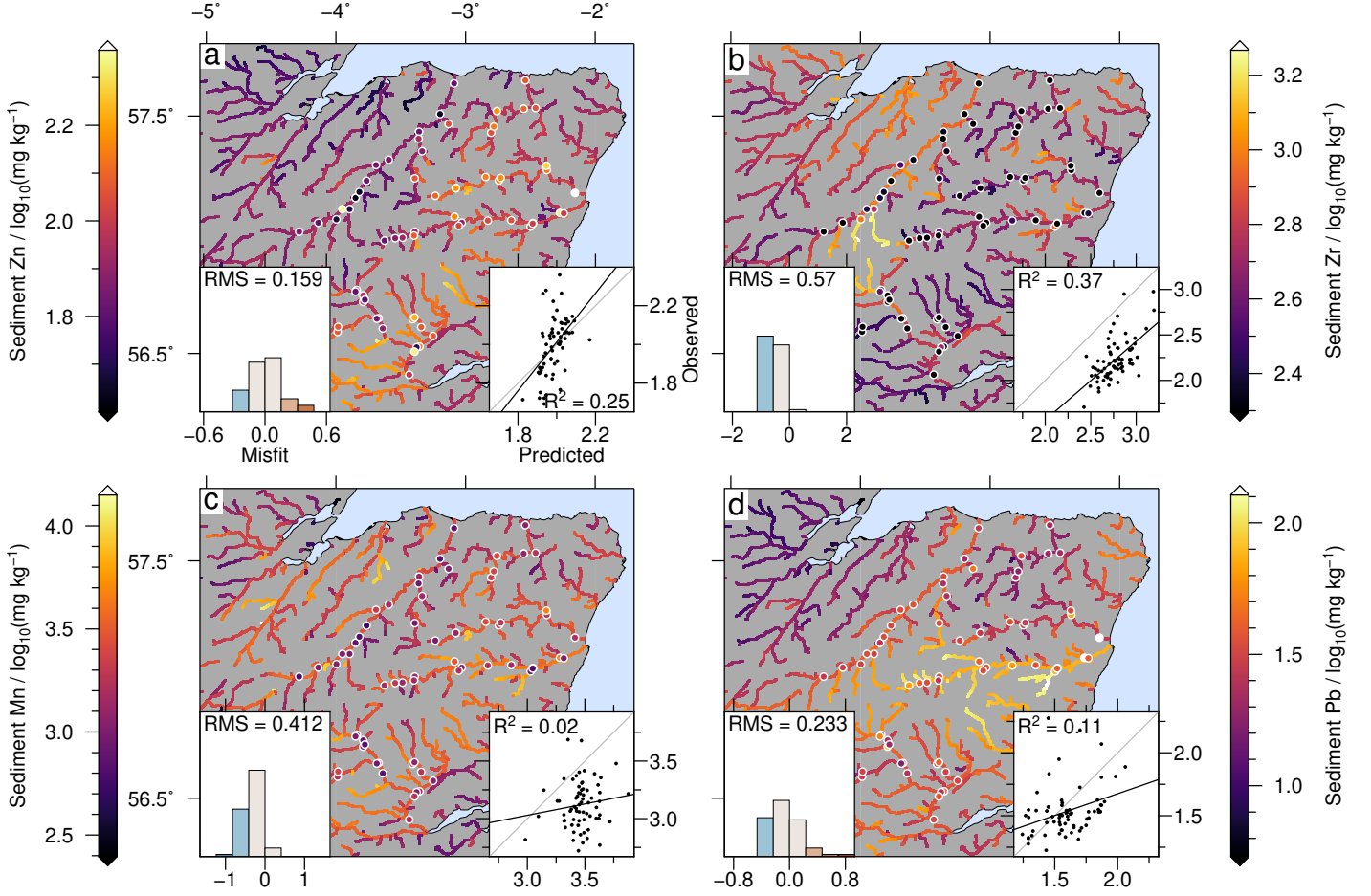
Figure 8. Comparison of observations and least accurate predictions. (a) Observed Zinc concentrations (coloured circles) overlain on predictions (coloured curves). Note logarithmic colour scale. Right inset shows cross plot of observations and predictions; grey line is 1:1 relationship; black line is linear fit to points; annotation shows R^2 value. Left inset shows histogram of misfit between observations and predictions; bin width is equal to RMS misfit; blue/red indicate over-/under-prediction. (b) Zirconium. (c) Manganese. (d) Lead. Results for elements with more accurately predicted concentrations are shown in Figure 5. Results for all other elements are shown in Figures 4, 6 and 7.
