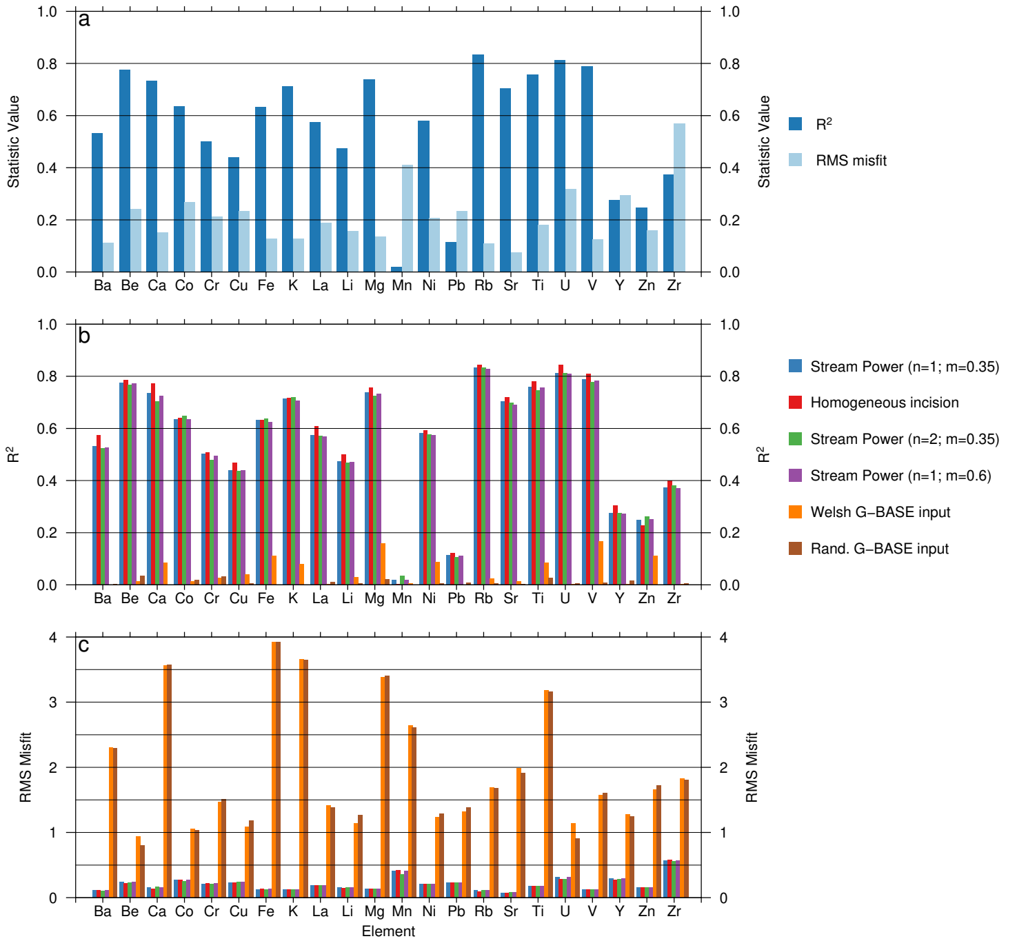
Figure 9. Evaluation of model predictions. (a) R^2 and RMS misfit between observed and predicted element concentrations for preferred Stream Power erosional model ( n = 1; m = 0.35 ). (b) R^2 for different models and parameterisations; see key and Supporting Information for visualisation of substrate generated using Welsh G-BASE measurements and a random distribution (Figure S1). (c) RMS misfit for different models/parameterisations.
