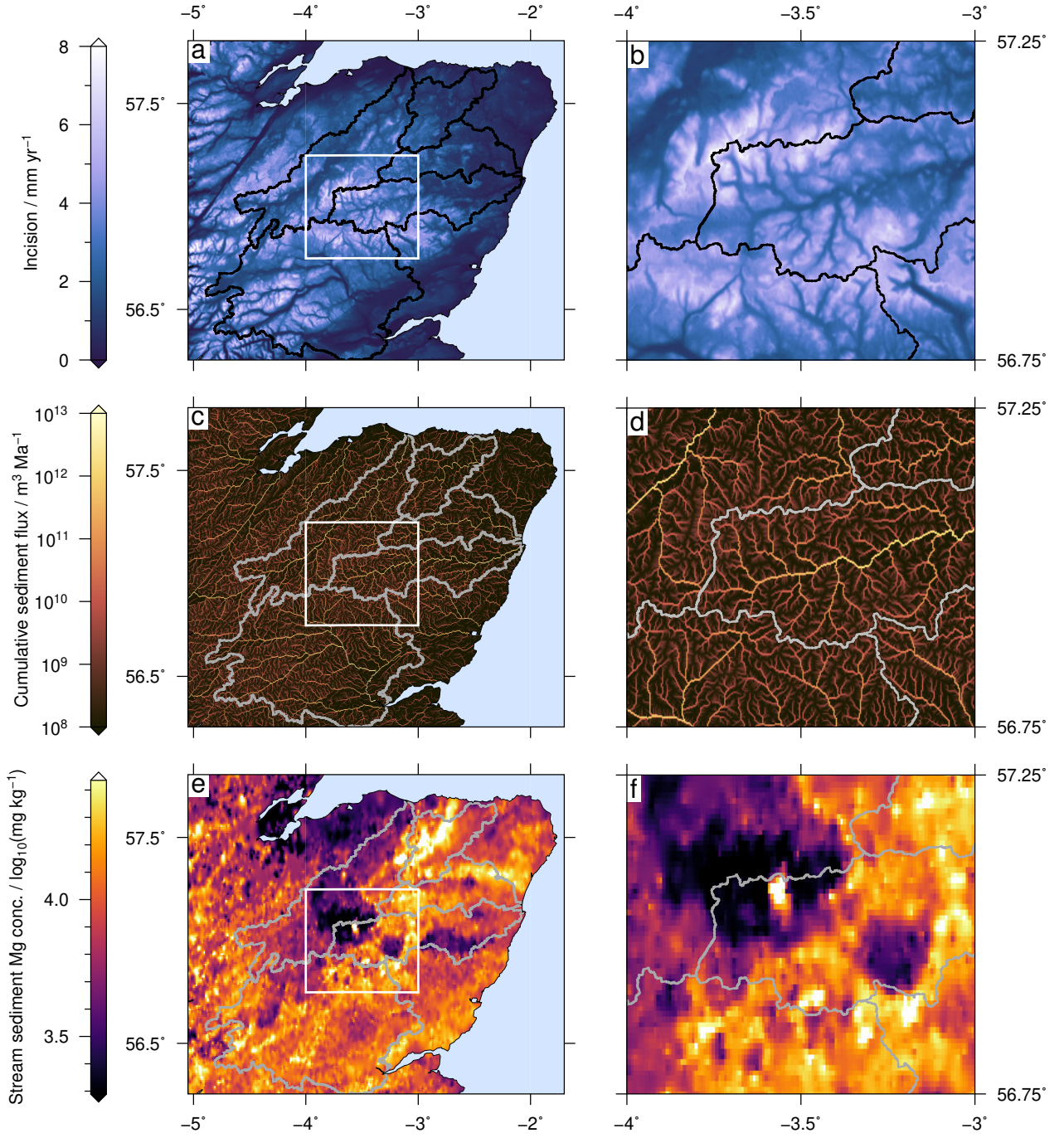
Figure 3. Inputs used in geochemical predictions. (a) Predicted incision, \partial z/\partial t , calculated using SRTM data set (Figure 1a) and Equation 3 with n = 1 , m = 0.35 , v = 3.62 \text{ m}^{0.3} \text{ Ma}^{-1} . Note that the white box = panel (b), which shows upper portion of Dee catchment. Grey lines indicate catchment boundaries. (c-d) Predicted cumulative sediment flux calculated by integrating incision (panel a) along flow paths. (e-f) Mg composition of first-order stream sediments interpolated from G-BASE localities using a continuous curvature spline with a tension factor of 0.25 (Figure 1c). Analogous maps were generated for all elements.
