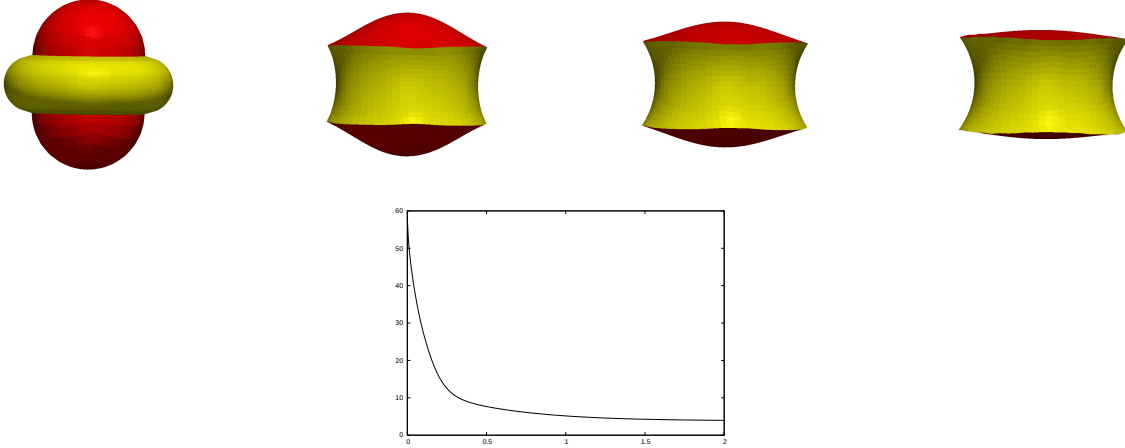
FIGURE 7.1. ( C^0 : \bar{\kappa}_1 = \bar{\kappa}_2 = 0 , \varsigma = 0.1 ) A plot of (\Gamma_i^m)_{i=1}^2 at times t = 0, 0.5, 1, 2 . Below a plot of the discrete energy E^{m+1}((\Gamma^m)_{i=1}^2) .
