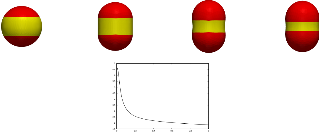
FIGURE 7.16. ( C^1 : \bar{\kappa}_1 = -2 , \bar{\kappa}_2 = -0.5 , \varsigma = 0.1 , \varrho = 2 , \theta = 0.05 ) Volume preserving flow. A plot of (\Gamma_i^m)_{i=1}^2 at times t = 0, 0.1, 0.5, 1 . Below a plot of the discrete energy E^{m+1}((\Gamma^m)_{i=1}^2) .
