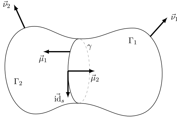
FIGURE 2.1. Sketch of \Gamma = \Gamma_1 \cup \gamma \cup \Gamma_2 with outer unit normals \vec{\nu}_i , conormals \vec{\mu}_i and tangent vector \vec{\text{id}}_s on \gamma for the case d = 3 .
