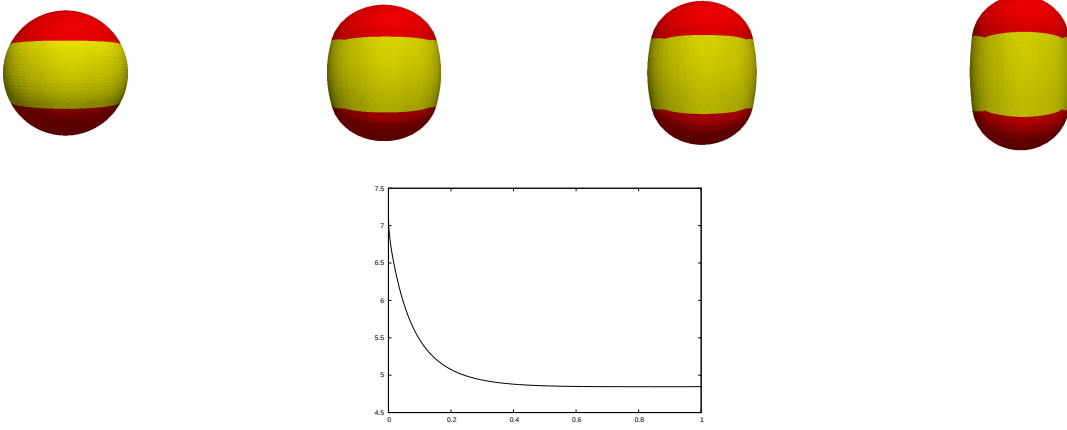
FIGURE 7.15. ( C^1 : \bar{\kappa}_1 = -2 , \bar{\kappa}_2 = -0.5 , \varsigma = 0.1 , \varrho = 2 ) Surface area preserving flow. A plot of (\Gamma_i^m)_{i=1}^2 at times t = 0, 0.1, 0.2, 1 . Below a plot of the discrete energy E^{m+1}((\Gamma^m)_{i=1}^2) .
