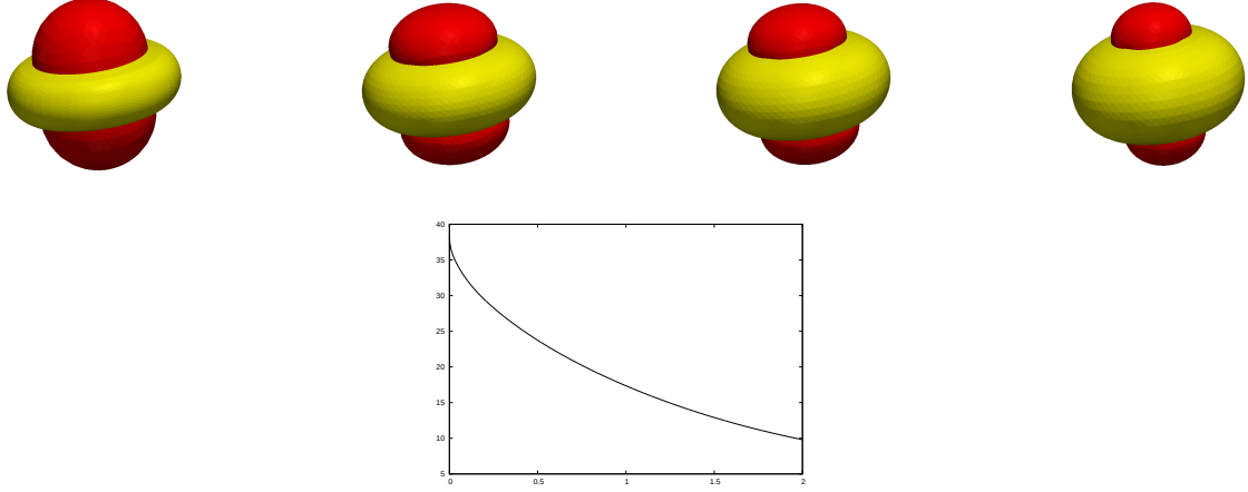
FIGURE 7.5. ( C^0 : \bar{\kappa}_1 = -2 , \bar{\kappa}_2 = -0.5 , \varsigma = 0.1 , \varrho = 2 ) Volume preserving flow. A plot of (\Gamma_i^m)_{i=1}^2 at times t = 0, 0.5, 1, 2 . Below a plot of the discrete energy E^{m+1}((\Gamma^m)_{i=1}^2) .
