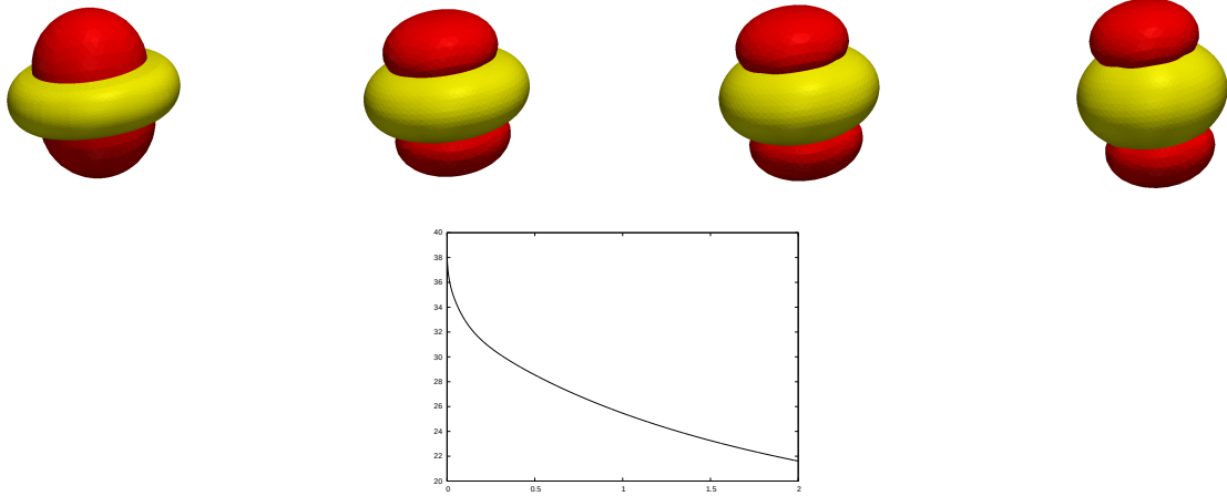
FIGURE 7.4. ( C^0 : \bar{\kappa}_1 = -2 , \bar{\kappa}_2 = -0.5 , \varsigma = 0.1 , \varrho = 2 ) Surface area preserving flow. A plot of (\Gamma_i^m)_{i=1}^2 at times t = 0, 0.5, 1, 2 . Below a plot of the discrete energy E^{m+1}((\Gamma^m)_{i=1}^2) .
