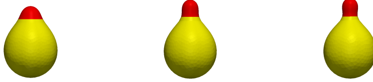
FIGURE 7.21. ( C^1 : \bar{\kappa}_1 = \bar{\kappa}_2 = 0 , \varsigma = 9 , \varrho = 4 ) A plot of (\Gamma_i^m)_{i=1}^2 at time t = 0.25 for the reduced volumes v_r = 0.95, 0.91 and 0.9 , respectively.
