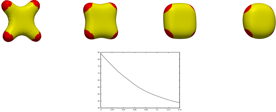
FIGURE 7.17. ( C^1 : \bar{\kappa}_1 = \bar{\kappa}_2 = 0 , \varsigma = 1 ) A plot of (\Gamma_i^m)_{i=1}^2 at times t = 0, 0.05, 0.1, 0.14 . Below a plot of the discrete energy E^{m+1}((\Gamma_i^m)_{i=1}^2) .
