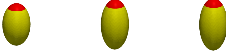
FIGURE 7.20. The initial shapes for v_r = 0.95, 0.91 and 0.9 , respectively.
