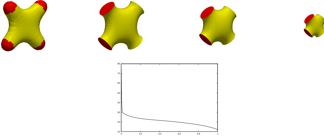
FIGURE 7.6. ( C^0 : \bar{\kappa}_1 = \bar{\kappa}_2 = 0 , \varsigma = 1 ) A plot of (\Gamma_i^m)_{i=1}^2 at times t = 0, 0.1, 0.5, 1 . Below a plot of the discrete energy E^{m+1}((\Gamma^m)_{i=1}^2) .
