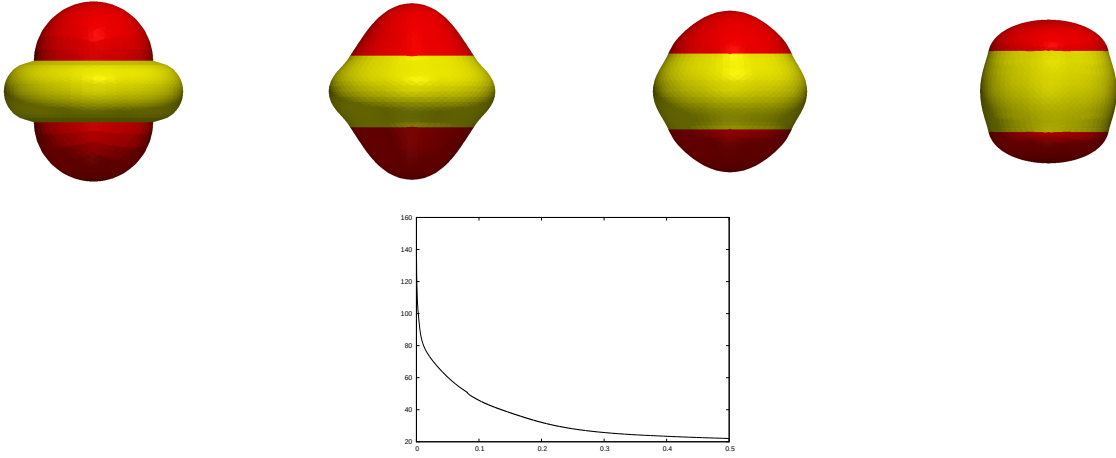
FIGURE 7.13. ( C^1 : \bar{\kappa}_1 = -2 , \bar{\kappa}_2 = -0.5 , \varsigma = 0.1 , \varrho = 2 ) A plot of (\Gamma_i^m)_{i=1}^2 at times t = 0, 0.1, 0.2, 0.5 . Below a plot of the discrete energy E^{m+1}((\Gamma^m)_{i=1}^2) .
