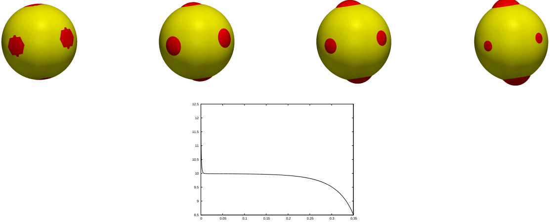
FIGURE 7.7. ( C^0 : \overline{\kappa}_1 = -4 , \overline{\kappa}_2 = -2 , \varsigma = 1 , \varrho = 2 ) Surface area preserving flow. A plot of (\Gamma_i^m)_{i=1}^2 at times t = 0, 0.1, 0.3, 0.35 . Below a plot of the discrete energy E^{m+1}((\Gamma^m)_{i=1}^2) .
