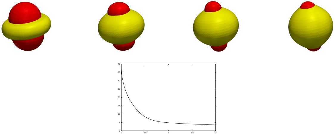
FIGURE 7.2. ( C^0 : \bar{\kappa}_1 = -2 , \bar{\kappa}_2 = -0.5 , \varsigma = 0.1 ) A plot of (\Gamma_i^m)_{i=1}^2 at times t = 0, 0.5, 1, 2 . Below a plot of the discrete energy E^{m+1}((\Gamma^m)_{i=1}^2) .
