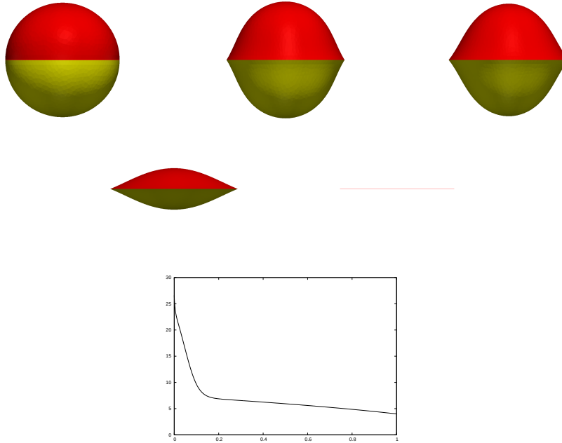
FIGURE 7.10. ( C^0 : \bar{\kappa}_1 = \bar{\kappa}_2 = 0 , \varsigma = 1 , \varrho = 2 ) A plot of (\Gamma_i^m)_{i=1}^2 at times t = 0, 0.01, 0.02, 0.1, 1 . At time t = 1 the evolution has reached a disk. Below a plot of the discrete energy E^{m+1}((\Gamma^m)_{i=1}^2) .
