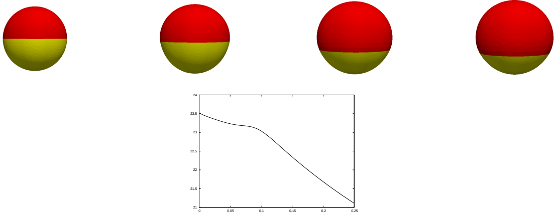
FIGURE 7.18. ( C^1 : \bar{\kappa}_1 = \bar{\kappa}_2 = -0.5 , \varsigma = 0 , \alpha_1^G = 0.5 , \alpha_2^G = 1 ) A plot of (\Gamma_i^m)_{i=1}^2 at times t = 0, 0.1, 0.2, 0.25 . Below a plot of the discrete energy E^{m+1}((\Gamma_i^m)_{i=1}^2) .
