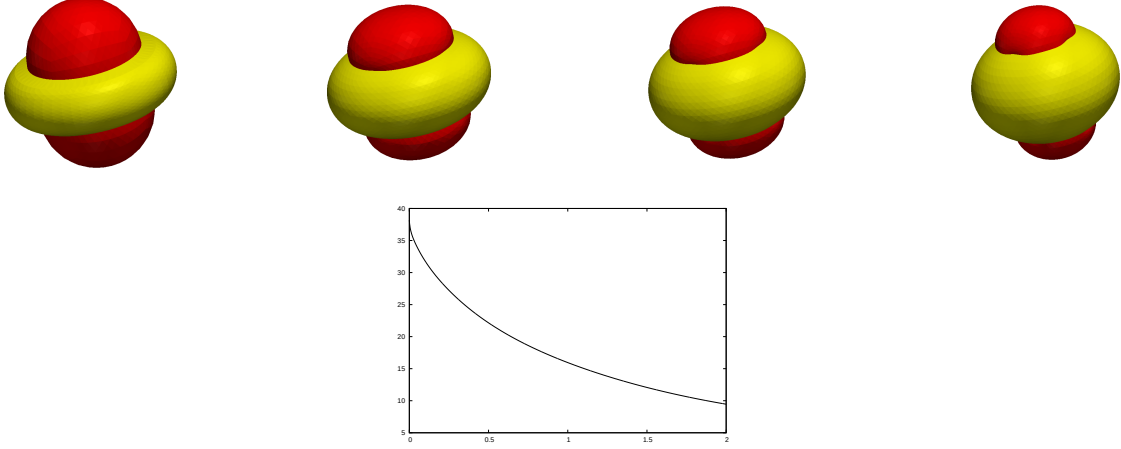
FIGURE 7.3. ( C^0 : \bar{\kappa}_1 = -2 , \bar{\kappa}_2 = -0.5 , \varsigma = 0.1 , \varrho = 2 ) A plot of (\Gamma_i^m)_{i=1}^2 at times t = 0, 0.5, 1, 2 . Below a plot of the discrete energy E^{m+1}((\Gamma^m)_{i=1}^2) .
