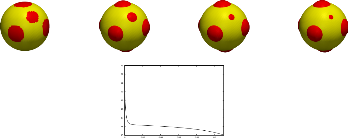
FIGURE 7.8. ( C^0 : \overline{\kappa}_1 = -4 , \overline{\kappa}_2 = -2 , \varsigma = 1 , \varrho = 2 ) Surface area preserving flow. A plot of (\Gamma_i^m)_{i=1}^2 at times t = 0, 0.05, 0.1, 0.11 . Below a plot of the discrete energy E^{m+1}((\Gamma^m)_{i=1}^2) .
