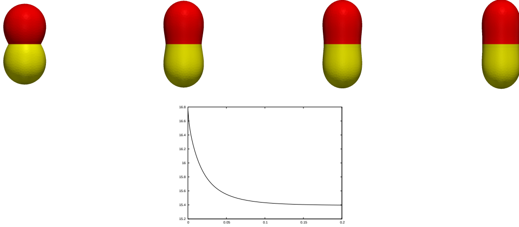
FIGURE 7.9. ( C^0 : \bar{\kappa}_1 = \bar{\kappa}_2 = -1 , \varsigma = 1 , \varrho = 2 ) Volume and surface area preserving flow. A plot of (\Gamma_i^m)_{i=1}^2 at times t = 0, 0.05, 0.1, 0.2 . Below a plot of the discrete energy E^{m+1}((\Gamma^m)_{i=1}^2) .
