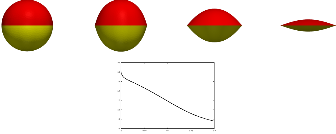
FIGURE 7.11. ( C^0 : \bar{\kappa}_1 = \bar{\kappa}_2 = 0 , \varsigma = 1 , \alpha_1^G = \alpha_2^G = -1 , \varrho = 2 ) A plot of (\Gamma_i^m)_{i=1}^2 at times t = 0, 0.01, 0.1, 0.2 . Below a plot of the discrete energy E^{m+1}((\Gamma^m)_{i=1}^2) .
