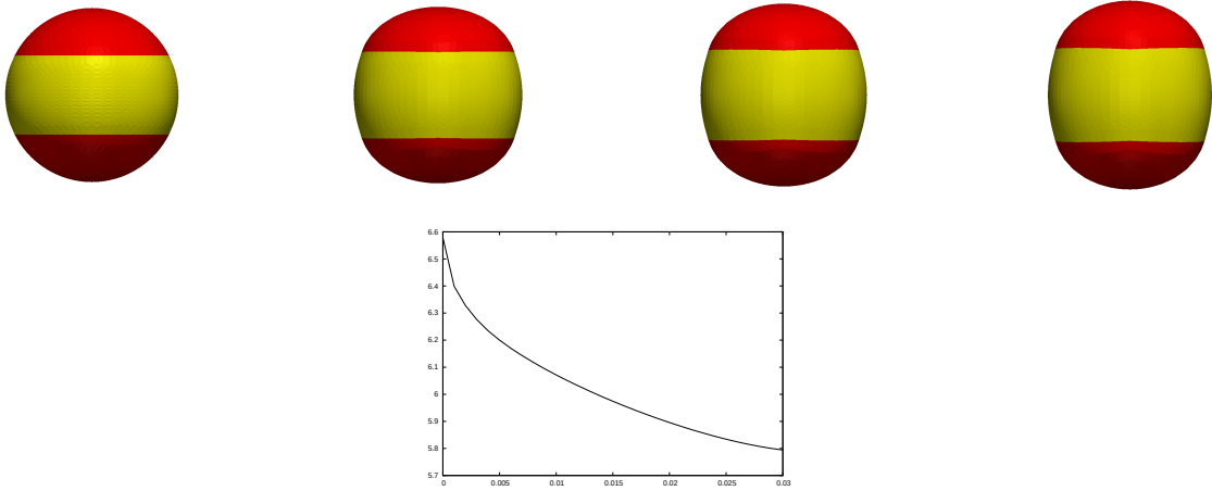
FIGURE 7.14. ( C^1 : \bar{\kappa}_1 = -2 , \bar{\kappa}_2 = -0.5 , \varsigma = 0.1 ) A plot of (\Gamma_i^m)_{i=1}^2 at times t = 0, 0.01, 0.02, 0.03 . Below a plot of the discrete energy E^{m+1}((\Gamma^m)_{i=1}^2) .
