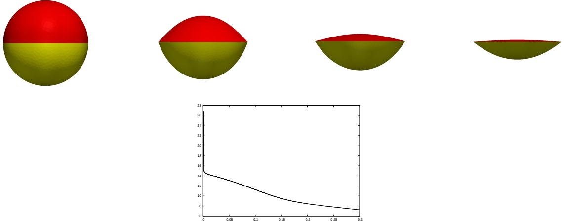
FIGURE 7.12. ( C^0 : \bar{\kappa}_1 = \bar{\kappa}_2 = 0 , \varsigma = 1 , \alpha_1^G = -1 , \alpha_2^G = -1.5 , \varrho = 2 ) A plot of (\Gamma_i^m)_{i=1}^2 at times t = 0, 0.1, 0.2, 0.3 . Below a plot of the discrete energy E^{m+1}((\Gamma^m)_{i=1}^2) .
