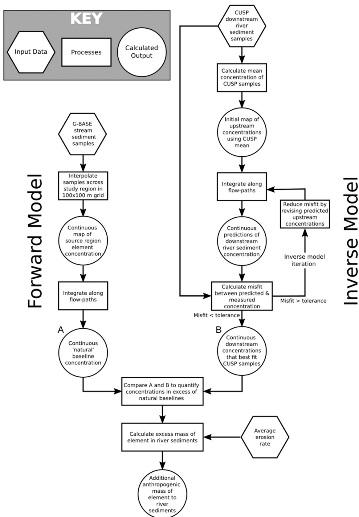
Fig. 2. Modelling strategy. The forward model generates continuous estimates of chemical baselines along rivers by mixing source region concentrations from the G-BASE downstream. The inverse model inverts element concentrations measured at specific sites along the Clyde river for source region concentrations, which includes natural and anthropogenic material. Finally, the differences between concentrations calculated from natural (e.g., geologic) sources (forward modelling of G-BASE samples) and measurements along the river (inverse modelling of CUSP samples) are used to calculate excess (anthropogenic) element concentrations and masses along the rivers.
