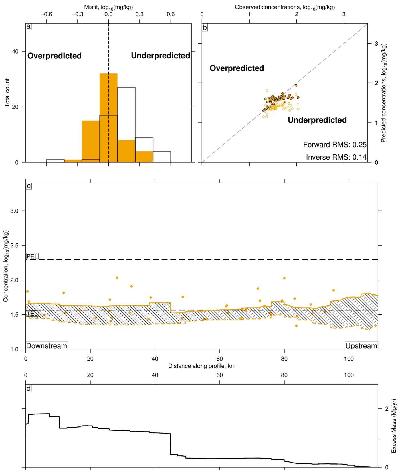
Fig. 8. Comparing baseline (forward model) predictions of Cu concentrations to predictions from best-fitting inverse model. (a–d) See Fig. 7 for explanation. Total calculated excess mass: 1500 kg/yr.
