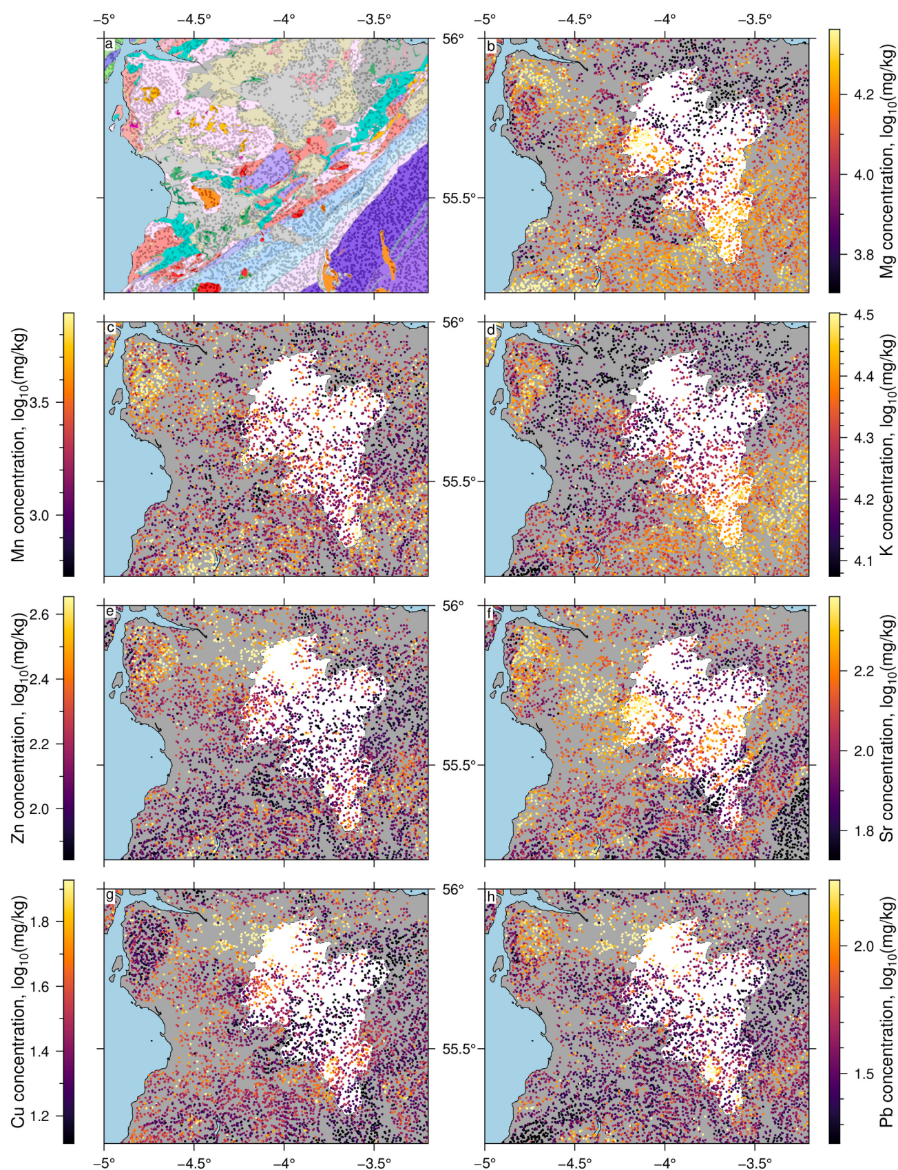
Fig. 3. Source region elemental concentrations. (a) Geologic map and G-BASE sample localities in first-order streams (grey circles; see Fig. 1). (b) Concentrations of Mg in G-BASE samples (coloured circles). White polygon = upper Clyde catchment. (c) Mn. (d) K. (e) Zn. (f) Sr. (g) Cu. (h) Pb.
