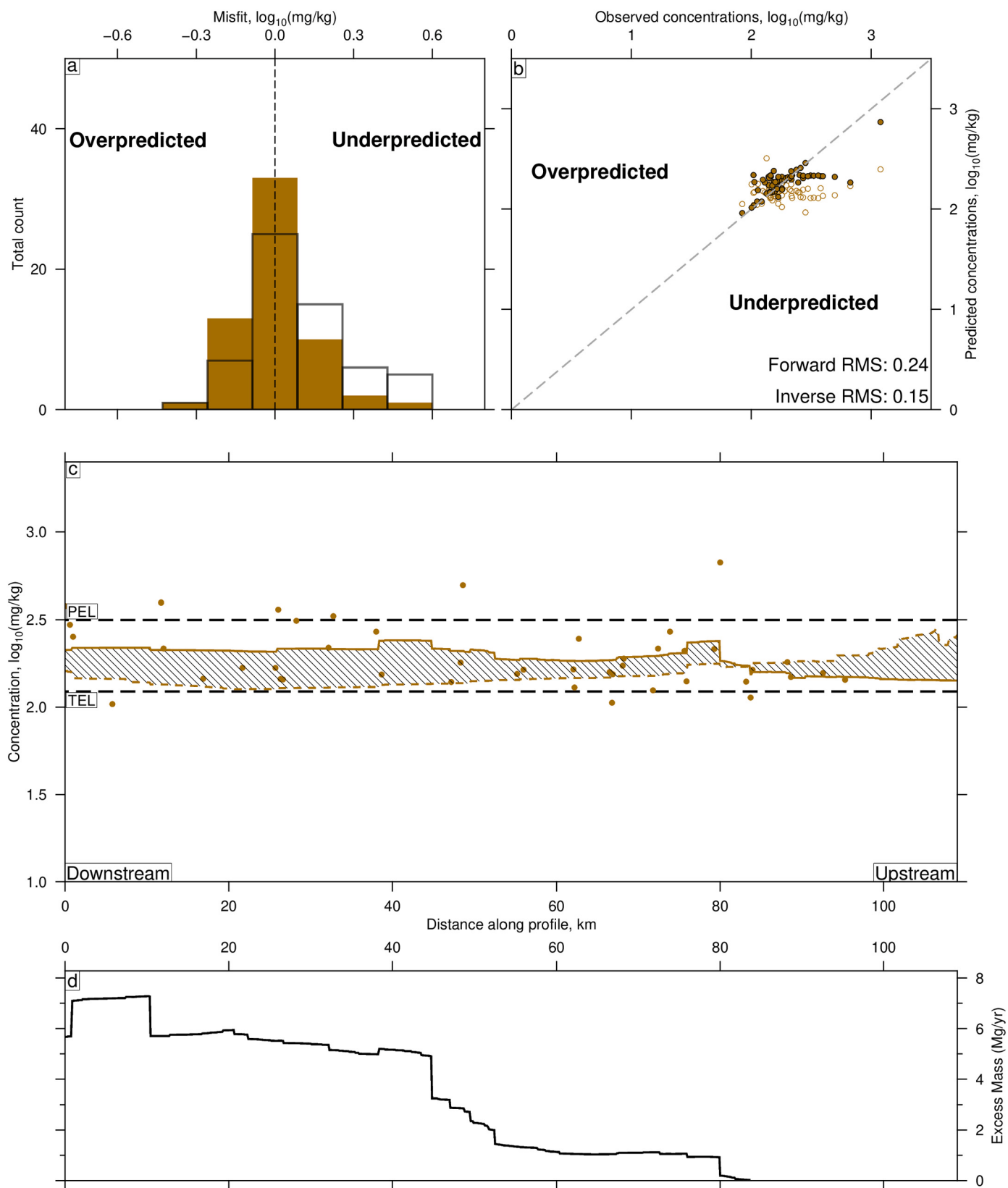
Fig. 9. Comparing baseline (forward model) predictions of Zn concentrations to predictions from best-fitting inverse model. (a–d) See Fig. 7 for explanation. Total calculated excess mass: 5700 kg/yr.
