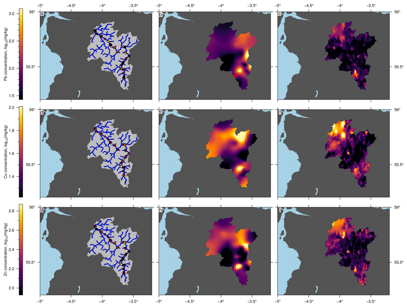
Fig. 6. Inverse modelling: source region heavy metal concentrations. (a, d, g) Coloured circles = Observed concentrations in CUSP samples inverted for upstream (source region) concentrations; light grey polygon/blue lines = drainage basin/network. (b, e, h) Predicted source region concentrations from best-fitting inverse model. (c, f, i) Observed 'geologic' source region concentrations interpolated from G-BASE measurements of first-order stream compositions (see Fig. 3). (a–c) Pb. (d–f) Cu. (g–i) Zn. (For interpretation of the references to colour in this figure legend, the reader is referred to the web version of this article.)
