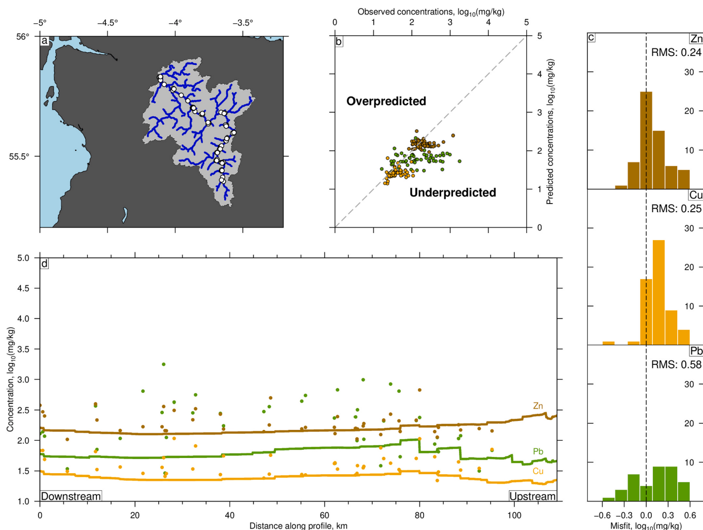
Fig. 5. Forward modelling: calculated baselines for select heavy metals. (a) Blue = upper Clyde drainage network; white circles = CUSP samples. (b) Observed vs. predicted concentrations for Zn (brown), Pb (green), Cu (yellow). Dashed line = 1:1 relationship. (c) Misfit (difference) between observations and predictions. Bin size = 0.15\log_{10}(\text{mg/kg}) . Note annotated root-mean-square misfit (RMS); and tendency for under-prediction. (d) Circles = observed concentrations; solid lines = predicted downstream composition along Clyde river. See Fig. 4 for extended caption. (For interpretation of the references to colour in this figure legend, the reader is referred to the web version of this article.)
