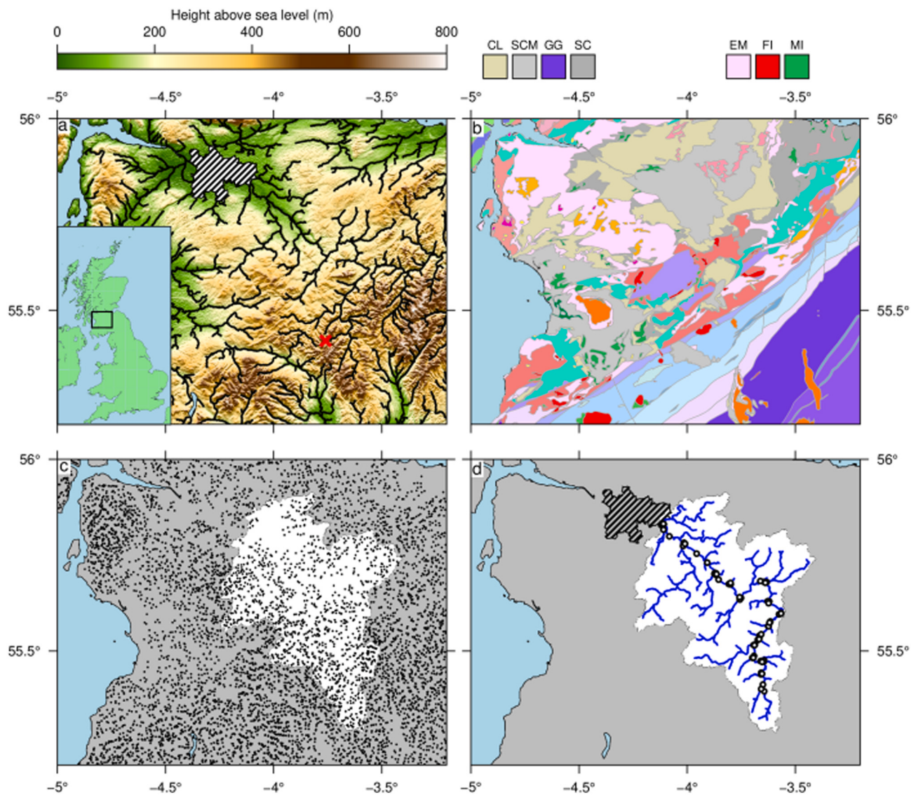
Fig. 1. Study area: Clyde basin, Scotland. (a) Topography (SRTM 1 arc sec) and extracted drainage network (Farr and Kobrick, 2000; De Jager and Vogt, 2010). Hashed polygon = Glasgow city area. Red cross = Lowther Hills Pb mining area. (b) Simplified geologic map. CL: Clackmannan Group (fluvial sandstones), SCM: Scottish Coal Measures (Mud/Silt/Sandstone), GG: Gala Group (Wackestone), SC: Strathclyde Group (estuarine sedimentary rock), EM: Extrusive Mafic lava/tuff, FI: Felsic Intrusions, MI: Mafic Intrusions. (c) Black circles = G-BASE geochemical samples of first-order stream sediments. White polygon = Upper Clyde drainage basin, the focus of this study. (d) White circles = geochemical samples along Clyde river collected as part of the Clyde Urban Super Project (CUSP). (For interpretation of the references to colour in this figure legend, the reader is referred to the web version of this article.)
