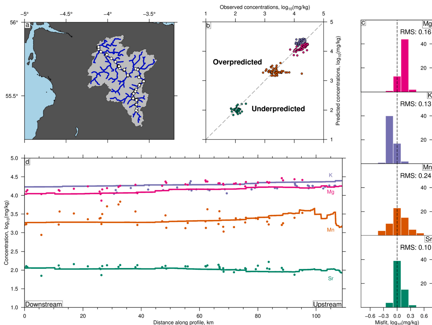
Fig. 4. Forward modelling: calculated baselines for select elements. (a) Blue = upper Clyde drainage network; white circles = locations of 60 CUSP samples used to test model predictions. (b) Observed (CUSP) vs. predicted concentrations at sample sites for Mg (pink), K (purple), Mn (orange), Sr (dark green); predictions were generated from forward model (solid lines in panel d; Eq. (2); see body text; Supplementary Fig. 7); dashed line = 1:1 relationship. (c) Difference, \log(D_i) - \log(F(C_i)) , between observations and predictions. Bin size = 0.15 \log_{10}(\text{mg/kg}) ; ordinates give absolute count ( N = 60 ); dashed line is centred on 0. Root Mean Square (RMS) misfit for each element is annotated. (d) Circles = observed concentrations of labelled elements (CUSP; white circles in panel a); solid lines = predicted elemental concentrations along Clyde river. (For interpretation of the references to colour in this figure legend, the reader is referred to the web version of this article.)
