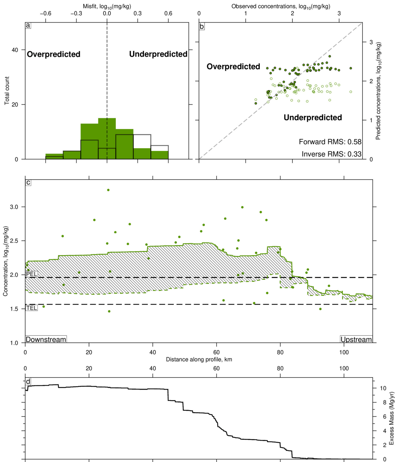
Fig. 7. Comparing baseline (forward model) predictions of Pb concentrations to predictions from best-fitting inverse model. (a) Misfit (difference) between observed and theoretical concentrations at the locations of the 60 CUSP samples (see Fig. 6a). Bin size = 0.15 \log_{10}(\text{mg/kg}) . Ordinate gives absolute count ( N = 60 ). Solid green = results from best-fitting inverse model (Fig. 6b). Black = results from forward model with source region parameterised using observed G-BASE first-order stream concentrations (Fig. 6c). (b) Observed (CUSP) vs. predicted concentrations at the locations of the CUSP samples; solid/open circles = results from best-fitting inverse model/forward model. RMS = root mean squared misfit between observations and predictions from forward and best-fitting inverse models. (c) Pb concentrations along the main river profile. Circles = observed concentrations (CUSP). Green dashed line = baseline predicted by forward modelling. Solid green line = predictions from best-fitting inverse model. Black dashed lines indicate threshold (TEL) and probable (PEL) effect levels (toxic elemental concentrations) for adverse effects on biological activity (Hudson-Edwards et al., 2008). (d) Calculated excess mass of Pb added to river per year; difference between predictions from best-fitting inverse and forward models. Total calculated excess mass: 9700 kg/yr. (For interpretation of the references to colour in this figure legend, the reader is referred to the web version of this article.)
