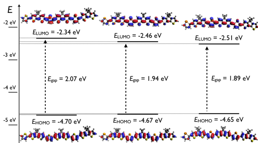
Figure 6. Molecular orbital distribution of HOMO (bottom) and LUMO (top) for C_{16} CPDT-T (left), C_{16} CPDT-T (middle), and C_{16} CPDT-Te (right) at the B3LYP/6-311G(d) level of theory (isodensity = 0.02) and SDD ECP for Se and Te atoms. The absolute values of E_{HOMO} , E_{LUMO} , and E_{gap} shown are obtained by computational means.
