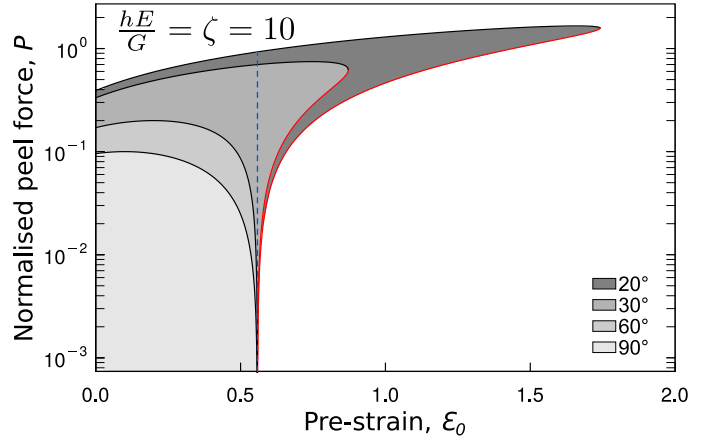
Figure 4: ‘Stability envelopes’ for tape peeling at varying tape pre-strains and peel angles \phi . If the strain exceeds a minimum strain \varepsilon_{\min} (dashed blue line), stable attachment requires the application of the minimum force to stabilise the contact (red line). In this regime, spontaneous detachment occurs whenever the applied force drops below this lower bound, providing a rapid and efficient detachment mechanism.
