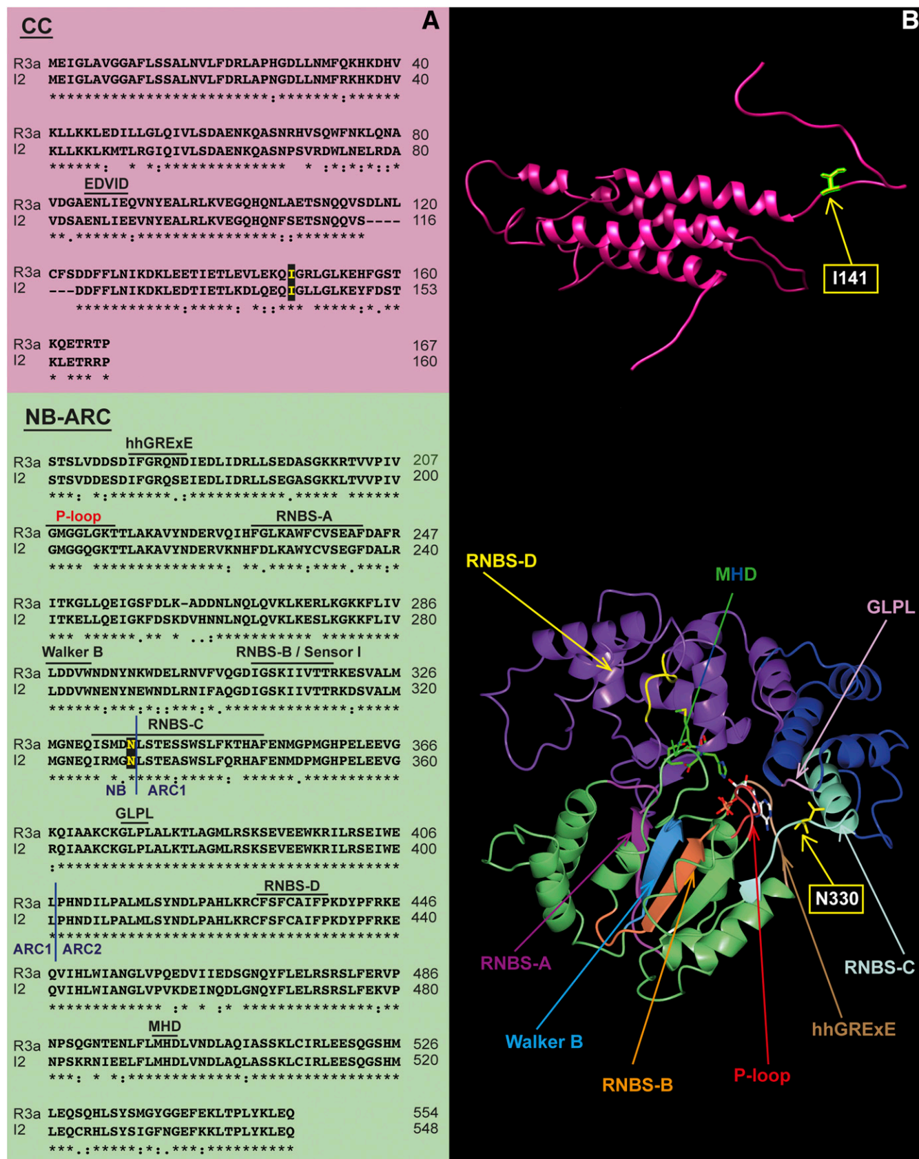
Fig. 2. I2 and R3a are highly similar in the N-terminal region. A , Protein sequence alignment of the CC and NB-ARC domains of I2 and R3a. The amino-acid positions that were subjected to mutation are highlighted in yellow. Conserved R-protein motifs in the NB-ARC domain are overlaid according to van Ooijen et al. (2007). Blue lines delimit the three subdomains of the NB-ARC: NB, ARC1, and ARC2. B , Structural model of the CC and NB-ARC domain of I2. Models were generated by remote homology modeling using the IRTFold2 server (Buenavista et al. 2012; McGuffin et al. 2015). The CC domain is shown in pink, and NB-ARC is shown in three different colors depending on the subdomain: NB (green), ARC1 (purple), and ARC2 (blue). Amino acids corresponding to the single-residue I2 mutations are shown in yellow stick representation. Carbon atoms of ATP are shown in white. Locations of NLR-protein motifs are indicated with arrows.
