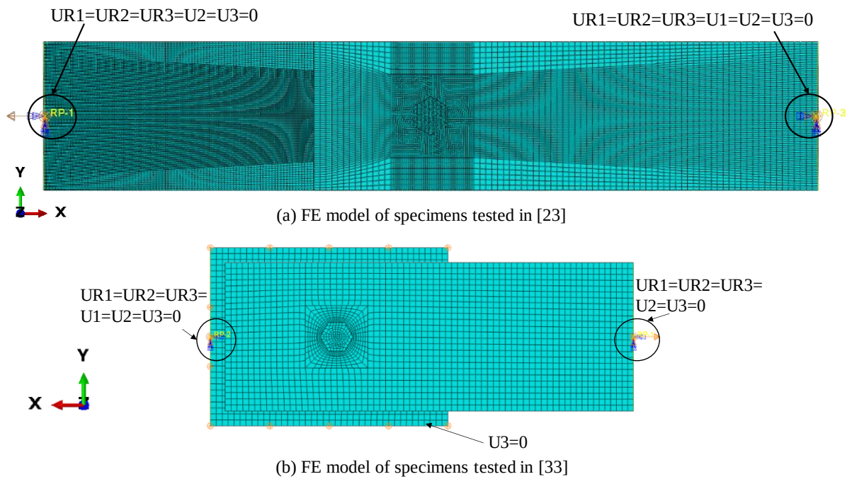
Fig. 9 Mesh and boundary conditions of FE models
