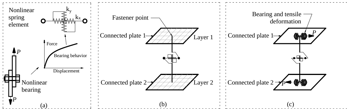
Fig. 4 Modelling of bolted connections using nonlinear springs [27]
