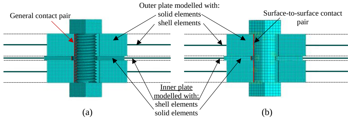
Fig. 7 Cross-section of joint with (a) threaded and (b) non-threaded bolt
