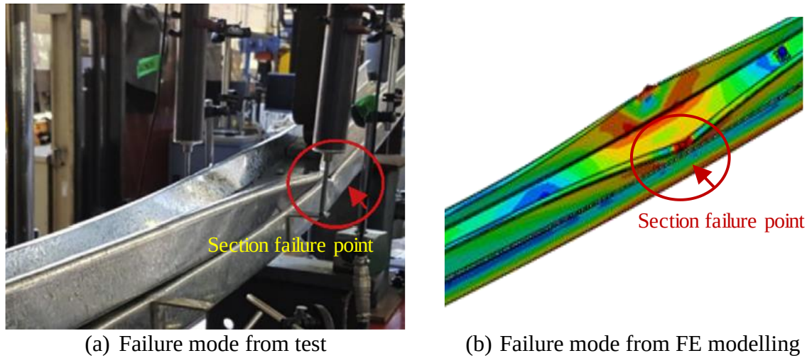
Fig. 20 Typical failure mode of C10010 built-up specimens from: (a) test and (b) FE modelling
