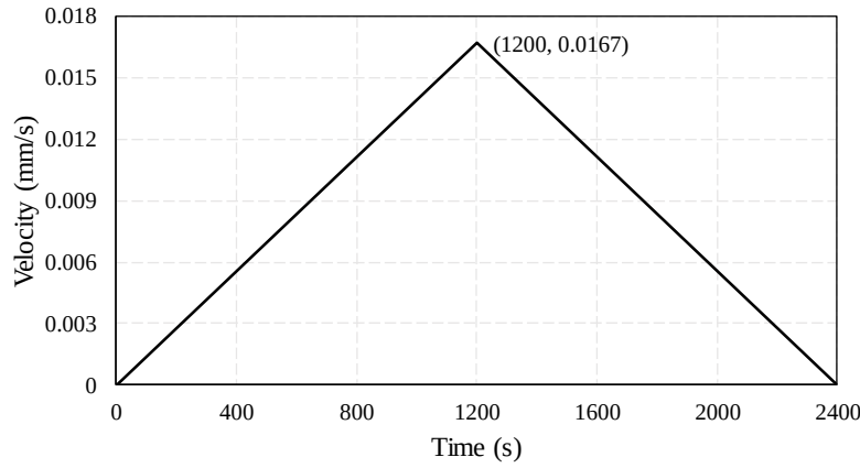
Fig. 10 Velocity-time relationship employed in explicit FE analyses of cold-formed steel lap connections
