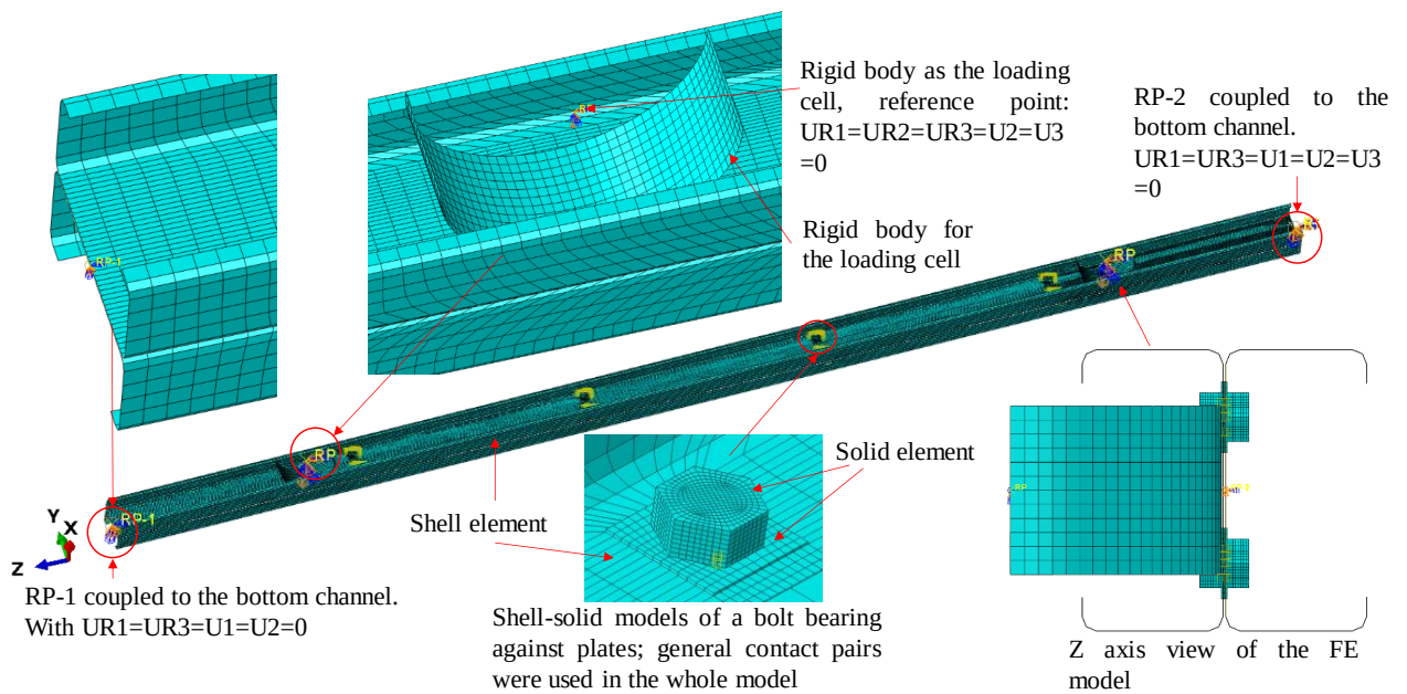
Fig. 16 FE model of specimen C10010-4R-BF
