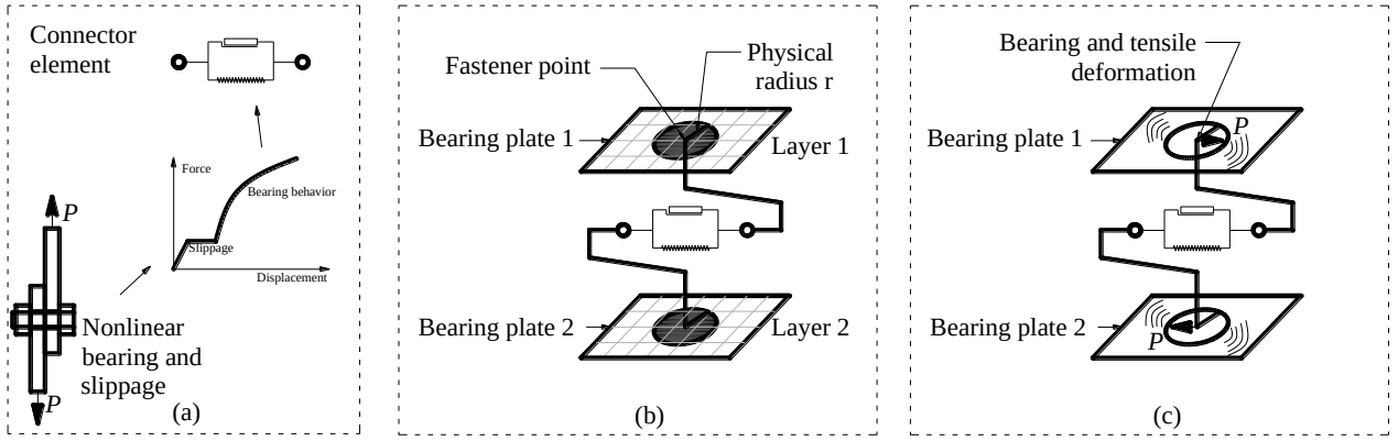
Fig. 5 Use of nonlinear connectors in the modelling of fasteners in bolted connections
