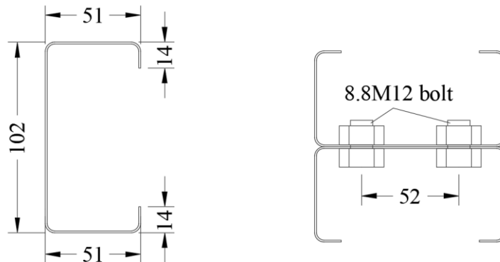
Fig. 15 Nominal dimensions (in mm) of built-up beams tested in [36]
