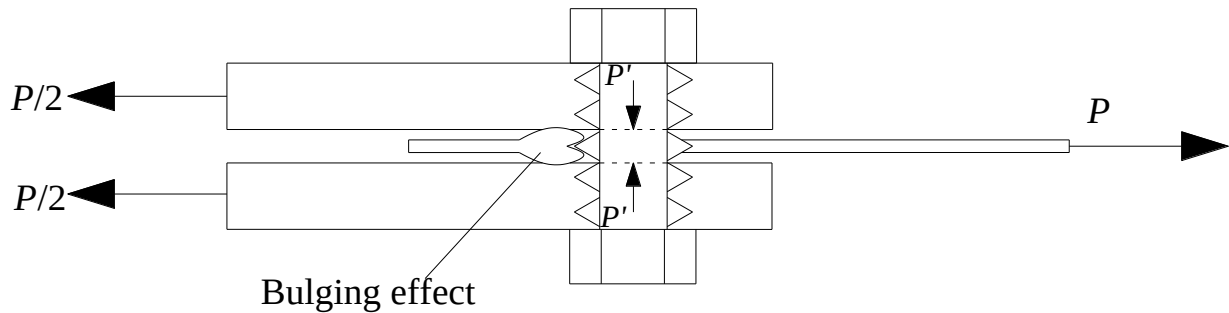
Fig. 3 Thread penetration and bulging effect in thin steel plate, leading to the development of tensile force P' in the bolts
