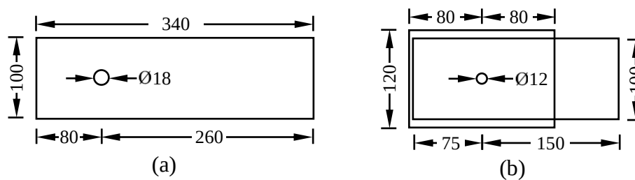
Fig. 8 Nominal dimensions (in mm) of specimens for lap tests reported in: (a) [27] and (b) [37]
