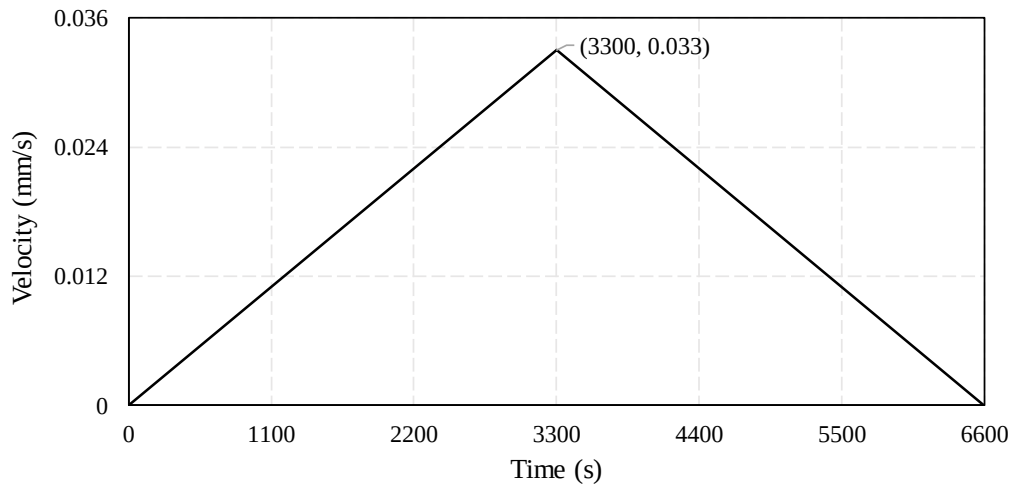
Fig. 17 Velocity-time relationship employed in the explicit FE analyses of cold-formed steel built-up members
