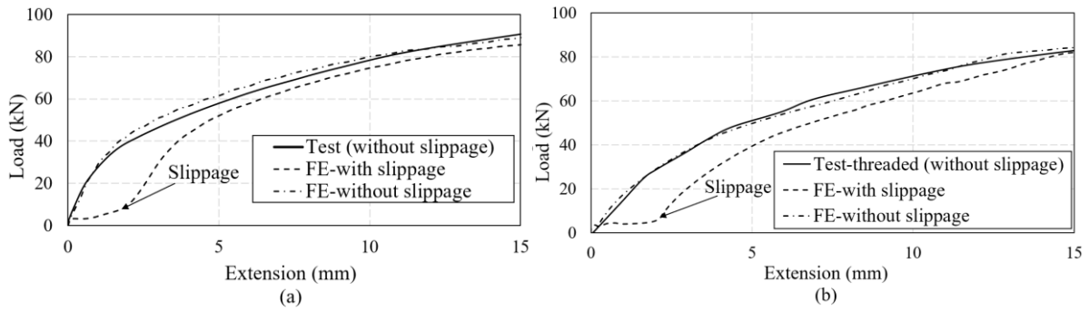
Fig. 14 Load-extension curve of lap joint considering pretension force with: (a) partially-threaded and (b) fully-threaded bolts
