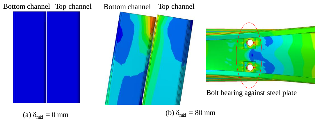
Fig. 21 Slip at the interface between the two channel sections (specimen C10010-2R-B55)
