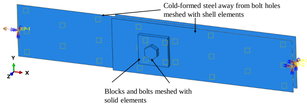
Fig. 6 Use of solid and shell elements in a typical model of a double-shear lap connection
