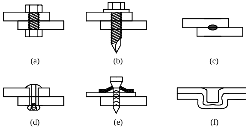
Fig. 1 Fastener types used in cold-formed steel construction: (a) bolts (b) self-tapping screws (c) spot welds (d) blind rivets (e) power actuated fasteners (cartridge fired pins) (f) clinching connections
