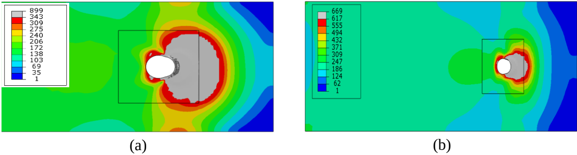
Fig. 12 Von Mises stress contours at 3 mm extension of specimen tested in (a) [27] and (b) [37] (contour units: N/mm 2 )
