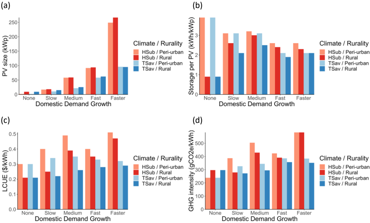
Figure 8 Key metrics associated with an optimal microgrid system across tropical savanna and humid subtropical climates, peri-urban and a rural locations, and rates of domestic demand growth: (a) PV size in year 5, (b) storage per PV in year 5, (c) levelised cost of used electricity, and (d) greenhouse gas emissions intensity.
