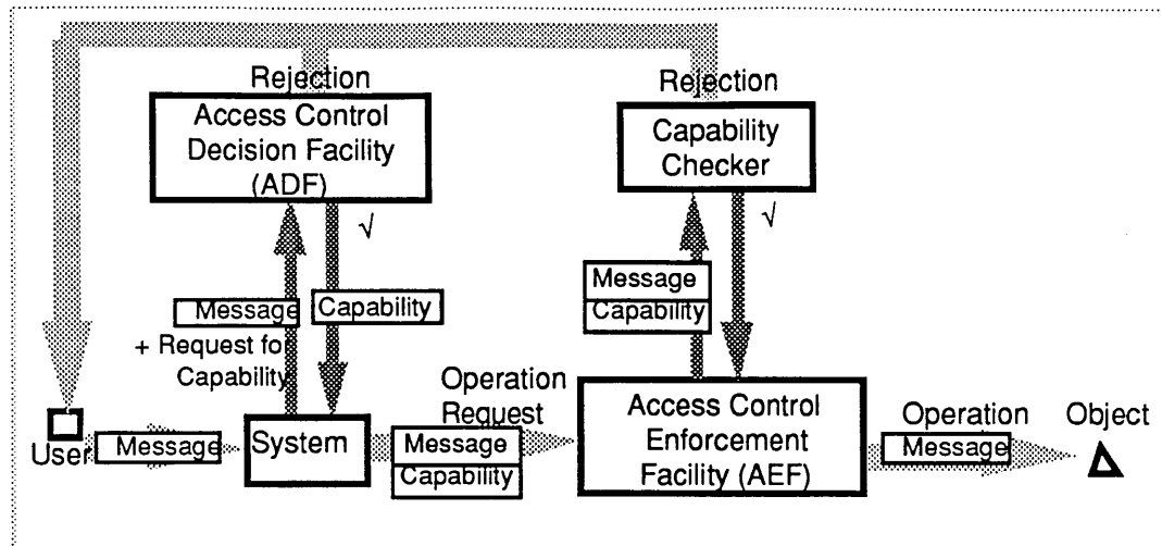
Figure VI.2 ADF Generates Capabilities
