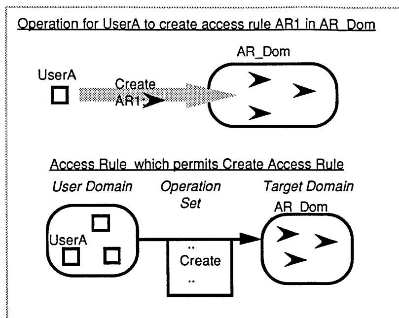
Figure IV.1 Necessary (but not Sufficient) Conditions for Creation of an Access Rule
