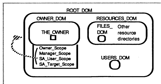
Figure V.1 Root Domain
