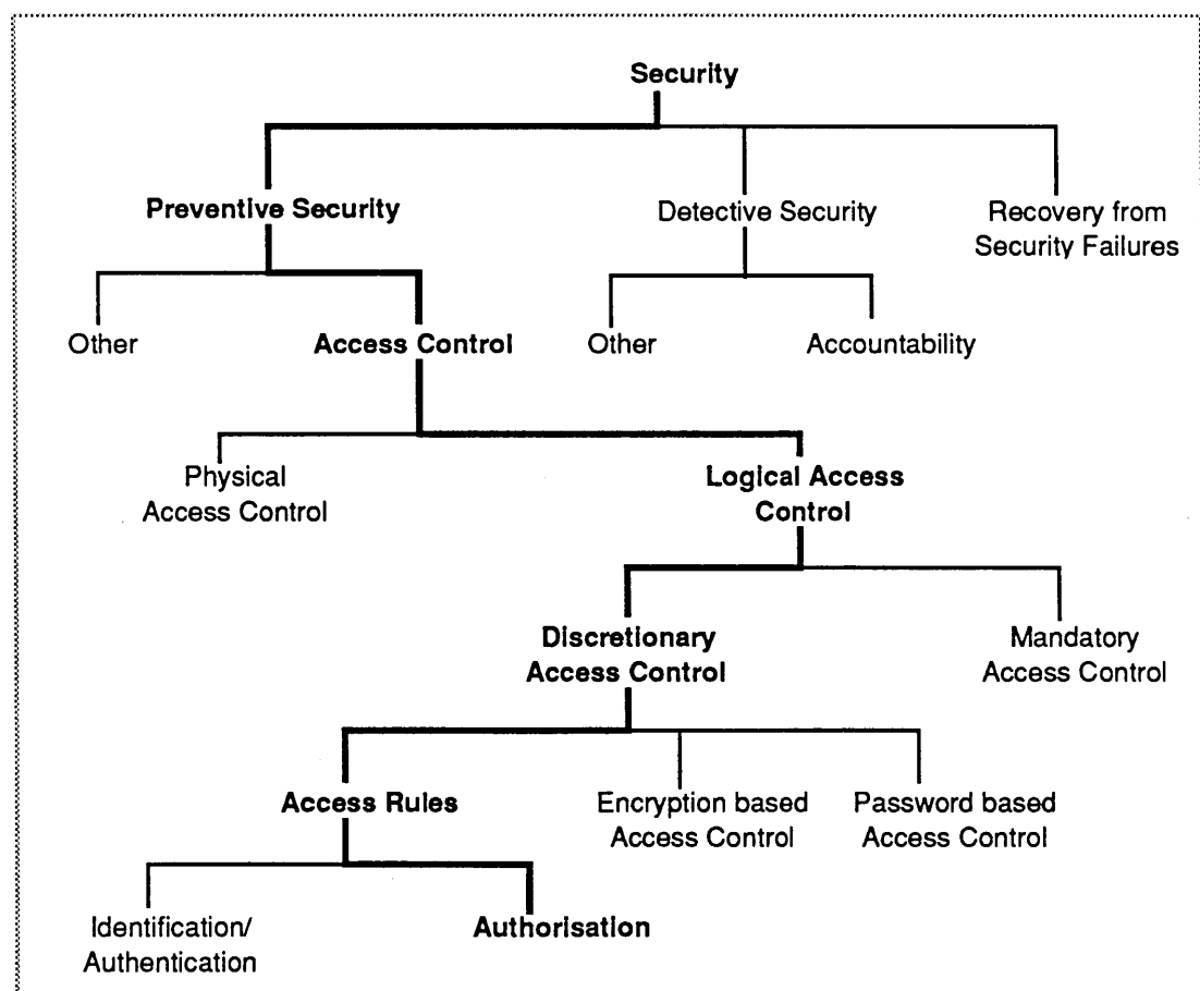
Figure II.1 Security Concepts
