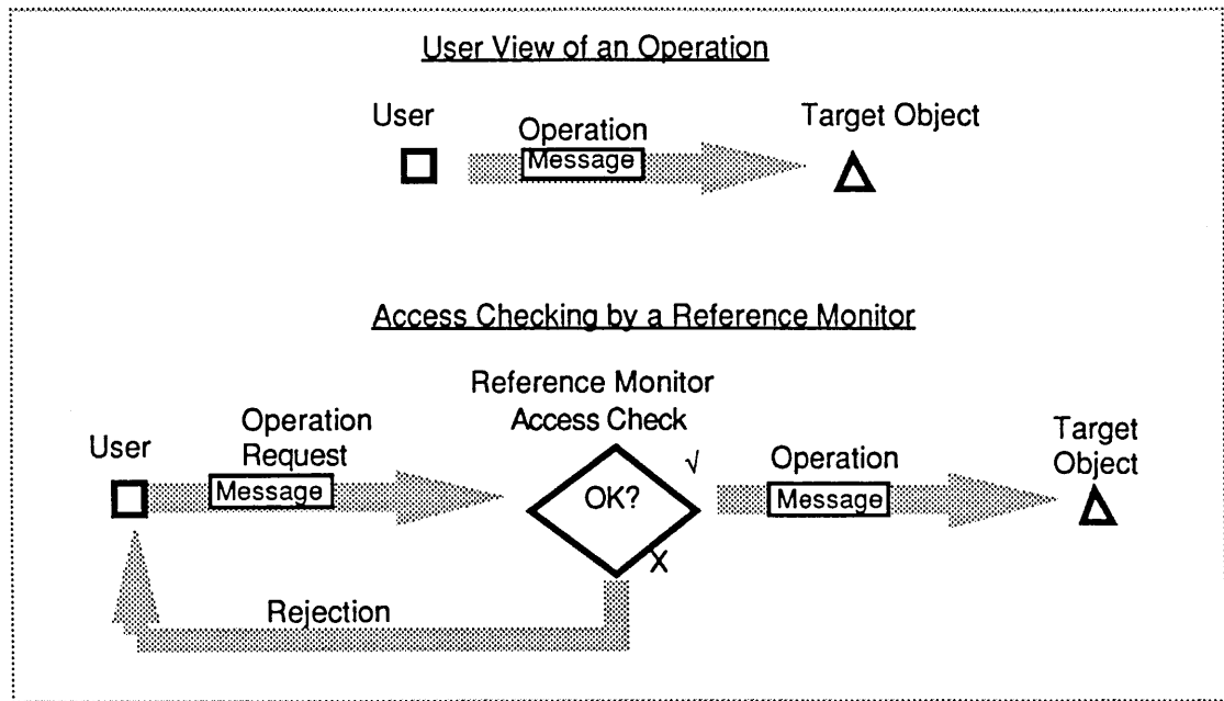
Figure II.2 Reference Monitor Access Check
