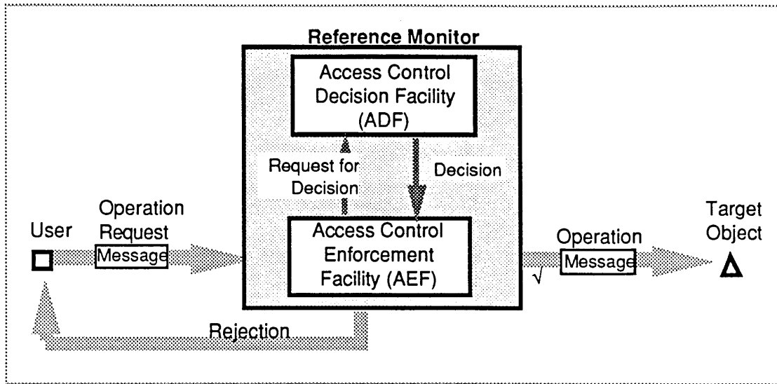
Figure II.3 Reference Monitor Refined by AEF & ADF
