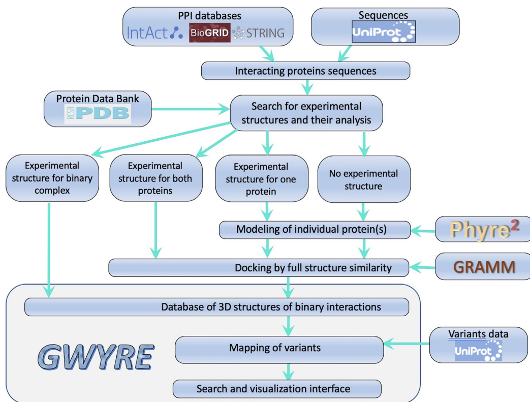
Figure 1. Modeling pipeline.
