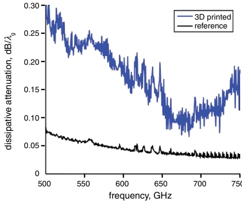
Fig. 6 Calculated dissipative attenuation for WM-380 5 mm 3D printed line (blue) and 25.4 mm reference waveguide (black)
