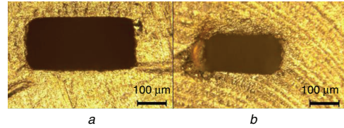
Fig. 2 Micrographs of 3D printed MPRWGs
