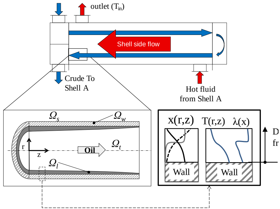
Fig. 4. Sketch indicating the radial location used to explain the radial distribution of the properties in the deposit in Figs. 5-7 (exit of the 2 nd pass of shell B).
