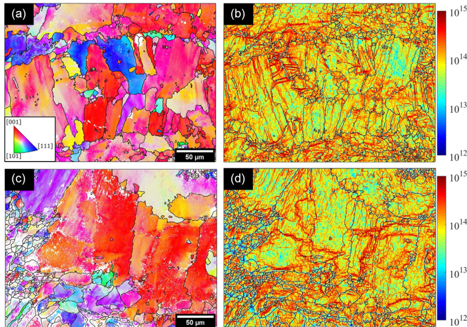
Figure 12. EBSD–IPF along the horizontal LD with their corresponding GND maps, measured in \text{m}^{-2} , in the gauge region near the fracture surface: a,b) B0 condition; c,d) CB67 condition.
