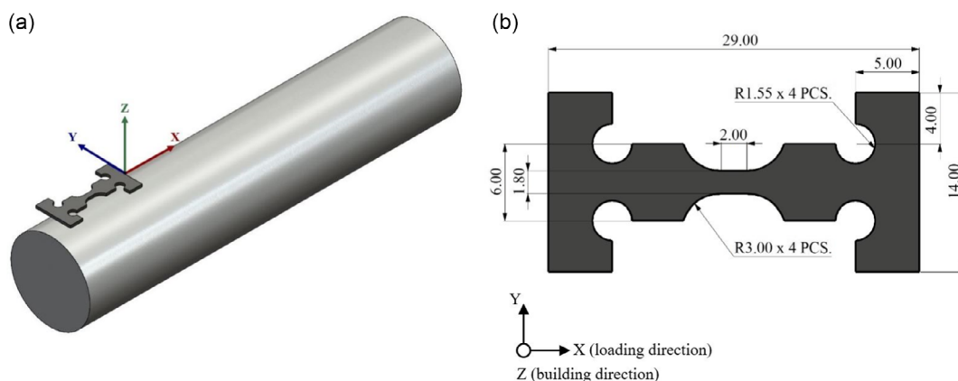
Figure 1. a) Model of the cylinders fabricated by L-PBF. An in situ tensile testing sample is depicted above, showing the test sample was machined along a cylinder fabricated horizontally using L-PBF. b) Dimensions of test samples. Note that the BD was along the Z axis, whereas the uniaxial LD was along X, which coincides with the scanning bidirections of the B0 strategy. All dimensions in mm and figures not to scale.
