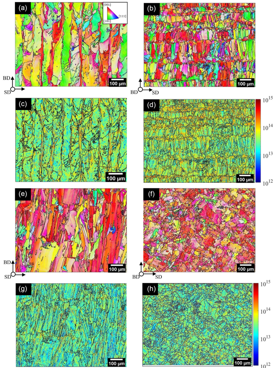
Figure 4. EBSD-IPF of the B0 and CB67 conditions with their corresponding GND spatial distribution maps, measured in \text{m}^{-2} . The B0 condition is presented in a–d), whereas the CB67 is presented in e–h). Note that the left column shows the cross section along the BD with IPF \parallel BD, whereas the right column shows the top view along the SD with IPF \parallel BD.
