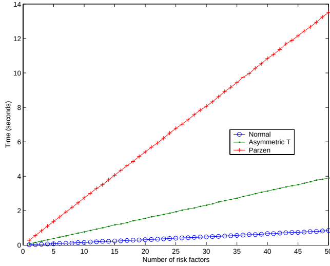
FIG. 3.2. Computation time (in seconds) versus the number risk factors n for the three return models from Section 2. The number of dates in the time series is d = 1000 and the grid has N = 4096 points. As the figure shows, the difference between the models is large implying that the parameter estimation and discretization dominate the actual computation time.
