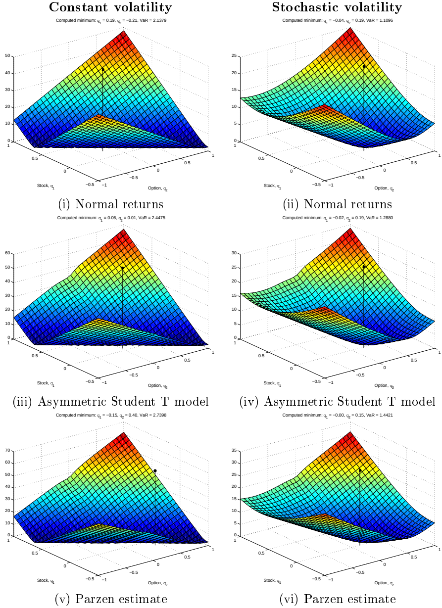
FIG. 4.2. The 99% value-at-risk surface as a function of \theta_1 , the position in Toronto35, and \theta_2 , the position in call options on Toronto35. The point marked is the computed solution to the optimization problem. Volatility as a risk factor changes the shape of the value-at-risk surface and makes the minimum well defined.
