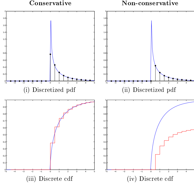
FIG. 3.1. An example of the importance of a discretization method that conserves probability density. Consider \pi = X^2 where X is normal—a \chi^2 random variable with one degree of freedom. For the conservative method, the discrete pdf and cdf are close to the pdf and cdf of the \chi^2 random variable. In the non-conservative method, the pdf is sampled at the grid points to get a discrete approximation. As the graph for the cdf shows, the distribution function for the discrete approximation is not close the original cdf.
