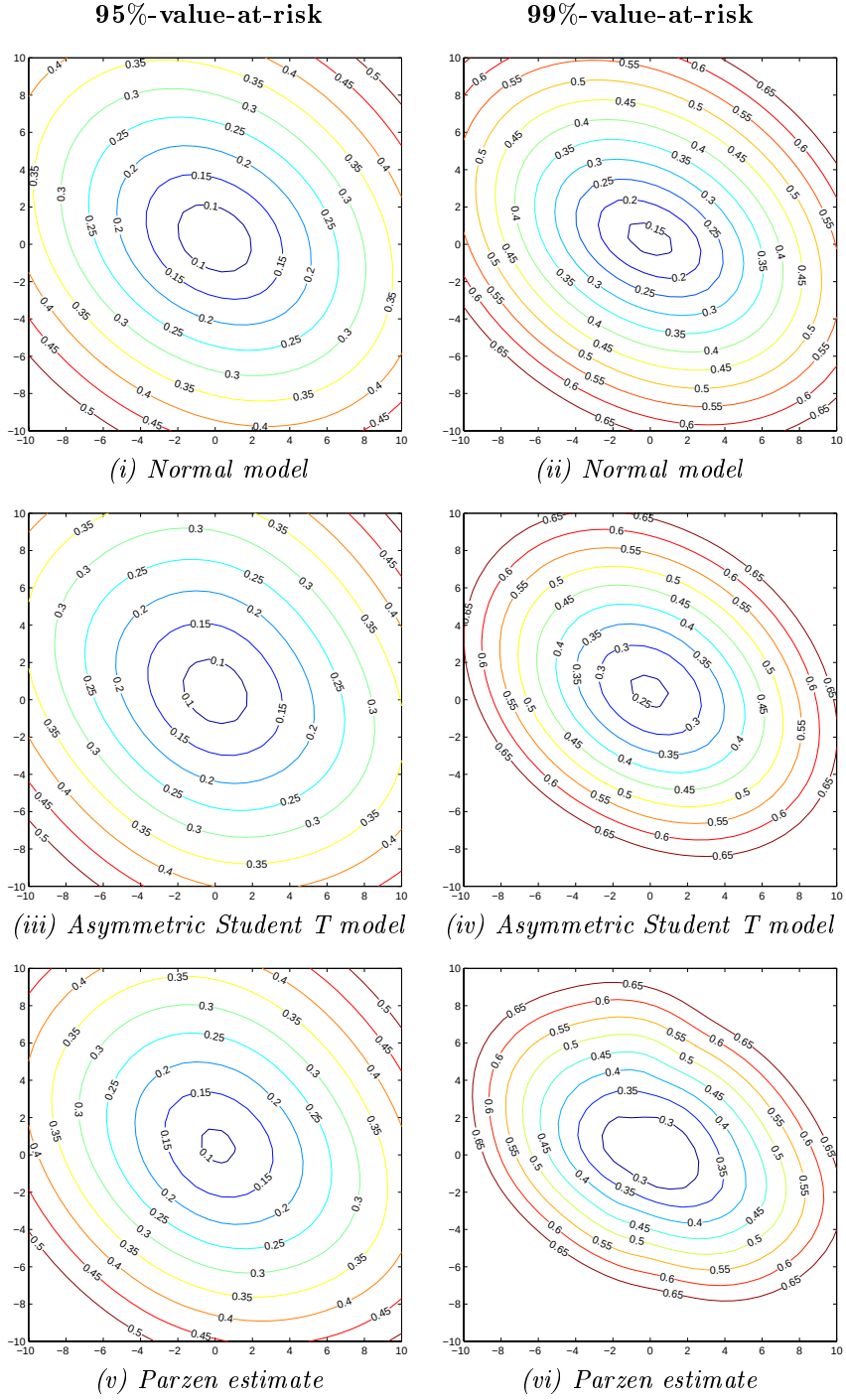
FIG. 4.1. Value-at-risk for a portfolio, with two European call options and positions in the two underlying stocks, as a function of \Delta_1 and \Delta_2 . The horizontal axis is \Delta_1 , the linear position in BCE; and the vertical axis is \Delta_2 , the linear position in CTRa.
