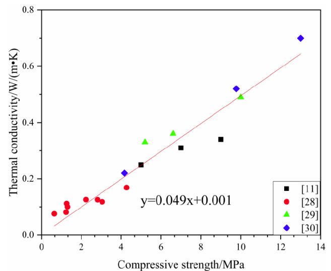
Figure 1: The relationship between thermal conductivity and 28-day compressive strength of concrete with aluminum powder as a foaming agent.
