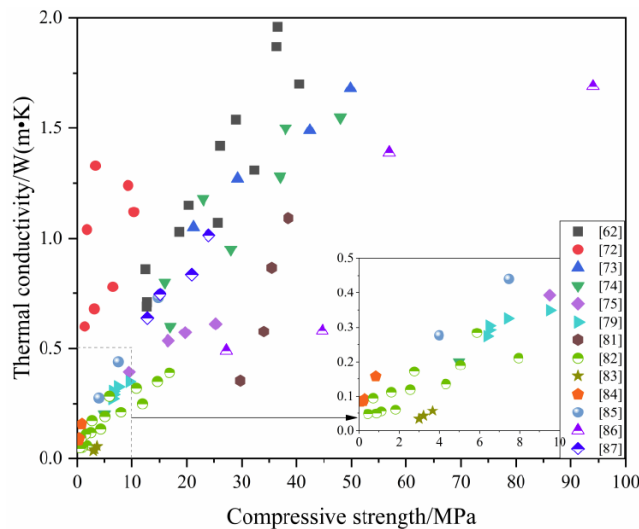
Figure 5: The relationship between thermal conductivity and 28-day compressive strength of concrete with different organic porous aggregates.
