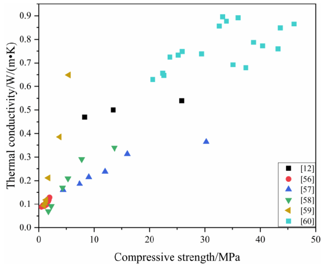
Figure 3: The relationship between thermal conductivity and 28-day compressive strength of concrete with different mechanical foaming materials.
