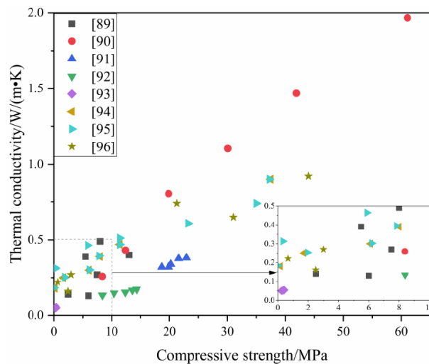
Figure 6: The relationship between thermal conductivity and 28-day compressive strength of concrete with different aerogels.
