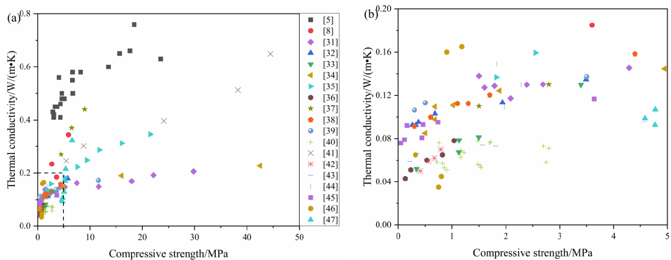
Figure 2: (a) the relationship between thermal conductivity and 28-day compressive strength of concrete with hydrogen peroxide as a foaming agent, (b) zoomed in from 0 to 5 MPa.
