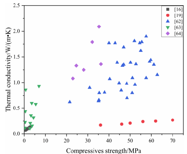
Figure 4: The relationship between thermal conductivity and 28-day compressive strength of concrete with different cenospheres.
