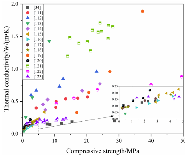
Figure 7: The relationship between thermal conductivity and 28-day compressive strength of concrete with different aggregates.
