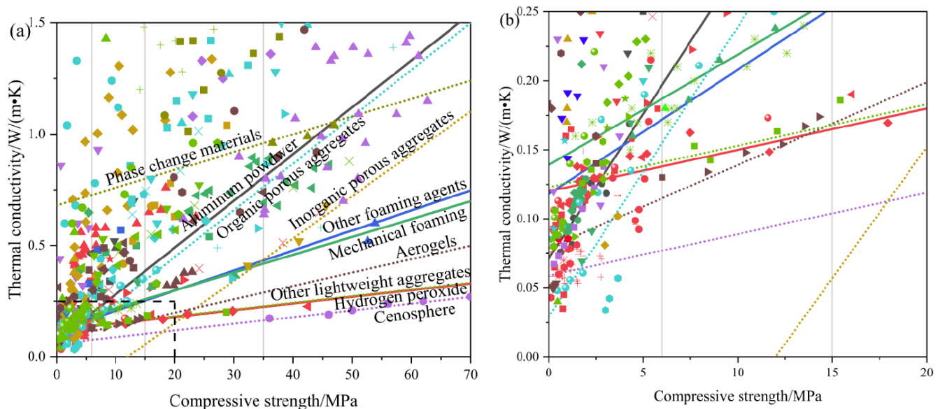
Figure 8: (a) The relationship between thermal conductivity and 28-day compressive strength of the best performance compositions, (b) zoomed in from 0 to 20 MPa.
