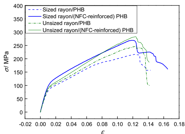
Fig. 6. Typical stress ( \sigma ) – strain ( \epsilon ) curves for sized rayon fibre-reinforced neat and (NFC-reinforced) PHB composites and unsized rayon fibre-reinforced neat and (NFC-reinforced) PHB composites. (For interpretation of the references to colour in this figure legend, the reader is referred to the web version of this article.)
