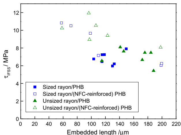
Fig. 3. Apparent interfacial shear stress \tau_{IFSS} as a function of embedded length for sized and unsized rayon fibre-reinforced neat and (NFC-reinforced) PHB single fibre model composites. (For interpretation of the references to colour in this figure legend, the reader is referred to the web version of this article.)
