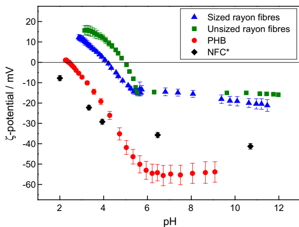
Fig. 2. \zeta -potential as a function of pH for sized and unsized rayon fibres, neat PHB and NFC (Values of zeta potential = f(\text{pH}) of NFC was taken with permission from Ref. [33]). (For interpretation of the references to colour in this figure legend, the reader is referred to the web version of this article.)
