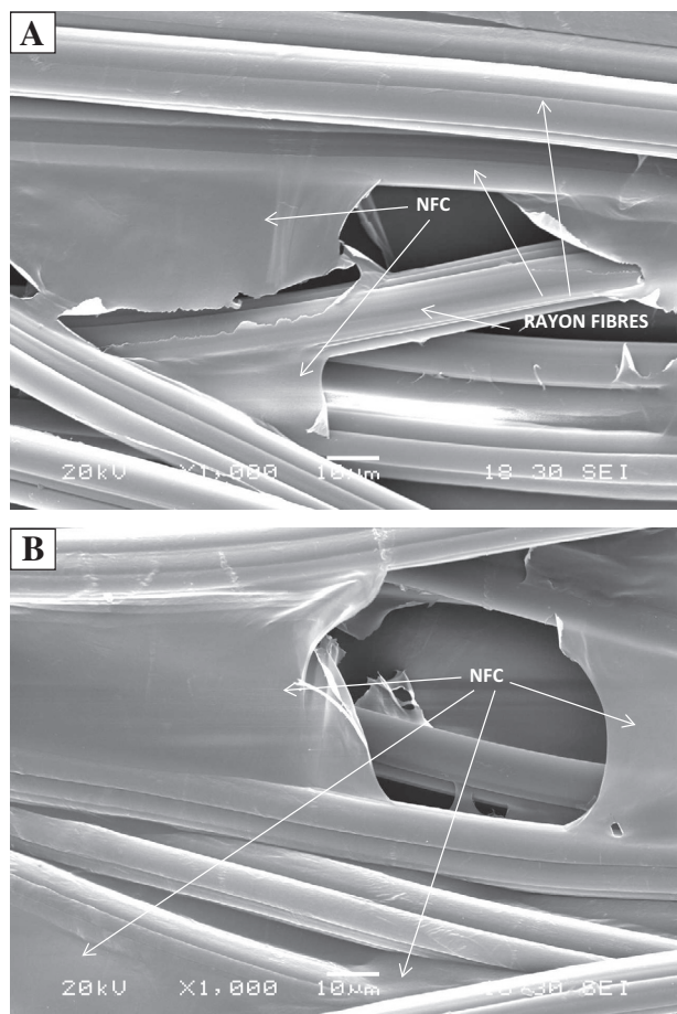
Fig. 5. Scanning electron micrographs of (A) sized and (B) unsized rayon fibres when dipped in a bath of water containing 2.5 wt.% of NFC. The NFC binds the fibres creating a bridge from fibre-to-fibre. (For interpretation of the references to colour in this figure legend, the reader is referred to the web version of this article.)
