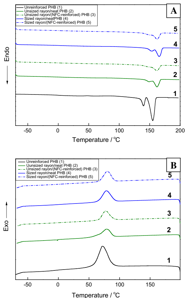
Fig. 4. 2 nd Heating (A) and cooling (B) curves of rayon fibre-reinforced neat and (NFC-reinforced) PHB composites observed during DSC scan. (For interpretation of the references to colour in this figure legend, the reader is referred to the web version of this article.)
