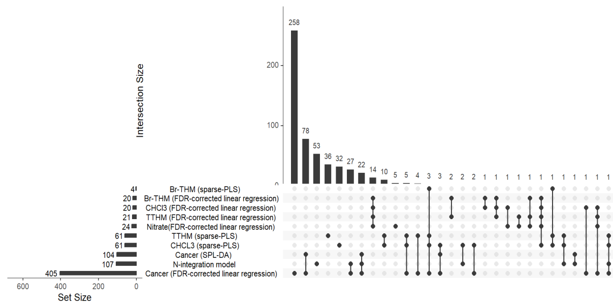
Figure 1. Upset plot showing the number of metabolomic features associated with exposure to water contaminants and colorectal cancer using different statistical models. Multivariate models are sparse-PLS (exposure) or PLS-DA (cancer). The remaining are FDR-corrected linear regression models, or N-integration model (DIABLO). The plot illustrates the intersections between the different models and the number of unique and shared features identified for each contaminant/cancer outcome. The subsets are ordered by frequency. The plot was generated using the R package UpSetR 21 .
