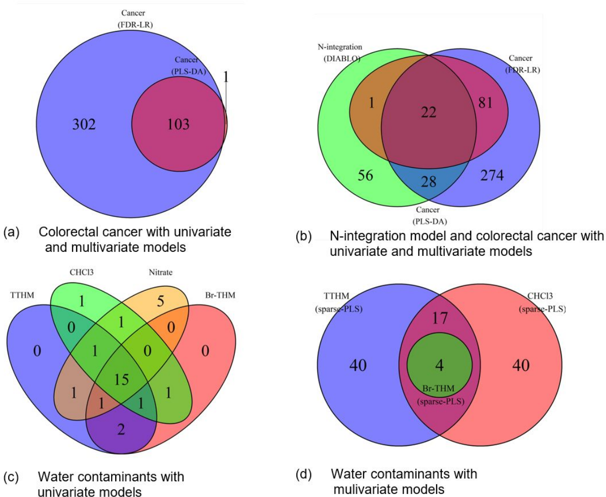
Figure 3. Venn diagrams showing the metabolomic features associated with water contaminants and colorectal cancer using different statistical models and the overlap between models.
