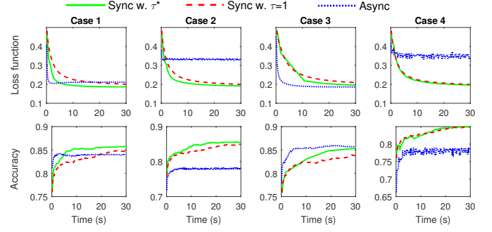
Fig. 10: Synchronous vs. asynchronous distributed DGD with SVM.
