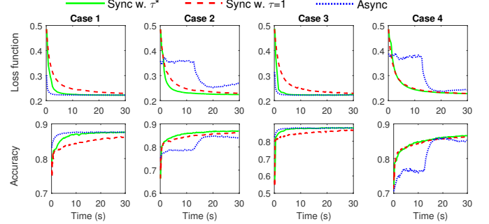
Fig. 11: Synchronous vs. asynchronous distributed SGD with SVM.
