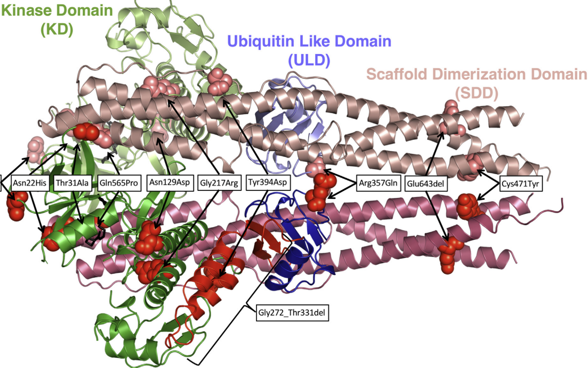
Fig. 1. TBK1 mutations identified to date and their location in TBK1 structure. (A, B) Schematic representation of TBK1 protein structure (Tu et al., 2013) showing a map of nonsense (A) and missense (B) variants found in the literature and in our cohort. For more details on the variants found in this study see Table 1. (C) TBK1 homodimer crystal structure (PDB 4IM0) mapping the mutations found in our study excluding premature stop codons and frameshift deletions. Abbreviations: CTD, C-terminal domain (light blue); KD, kinase domain (green); SDD, scaffold dimerization domain (pink); TBK1, TANK binding kinase 1; ULD, ubiquitin-like domain (purple). (For interpretation of the references to color in this figure legend, the reader is referred to the Web version of this article.)
