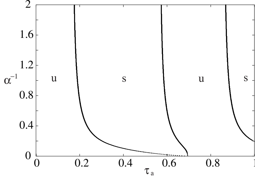
Figure 3: Stability of the synchronous solution \phi = 0 as a function of \alpha^{-1} and \tau_a for weak excitatory coupling with I = 2 . Stable and unstable regions are denoted by s and u respectively. The stability diagrams are periodic in \tau_a with period \ln[I/(I-1)] . (This periodicity would be distorted in the strong coupling regime since the collective period of oscillation depends upon the strength of coupling).
