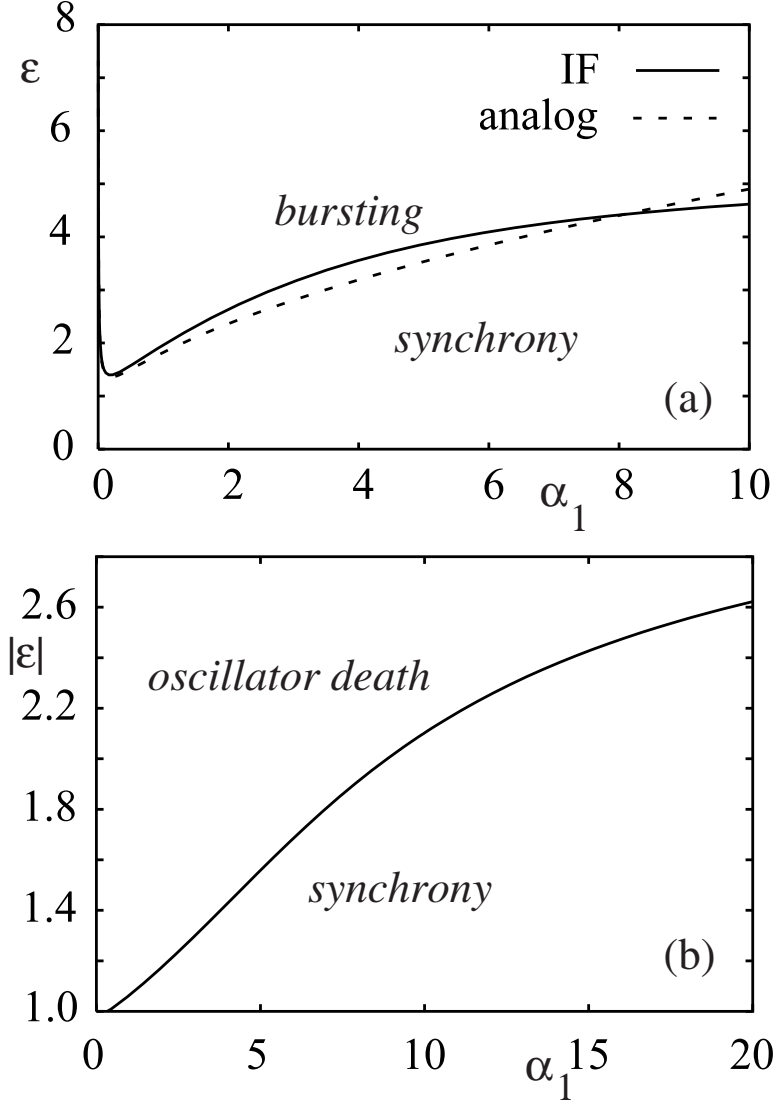
Figure 14: Critical coupling for a bifurcation in the firing times as a function of the rise-time \alpha_1 for fixed decay-time \alpha_2 = 0.2 . (a) Excitatory/inhibitory pair with \epsilon > 0 , W_{11} = W_{22} = 0 , W_{21} = 1 and W_{12} = -2 . Bursting can occur even for fast rise-times. The corresponding critical coupling for the analog model is shown as a dashed curve. (b) Inhibitory pair of IF neurons with \epsilon < 0 , W_{11} = W_{22} = 0 , W_{21} = W_{12} = 1 . Critical coupling is only weakly dependent on \alpha_1 .
