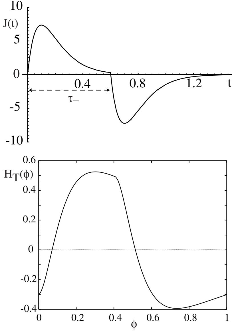
Figure 1: (a) Delay kernel J(t) and (b) associated interaction function H_T(\phi) for a combination of excitatory and delayed inhibitory synaptic interactions given by equation (3.12). Here \alpha_{\pm} = 10 , \tau_+ = 0 , \tau_- = 0.6 and T = \ln 2 .
