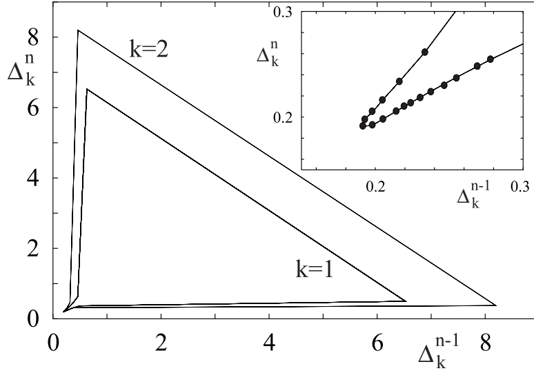
Figure 9: A plot of the inter-spike intervals (\Delta_k^{n-1}, \Delta_k^n) of the spike trains shown in Fig. 8a illustrating how they lie on closed periodic orbits. Points on an orbit are connected by lines. Note that each triangular region is associated with only one of the neurons, highlighting the difference in inter-burst intervals (see also Fig. 8a). The inset is a blow up of orbit points for one of the neurons within a burst.
