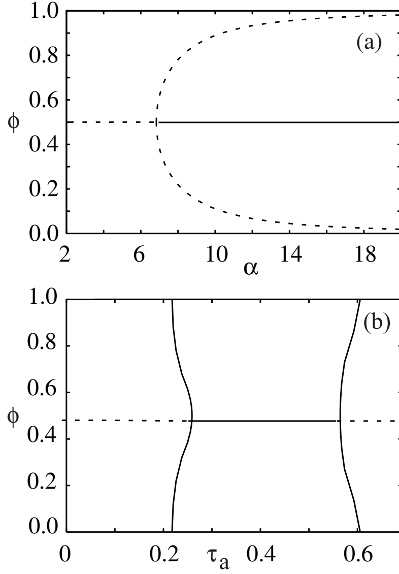
Figure 2: (a) Relative phase \phi = \phi_2 - \phi_1 for a pair of IF oscillators with symmetric inhibitory coupling as a function of \alpha with I = 2 . In each case the anti-phase state undergoes a bifurcation at a critical value of \alpha = \alpha_c where it becomes stable and two additional unstable solutions \phi , 1 - \phi are created. The synchronous state remains stable for all \alpha . (b) Relative phase \phi vs. discrete delay \tau_a for a pair of pulse-coupled integrate-and-fire oscillators with I = 2 and \alpha = 2 .
