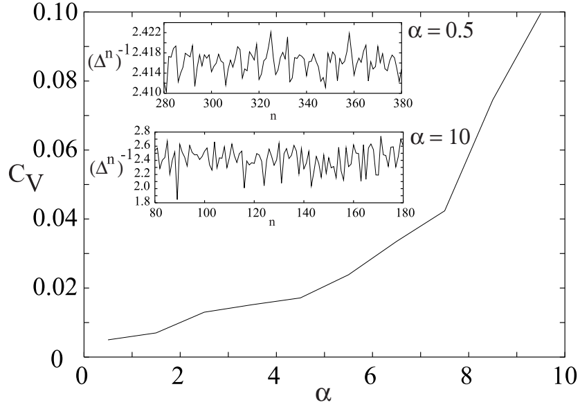
Figure 13: Plot of the coefficient of variation C_V for a single IF oscillator as a function of the inverse rise-time \alpha . All other parameter values are as in Fig. 12. For each \alpha , the oscillator is chosen to be one with the maximum mean firing rate. Insets: Time series showing variation of the inverse ISI (\Delta^n)^{-1} with n for two particular values of \alpha .
