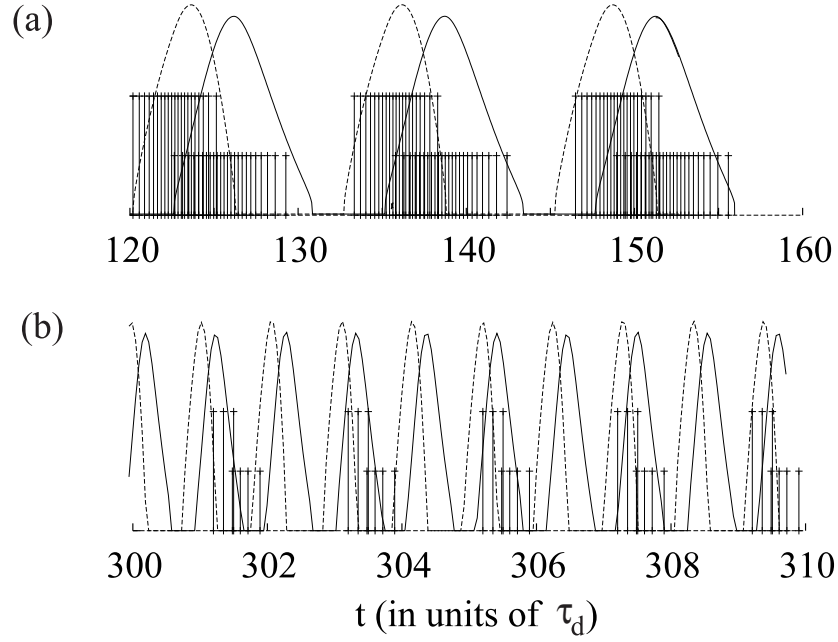
Figure 8: Spike train dynamics for a pair of IF neurons with both excitatory and inhibitory coupling corresponding to points A and B in Fig. 7 respectively. The firing times of the two oscillators are represented with lines of different heights (marked with a + ). Smooth curves represent variation of firing rate in the analog version of the model.
