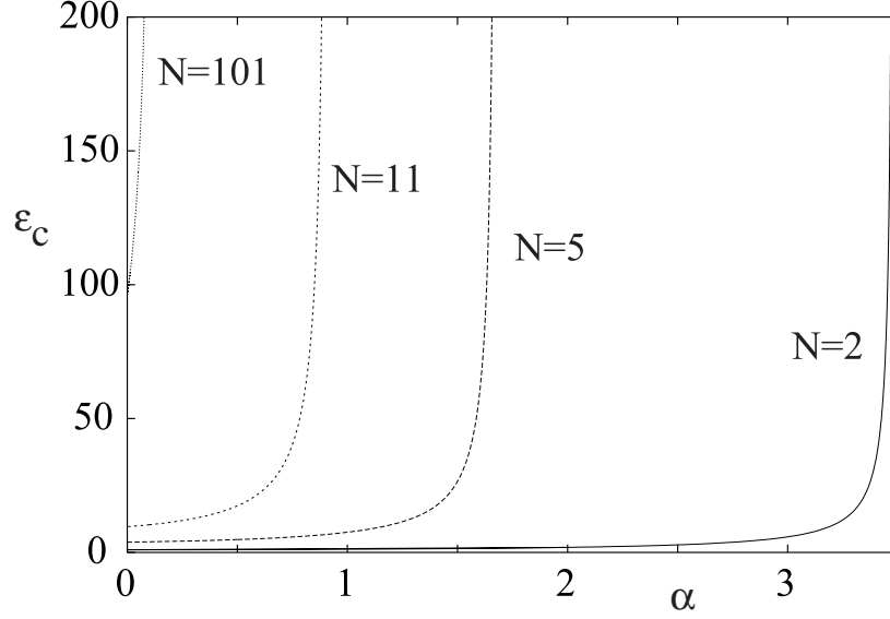
Figure 6: Plot of critical coupling \epsilon_c as a function of \alpha for various network sizes N . The critical inverse rise-time \alpha_0(N) is seen to be a decreasing function of N with \alpha_0(N) \rightarrow 0 as N \rightarrow \infty .
