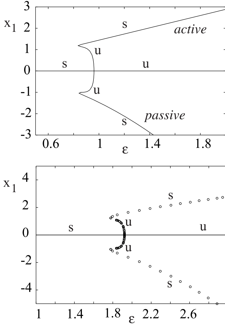
Figure 4: (a) Bifurcation diagram for a pair of analog neurons with symmetric inhibitory coupling and external input I = 2 . (b) Subcritical Hopf bifurcation for a pair of analog oscillators with self-interactions. \alpha = 0.5 , I = 2 , W_{11} = W_{22} = 0 , W_{21} = 1 and W_{12} = -2 . Open circles denote the amplitude of the resulting limit cycle from the Hopf bifurcation point \epsilon \approx 2.0 . Also 's' ('u') stands for stable (unstable) dynamics.
