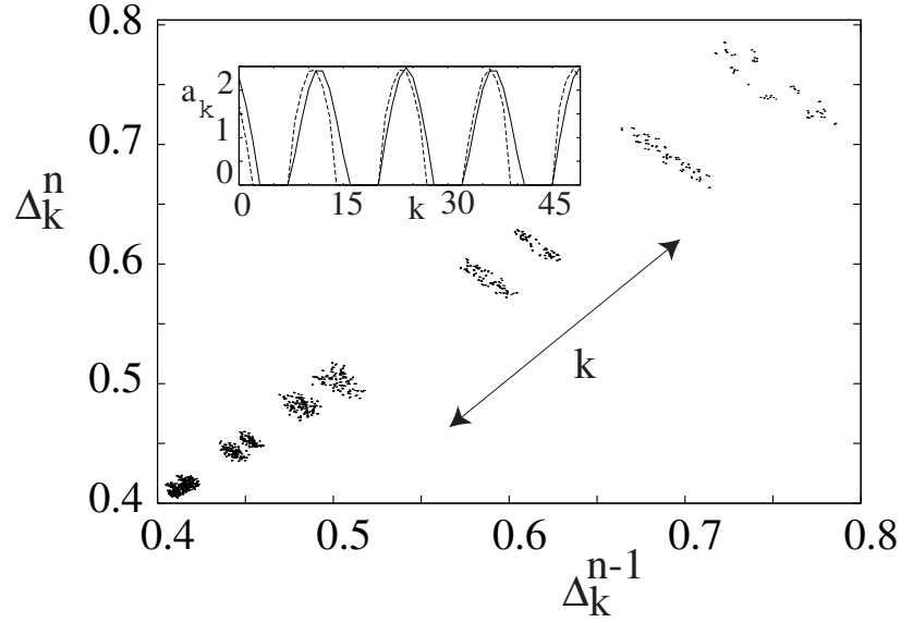
Figure 12: Separation of the inter spike interval orbits in phase-space for a ring of N = 51 IF corresponding to point A in Fig. 11 ( \alpha = 2 , \epsilon = 0.4 ). The attractor of the embedded inter-spike interval (ISI) with coordinates, (\Delta_k^{n-1}, \Delta_k^n) , is shown for all N neurons. Inset: Regular spatial variations in the long-term average firing rate a_k (dashed curve) are in good agreement with the corresponding activity pattern (solid curve) found in the analog version of the network constructed in section 3.2 with a_k now determined by the mean firing rate function (3.18).
