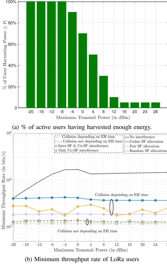
Figure 7: (a) The proportion of active users having harvested enough energy and (b) the minimum throughput rate of LoRa users versus maximum transmit power with density 2000 users per \text{km}^2 .
