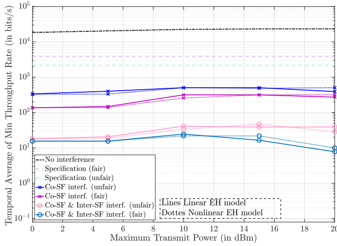
Figure 14: Temporal average of minimum data rate vs P_t in dBm with K = 4 , and SF \in \{7, 8, 9\} .
