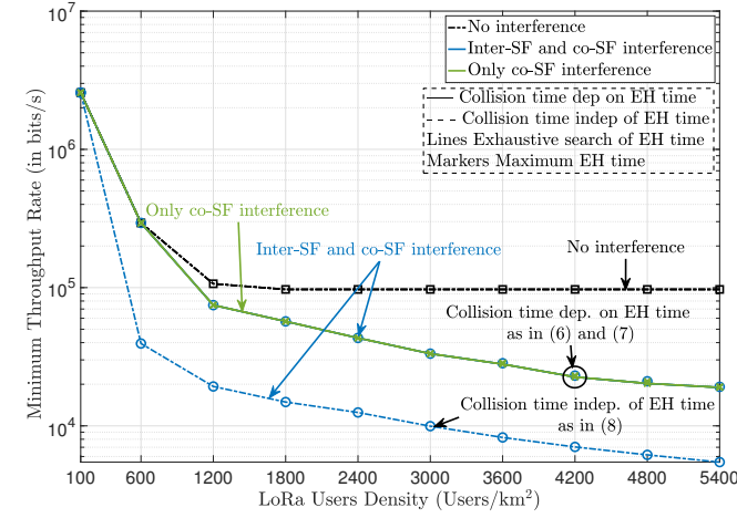
(a) Exhaustive search vs maximum EH time for unfair SF allocation.
