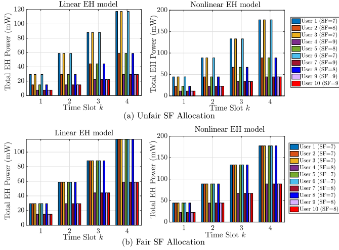
Figure 13: Example of the total harvested power for 10 exemplary users with K = 4 .
