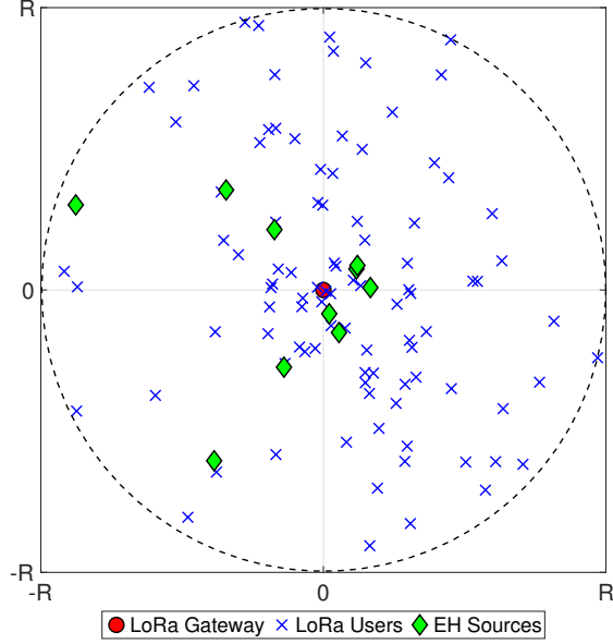
Figure 4: An example of LoRa network consisted of one gateway and LoRa users with density 10^4 Users/km 2 harvesting from power beacons with density 10^3 PBs/km 2 .
