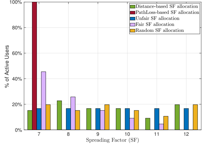
Figure 5: Allocation of active users to different SF \in \{7, \dots, 12\} according to different allocation algorithms, for a density 10^4 Users/km 2 .
