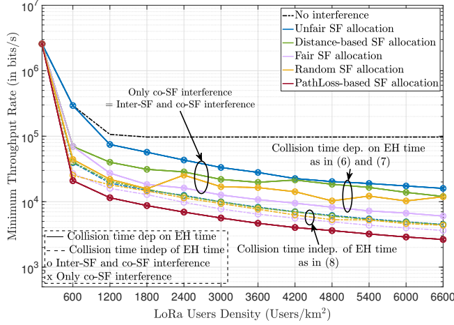
(b) Packet collision time either depending on EH time or not, with maximum EH time.
