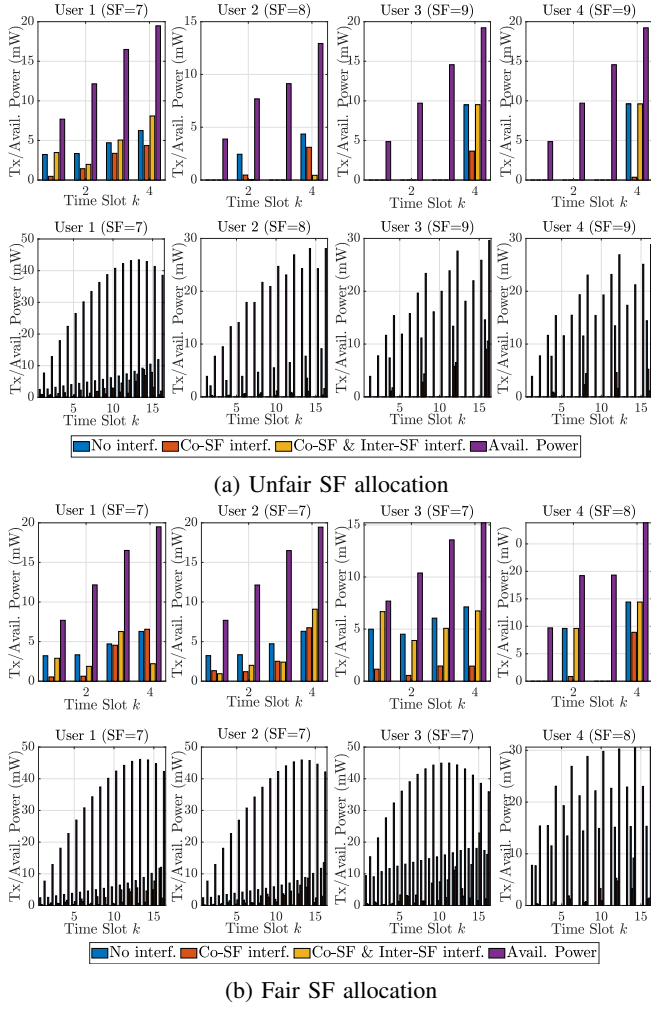
Figure 9: Example of transmit power and available power for 4 users for (a) unfair SF allocation and (b) fair SF allocation, with K = 4 and K = 16 .
