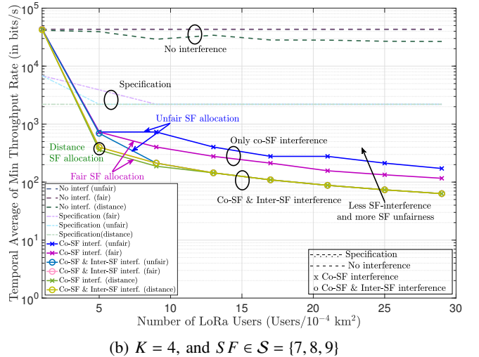
Figure 11: Temporal average of minimum data rate vs LoRa users density per km 2 for different SF allocation algorithms, and different interference scenarios, with P_t = 17\text{dBm} .
