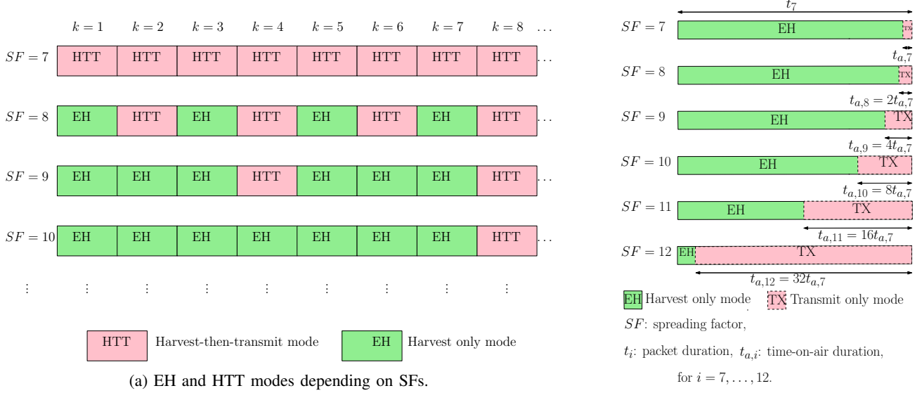
Figure 2: Illustration of maximum number of transmission attempts a_{n,max} and EH modes per SF during T with K time slots of width t_7 .
