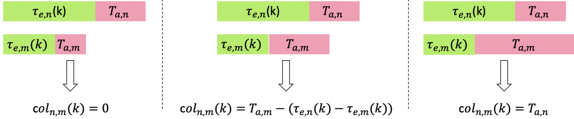
Figure 3: Collision time depending on EH time for \tau_{e,n}(k) > \tau_{e,m}(k) if two users start to transmit at the same time slot k .
