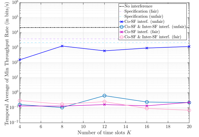
Figure 10: Temporal average of minimum throughput rate vs number of time slots K , with P_t = 17\text{dBm} , SF \in \{7, 8, 9\} , and density 4 \times 10^4 users/km 2 .
