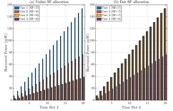
Figure 8: Example of the total harvested power for 4 users for (a) unfair SF allocation and (b) fair SF allocation, with K = 20 , and SF \in \{7, 8, 9\} .
