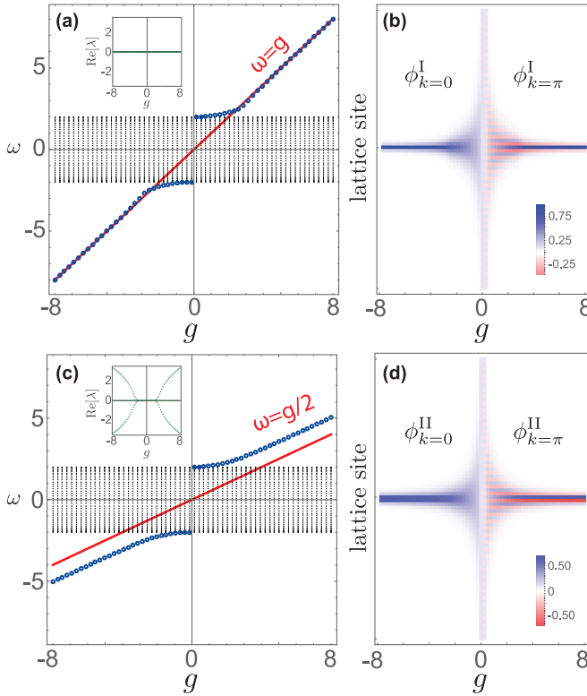
FIG. 10. Numerical breather solutions in the DNLSE [Eqs. (1) and (B1)] with \epsilon = 1 . (a) Linear spectrum (black) and one-site breather energies (blue). The inset shows the real part of the stability eigenvalues \text{Re}[\lambda] . (b) Breather profiles \phi_R . Blue (red) represents positive (negative) components. (c) and (d) Same as (a) and (b) but for two-site breathers.
