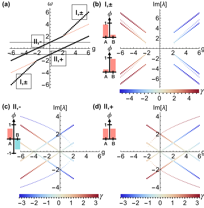
FIG. 1. Analytical molecular limit breather solutions of the nonlinear SSH chain [Eqs. (12) and (24)] for m = 1 , \epsilon = 0 . (a) Breather frequencies derived in Sec. IV B. The frequencies of linearly stable (unstable) breather solutions are shown with thick-black (thin-red) dots. The linear SSH spectrum at \omega = \pm m is indicated by gray-horizontal lines. (b)–(d) Linear stability spectrum \text{Im}[\lambda] and Krein eigenvalues \gamma of the stable breather solutions (the curves terminate when the respective solution becomes unstable). Here, nondegenerate (macroscopically degenerate) stability eigenstates are indicated by thin (thick) dots (see Sec. III B for details). At nonlinearity |g| > 2 , there exist two degenerate stable breathers [solutions (I, \pm )] that are mostly localized on either the A (+) or B (−) site and exchanged by inversion symmetry. In the limit g \rightarrow \infty , these modes approach delta-localized breathers (see also Appendix B). At g < 2 ( g > -2 ) respectively, a further breather mode exists [solutions (II, \pm )] that continuously connects to the SSH band at \omega = m ( \omega = -m ). These “band” breathers share their inversion eigenvalue and center of mass with the Wannier states of the respective linear band.
