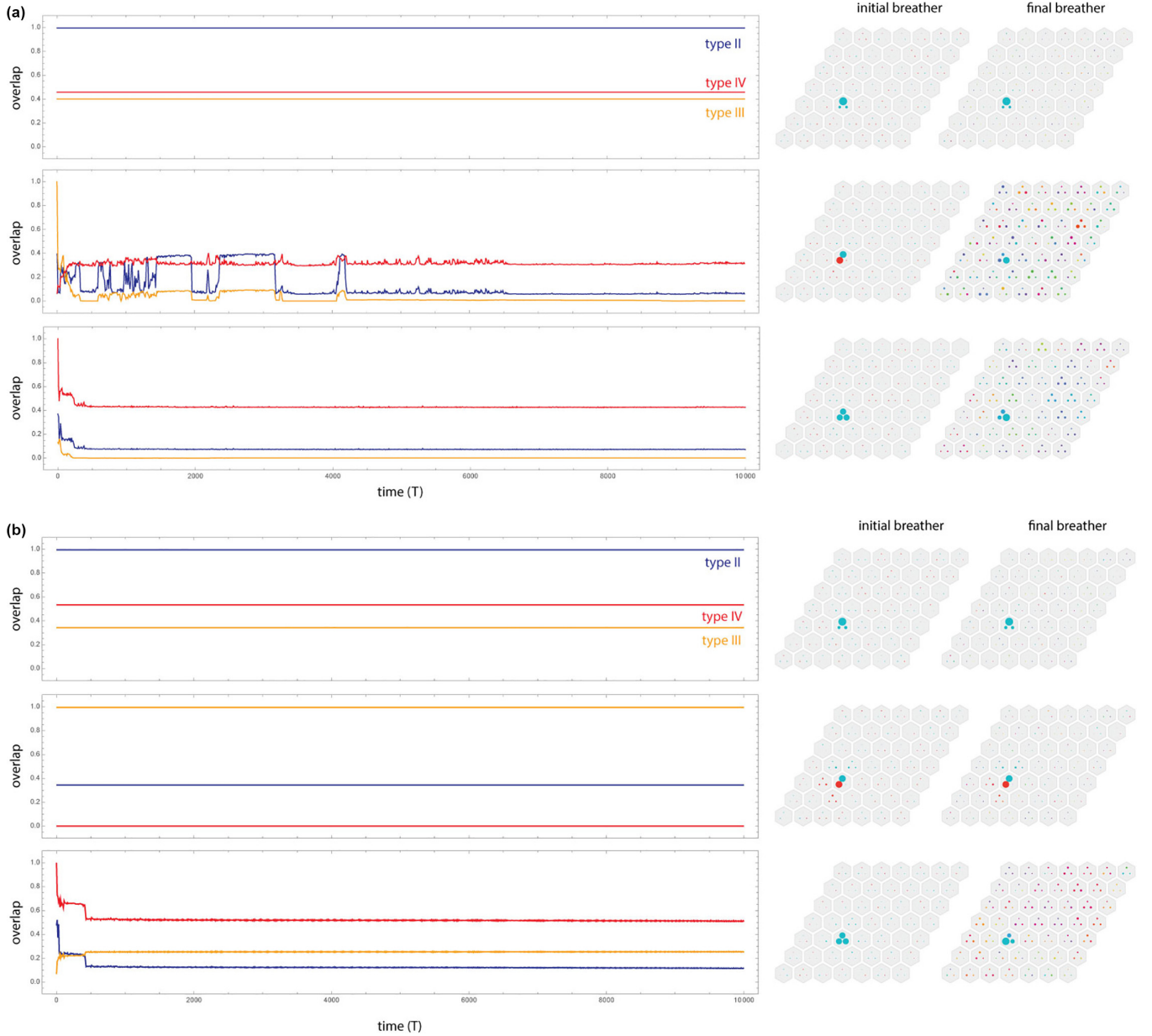
FIG. 11. Time-evolution of breathers in the nonlinear Kagome lattice with real-space hopping matrix (37) under small perturbations. The parameters of the lattice are m = 1 and \epsilon = 0.1 . The strength of nonlinearity is set to g = -12 in (a) and g = -8 in (b). At these values of g , there are three breather solutions: \phi^{(II)} , \phi^{(III)} , and \phi^{(IV)} . The initial fields are \phi^{(i)}(t = 0) = \phi^{(i)} + \phi_{\text{pert}} , for i = \text{II, III, and IV} , where \phi_{\text{pert}} is a random field drawn from a uniform distribution between \pm 0.01 . The fields \phi^{(i)}(t = 0) are normalized to have unit magnitude, which is preserved throughout the time evolution. Each plot corresponds to one time evolution, and the blue, red, and yellow lines indicate the overlaps (inner product) of the instantaneous field with the unperturbed breathers \phi^{(i)} . The simulations were performed using the RK4 algorithm with a time step \Delta t = 0.005 and run for 10 000 breather periods.
