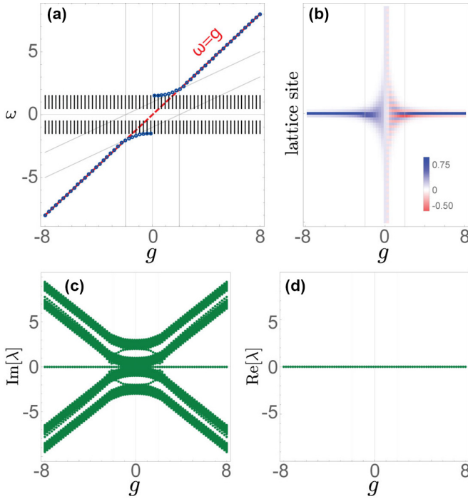
FIG. 2. Numerical breather solutions of Type (I, \pm ) ( |g| > 2 ) and Type (II, \pm ) ( |g| \leq 2 ) in the nonlinear SSH chain [Eqs. (12) and (24)] with m = 1 and \epsilon = 0.5 . (a) Linear spectrum (black) and breather frequencies (blue). (b) Spatial profiles \phi_{(R,\alpha)} . Blue (red) color represents positive (negative) components. (c) and (d) Linear stability eigenvalues \lambda .
