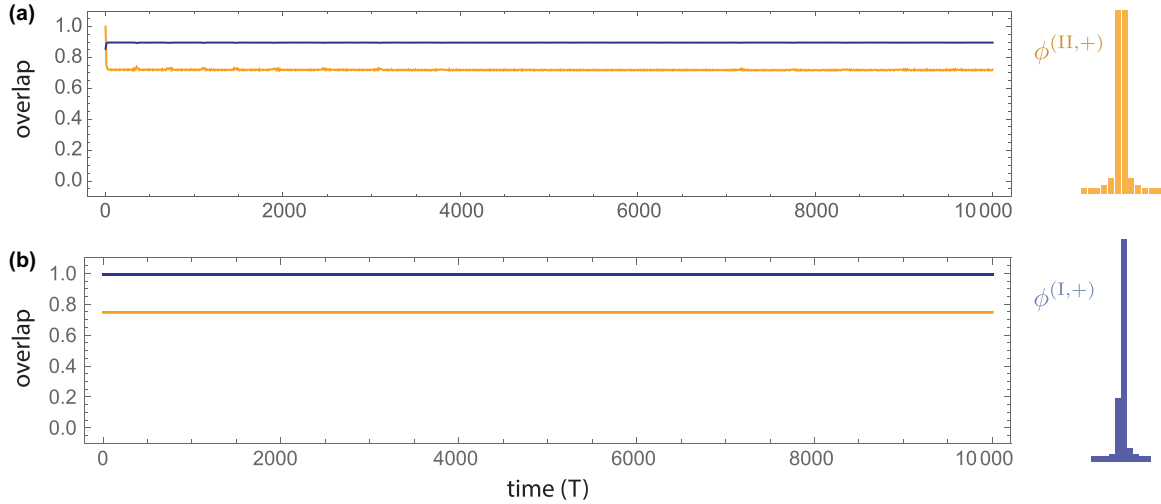
FIG. 4. Time evolution of linearly stable vs linearly unstable breathers in the nonlinear SSH chain under small perturbations. The parameters of the SSH chain are m = 1 and \epsilon = 0.15 . The strength of nonlinearity is set to g = -4 . At this value of g , there are two breather solutions: \phi^{(I,+)} , stable, and \phi^{(II,+)} , unstable. In (a), the initial field is \phi^{(a)}(t=0) = \phi^{(II,+)} + \phi_{\text{pert}} , while in (b), it is \phi^{(b)}(t=0) = \phi^{(I,+)} + \phi_{\text{pert}} , where \phi_{\text{pert}} is a random field drawn from a uniform distribution between \pm 0.02 . The fields \phi^{(a)}(t=0) and \phi^{(b)}(t=0) are normalized to have unit magnitude, which is preserved throughout the time evolution. The yellow and blue lines correspond to the overlaps of the instantaneous fields with the unperturbed breathers \phi^{(II,+)} and \phi^{(I,+)} , respectively. The simulations are performed using the RK4 algorithm with time step \Delta t = 0.005 and run for 10 000 breather periods.
