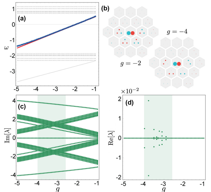
FIG. 9. Numerical breather solutions of Type III in the nonlinear breathing kagome lattice [Eqs. (12) and (37)] with m = 1 , \epsilon = 0.25 . (a) Analytical (red line) and numerical (blue dots) frequency \omega . (b) Breather profiles \phi_{(\mathbf{R},\alpha)} for g = -2 and g = -4 . (c) and (d) Stability eigenvalues \lambda . Instabilities develop in the region |g| \approx -3m (absent in the molecular limit), where stability eigenvalues with opposite Krein eigenvalues collide [Fig. 7(d)].
