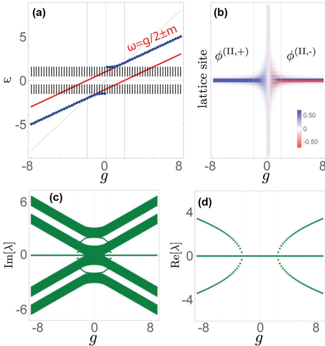
FIG. 3. Numerical breather solutions of Type (II, \pm ) in the nonlinear SSH chain [Eqs. (12) and (24)] with m = 1 and \epsilon = 0.5 . (a) Linear spectrum (black) and breather frequencies (blue). (b) Spatial profiles \phi_{(R,\alpha)} . Blue (red) color represents positive (negative) components. (c) and (d) Stability eigenvalues \lambda .
