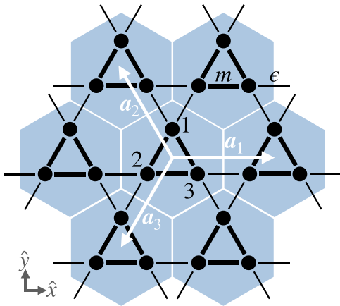
FIG. 6. Lattice vectors (white arrows), unit cell (blue hexagon), lattice sites (black dots), and hoppings (black lines) for the breathing kagome lattice model in Eq. (37). Strong hoppings inside the unit cell (weighted by m ) are indicated by thick lines while weak hoppings (weighted by \epsilon ), which connect different unit cells, are indicated by thin lines.
