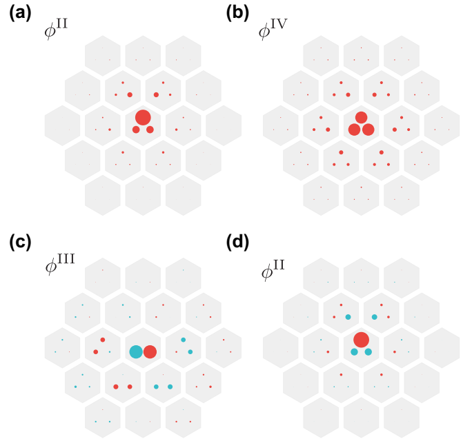
FIG. 8. Numerical in-gap breather profiles \phi_{(\mathbf{R},\alpha)} in the nonlinear breathing kagome lattice [Eqs. (12) and (37)] away from the molecular limit. In all plots, m = 1 ; in (a) and (d) \epsilon = 0.5 , while in (b) and (c) \epsilon = 0.25 ; additionally, g = -6 and \omega = -5.89 in (a), g = -4 and \omega = -3.34 in (b), g = -4 and \omega = -0.96 in (c), and g = +4 and \omega = 4.1 in (d). The area of the disks is proportional to the magnitude of the field and the red (teal) color represents a sign of +1 ( -1 ).
