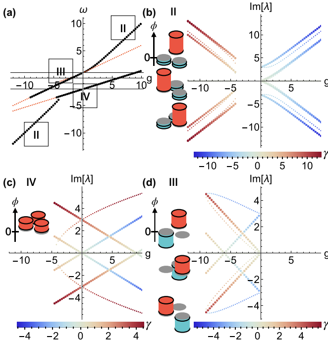
FIG. 7. Analytical molecular limit breather solutions in the nonlinear breathing kagome lattice [Eqs. (12) and (37)] for m = 1, \epsilon = 0 . (a) Breather frequencies derived in Sec. V B. The frequencies of linearly stable (unstable) breather solutions are shown with thick black (thin red) dots. The linear flat-band spectrum at \omega \in \{-2, 1, 1\} is indicated by gray horizontal lines. At g \lesssim -4 and g > 0 , there exist three stable, mostly on-site breather modes with C_2 eigenvalue \lambda^{(2)} = +1 and exchanged by C_3 symmetry (Type II). At fixed g , their stability eigenvalues shown in panel (b) all belong to Krein eigenvalues \gamma of the same sign, indicating stability away from the molecular limit. Here, nondegenerate (macroscopically degenerate) stability eigenstates are indicated by thin (thick) dots (see Sec. III B for details), and the curves terminate when the respective solution becomes unstable. At g \gtrsim -4.5 , one further stable breather with C_2 and C_3 eigenvalues \lambda^{(2)} = \lambda^{(3)} = +1 [Type IV, (c)] exists that continuously connects with the linear band at \omega = -2 . For -9.07m \lesssim g \leq 0 , three more stable two-site breathers with C_2 eigenvalue \lambda^{(2)} = -1 and exchanged by C_3 symmetry [Type III, (d)] exist within the gap that connect with the two degenerate bands at \omega = 1 .
