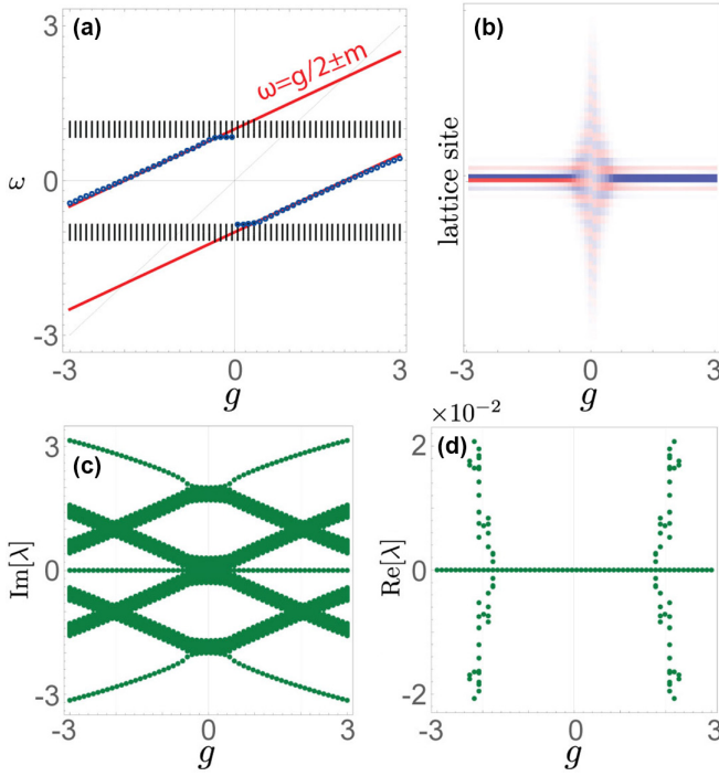
FIG. 5. Numerical in-gap breather solutions of Type (II, \pm ) in the nonlinear SSH chain [Eqs. (12) and (24)] with m = 1 and \epsilon = 0.15 . (a) Linear spectrum (black) and breather frequencies (blue). (b) Spatial profiles \phi_{(R,\alpha)} . Blue (red) color represents positive (negative) components. (c) and (d) Stability eigenvalues \lambda . Instabilities develop in the region |g| \approx 2m (absent in the molecular limit), where stability eigenvalues with opposite Krein eigenvalues collide [Figs. 1(c) and 1(d)].
