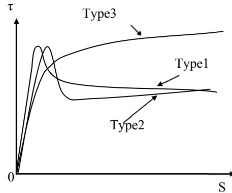
Fig. 2 Three kinds of load-slip curve
