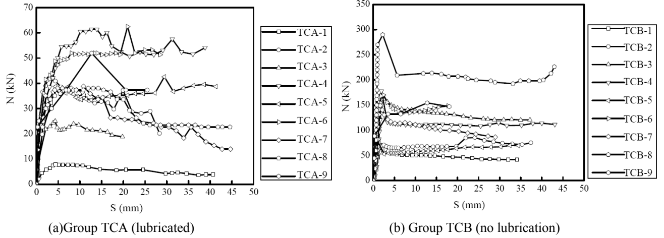
Fig. 7 Push-out load-slip curves for each specimen
