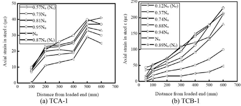
Fig. 8 Axial strains in narrow face of steel tubes along specimen lengths at different load levels
