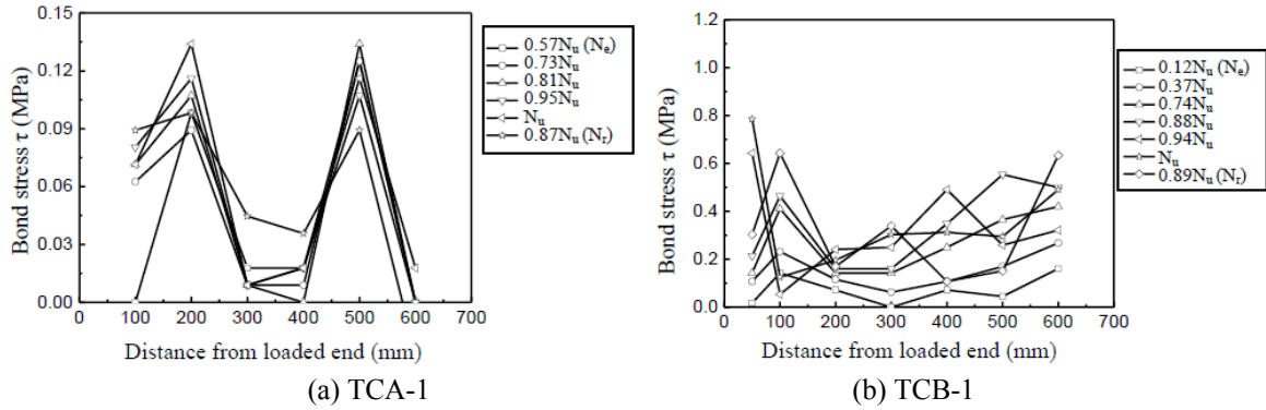
Fig. 11 Bond stress distribution in the narrow face of the steel tubes along specimen lengths at different load level
