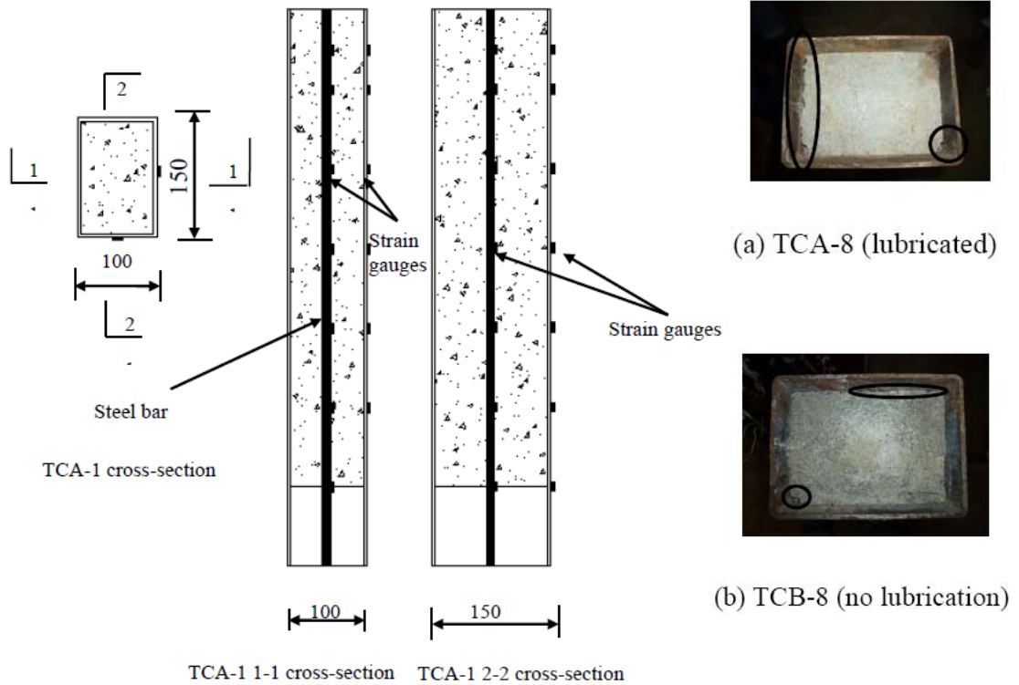
Fig. 5 Specimens details: TCA-1 (dimensions in mm)
