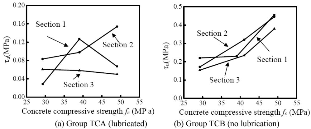
Fig. 15 Variation of average ultimate bond strength with concrete compressive strength
