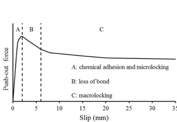
Fig. 1 Idealized response of push-out specimens
