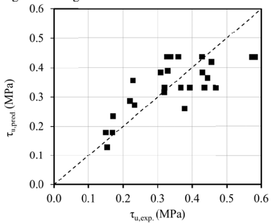
Fig. 19 Comparison of empirical equation with test data
