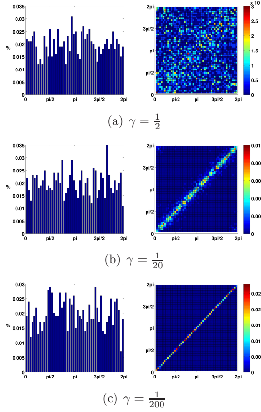
Figure 3: CL dynamics with N = 10^3 and three values of the parameter \gamma (from top to bottom: \gamma = 1/2 , \gamma = 1/20 , \gamma = 1/200 ). One and two particle equilibrium distributions (left and right respectively). Left: the horizontal axis is \theta \in [0, 2\pi] , the vertical axis is the distribution of \theta . Right: the square is the domain of (\theta_1, \theta_2) \in [0, 2\pi]^2 . The color coding indicates the 2-particle distribution.
