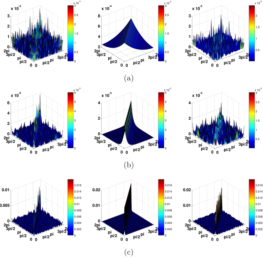
Figure 5: Perspective view of the equilibrium two-particle distribution of the CL dynamics as functions of (\theta_1, \theta_2) \in [0, 2\pi]^2 , with (a) \gamma = \frac{1}{2} ; (b) \gamma = \frac{1}{20} ; (c) \gamma = \frac{1}{200} . Left: numerical solution. Middle: analytical solution. Right: Difference between the numerical and analytical solution.
