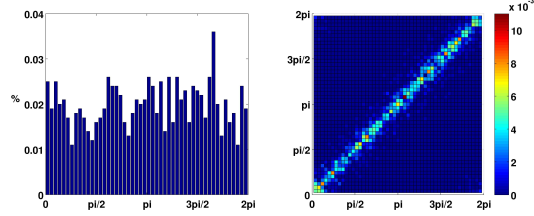
(a) N = 10^2
