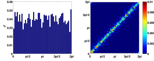
(c) N = 10^4
