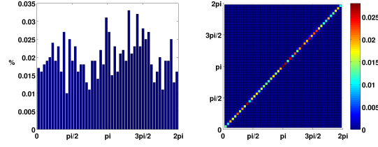
(b) N = 10^3
