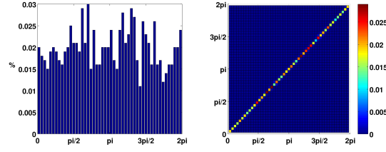
(c) N = 10^4
