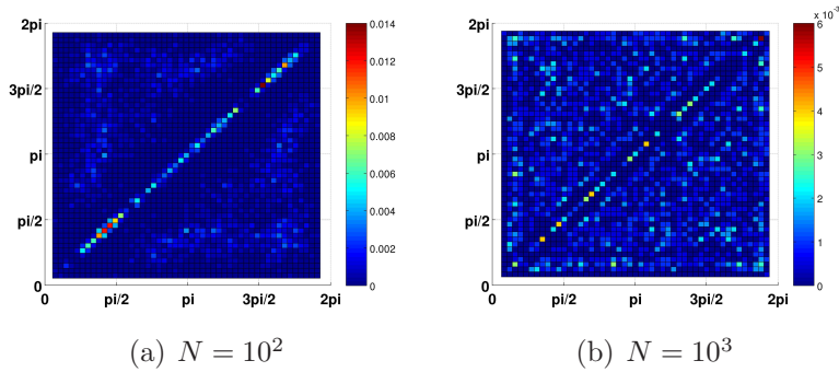
Figure 4: BDG dynamics with \gamma = 0.02 and \gamma' = 10\gamma and two values of the particle number (left: N = 10^2 ; right: N = 10^3 ). The two particle equilibrium distribution only is plotted. The square is the domain of (\theta_1, \theta_2) \in [0, 2\pi]^2 . The color coding indicates the 2-particle distribution.
