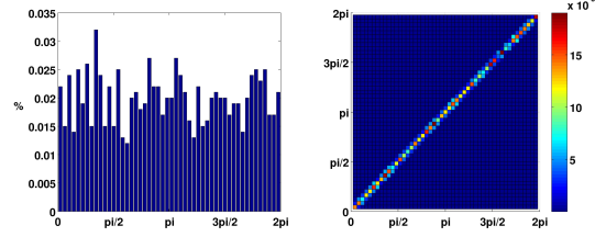
(a) N = 10^2
