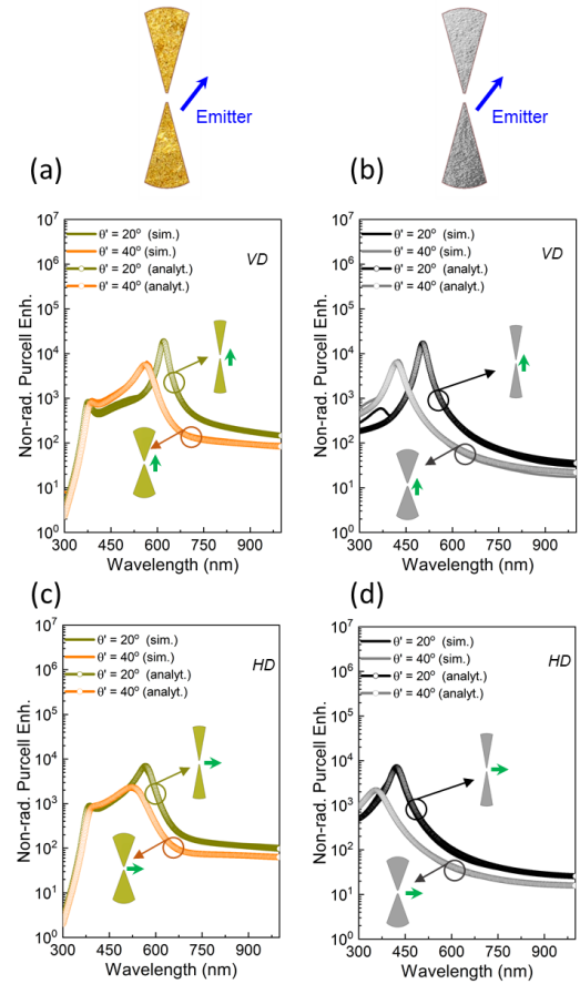
Figure 2. Analytical (symbols) and numerical (lines) results of the Non-radiative Purcell enhancement spectra for bowtie nanoantennas made of gold (left column) and silver (right column) with different values of \theta' when they are illuminated with a dipole nanoemitter under vertical (a,b) and horizontal (c,d) polarization.
