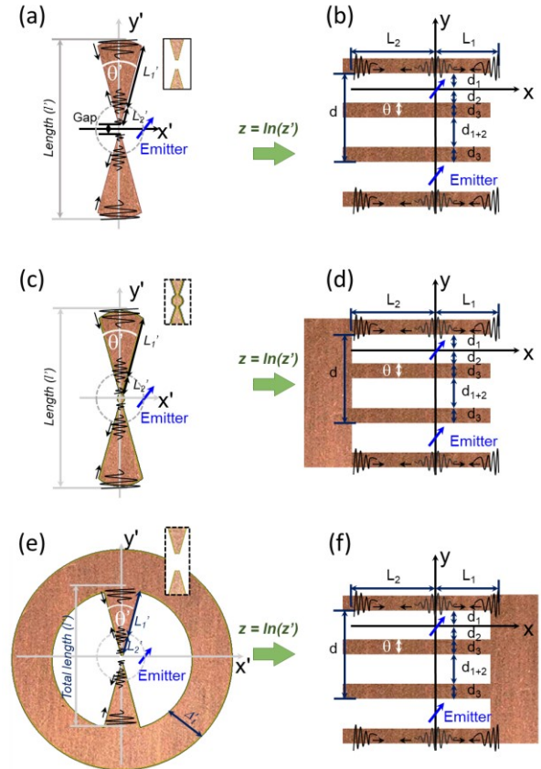
Figure 1. Schematic representation of the bowtie nanoantenna (a) diabolito nanoantenna (c) and nanocavity (e) along with their corresponding transformed space (right column).
