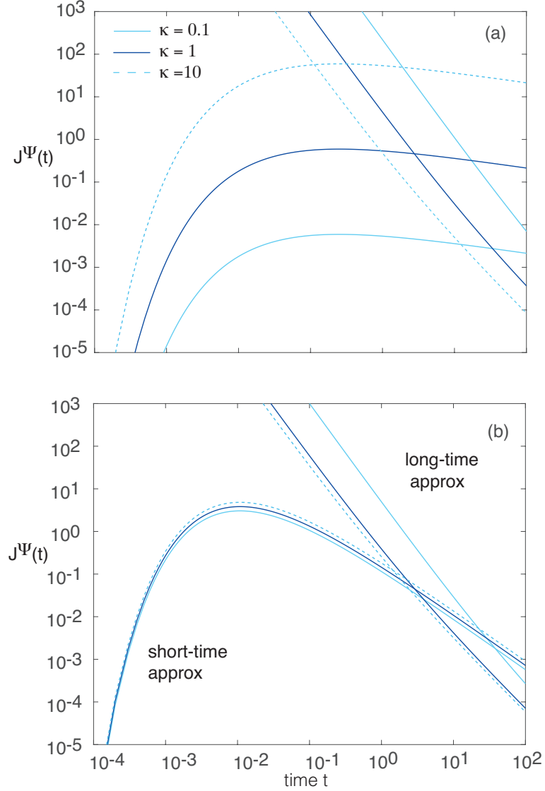
Figure 4. Same as Fig. 3 except that J\Psi(t) is plotted as a function of t for various values of \kappa with (a) \mu = 2 and (b) \mu = 0.1 .
