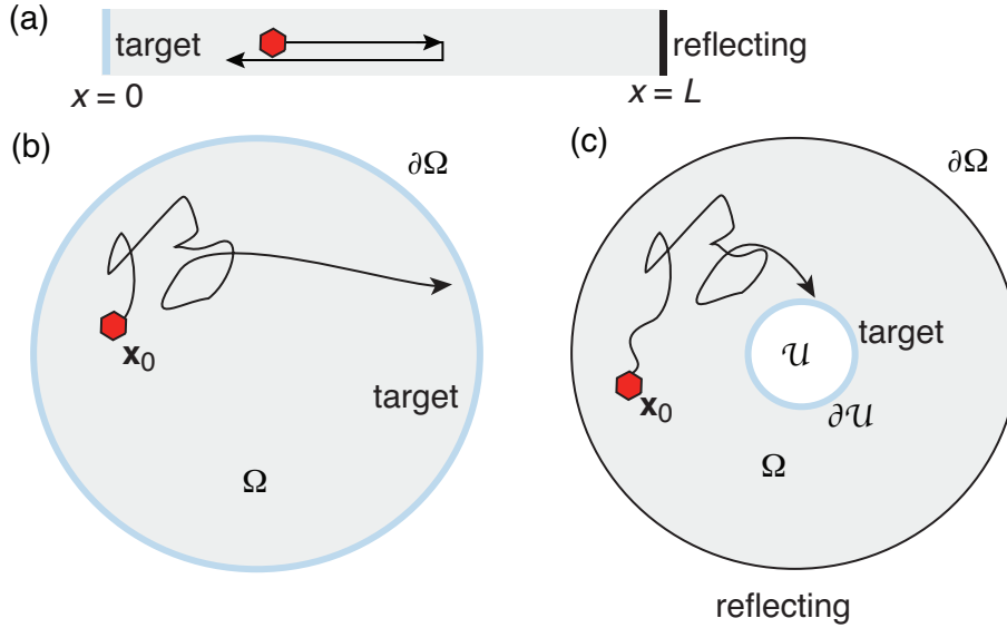
Figure 1. Diffusion in a bounded domain \Omega with a partially absorbing surface. (a) Finite interval with a partially absorbing boundary at x = 0 and a reflecting boundary at x = L . (b) Spherical domain \Omega with a partially absorbing surface \partial\Omega . (c) Annular domain with a reflecting exterior surface \partial\Omega and a partially absorbing interior surface \partial\mathcal{U} . Adsorption occurs at the surface \partial\mathcal{U} without the particle ever entering the interior of the trap \mathcal{U} .
