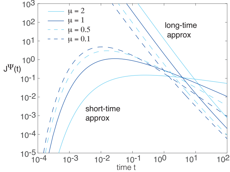
Figure 3. Fractional diffusion on the interval [0, L] with a partially absorbing boundary at x = 0 and a totally reflecting boundary at x = L . We plot the first two-terms in the asymptotic expansion (3.25) of the FPT density J^\Psi(t) for the gamma distribution (3.12) with \mathbb{E}[\ell] = \mu/\kappa = 1 and various values of \mu . We also show the corresponding short-time approximation (3.29). Other parameters are \alpha = 2/3 , K_\alpha = 1 , L = 1 , and x_0 = 0.75 .
