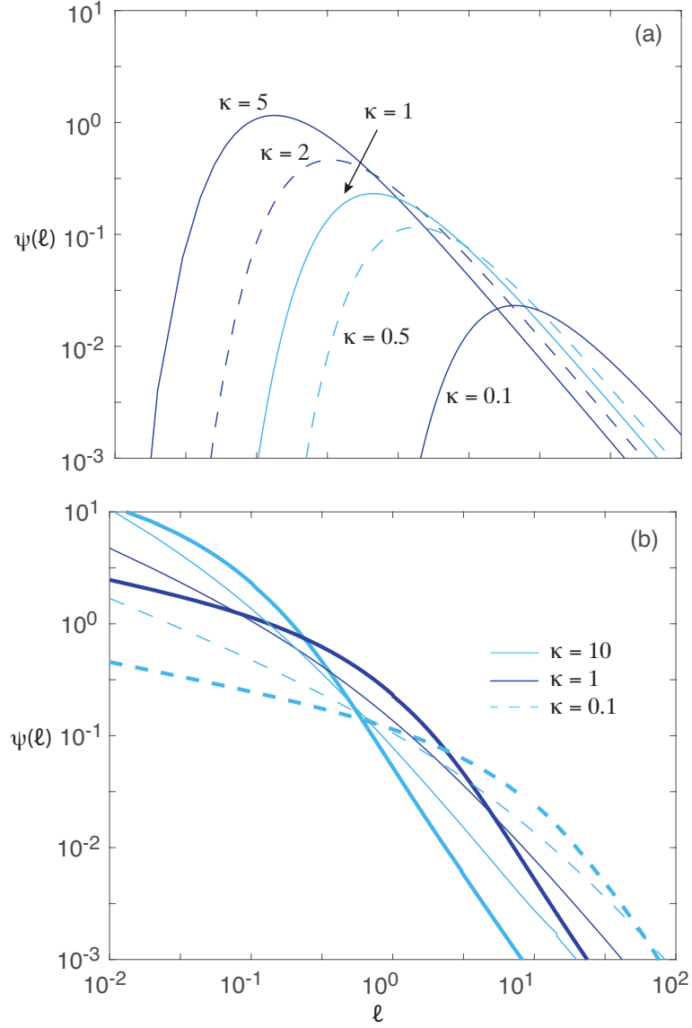
Figure 5. Two examples of a heavy-tailed distribution \psi(\ell) . (a) One-side Levy distribution for different values of \kappa . (b) Mittag-Leffler distribution for different values of \kappa with \mu = 0.5 (thin curves) and \mu = 0.75 (thick curves).
