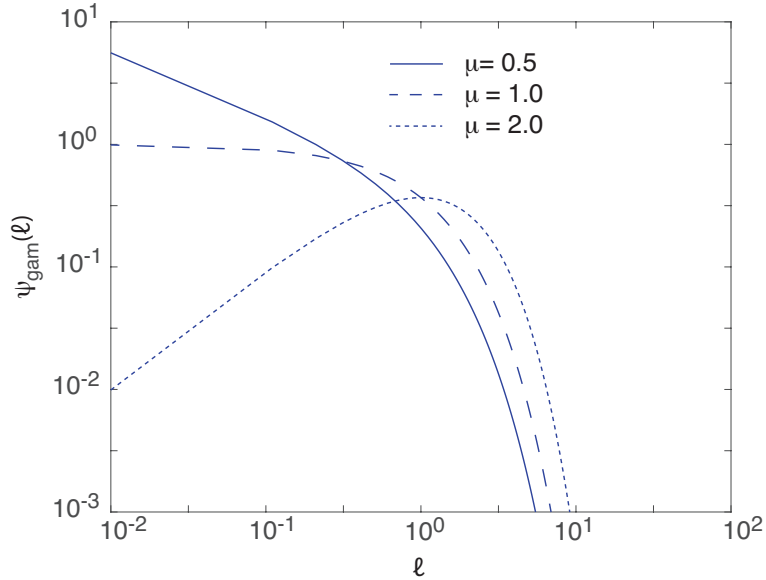
Figure 2. Plots of the probability density \psi_{\text{gam}}(\ell) as a function of the local time threshold for the gamma distribution with \kappa = 1 and various values of \mu .
