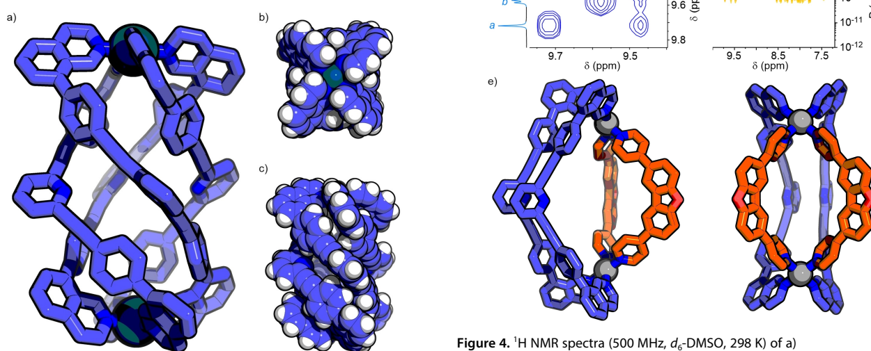
Figure 3. SCXRD structure of the \Lambda enantiomer of [\text{Pd}_2(2^{\text{Py}})_4]^{4+} a) from the side, with hydrogen atoms omitted for clarity, and space-fill models shown b) down the Pd...Pd axis, and c) from the side.
