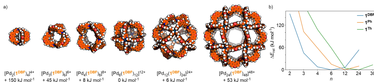
Figure 7. a) Geometry-optimised (GFN2-xTB) structures of [Pd_n(1^{DBF})_{2n}]^{2n+} cages with their relative single point energies per Pd(II) ion, \Delta E_{rel} (GFN2-xTB). b) \Delta E_{rel} versus topology nuclearity, n , for ligands 1.
