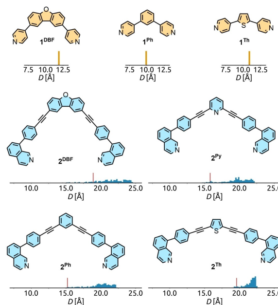
Figure 2. Structures of diverging ligands 1 and converging ligands 2 . Each structure includes the distribution of N–N distances over conformers generated (see below) within 5 \text{ kJ mol}^{-1} of the lowest energy conformer. For ligands 2 , conformers closest to the “as-drawn” planar structure indicated by red lines.
