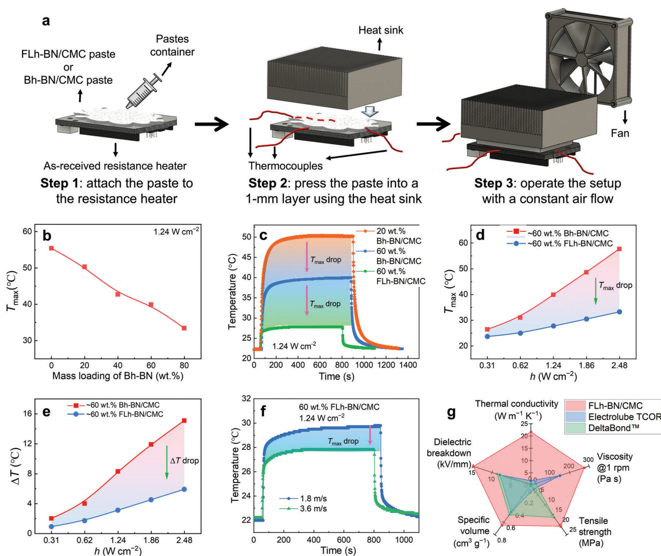
Figure 6. a) Configuration and assembly of the custom-built temperature monitoring setup, b) the T_{\max} performance of the Bh-BN/CMC at different mass loadings, c) real-time temperature evolution of the heater using different thermal pastes at 1.24 \text{ W cm}^{-2} , d) T_{\max} , and e) \Delta T of the 60 wt.% FLh-BN/CMC compared with that of the 60 wt.% Bh-BN/CMC, at different heat generation densities; f) real-time temperature evolution of the heater using the FLh-BN/CMC paste at different air convection rates, at 1.24 \text{ W cm}^{-2} and g) the radar plot comparing key parameters of the FLh-BN/CMC paste compared to commercial thermal pastes. [86,87]
