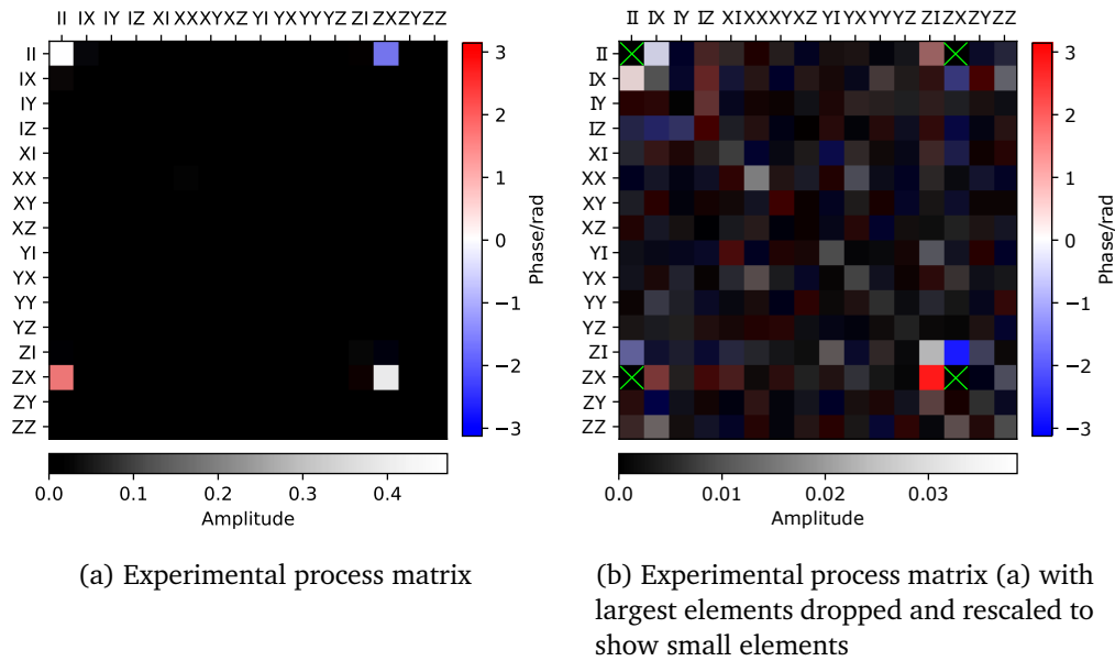
Figure 5: (a) Quantum process matrix extracted from the application of a cross-resonance interaction optimized for the gate \exp(i\pi/4ZX) using Bayesian optimization and implemented on the ibmq_paris quantum device. The ideal process matrix consists of the four terms which dominate the optimized process matrix, each with magnitude 1/2 . (b) The same optimized process matrix as (a), but with the four largest elements (corresponding to \chi elements indexed by products of \mathbb{I}\mathbb{I} and XZ ) set to 0 and the color bar rescaled to show the magnitude of the less significant terms. The optimized process matrix has some small residual unwanted terms and the magnitudes are slightly suppressed, but nevertheless yields a fidelity of approximately 0.93 even without any measurement error mitigation.
