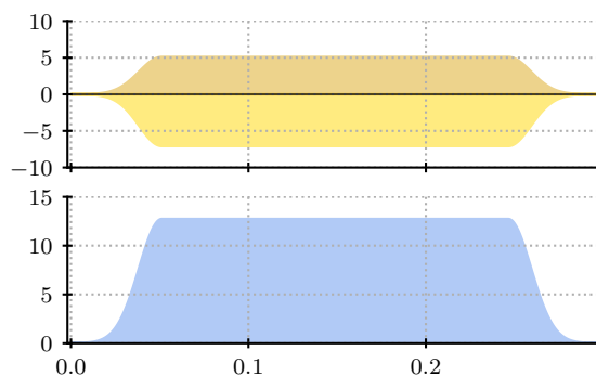
Figure 4: Plot showing the requested drive pulse amplitudes used in the optimization of the single application of the cross-resonance drive outlined in Sec. 3.3, with the yellow plots corresponding to cross-resonance pulses and the blue plots corresponding to the single qubit resonant pulses needed to counteract the spurious single qubit \mathbb{1}X term from the cross-resonance interaction and where the light and dark portions of the plots correspond to the real and imaginary components of the pulses respectively. This set of pulses corresponds to the highest fidelity observed in the optimization. The phase of the cross-resonance drives is non-zero due to the phase calibration outlined in Sec. 3.1. The Z\mathbb{1} term may be corrected using a virtual Z rotation [54] and so is not represented in this plot of physical pulses.
