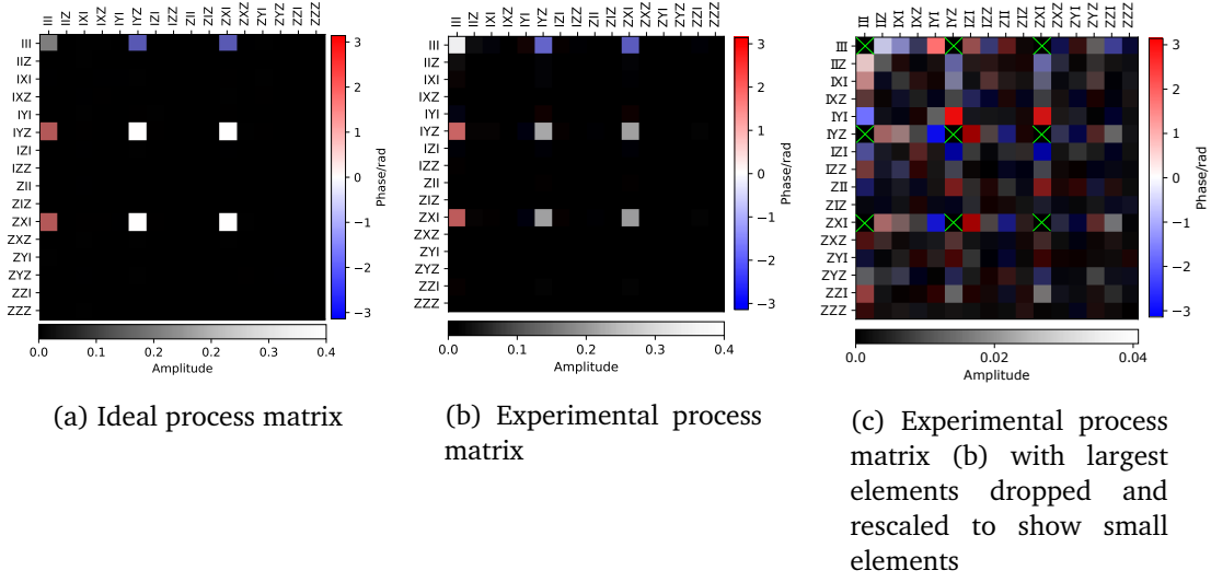
Figure 6: Experimental results for the optimization of an \exp(i\pi/4(ZX1 + 1YZ)) gate: (a) shows the ideal process matrix for the gate (showing only elements that can be generated by Eq. (5)) and (b) shows the experimental process matrix for the optimal drive parameters obtained through BO, implemented on the ibm_oslo quantum device. (c) shows the same experimental results as (b) but with the 9 largest terms (corresponding to \chi elements indexed by products of 111, 1YZ and ZX1 ) set to 0 (indicated by green crosses) and the color bar rescaled to show the magnitude of the less significant terms. Only terms that can be generated by the noisy cross-resonance and single qubit drive pulses are shown for clarity; the full process matrices including the dropped terms are shown in Appendix B. The qualitative features of the process matrix are accurately obtained, with the amplitude of the observed terms slightly reduced from the ideal matrix. Additionally, the Rabi angle is slightly misaligned, leading to a final process fidelity of 82%.
