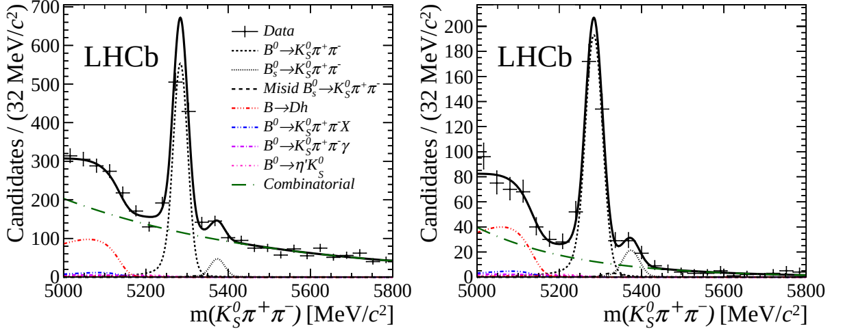
Figure 2: Distribution of K_S^0 \pi^+ \pi^- mass for signal candidates with fit results overlaid for (left) downstream and (right) long categories. The data are described by the black points with error bars. The overall fit is represented by the solid black line. The B^0 and B_s^0 signal components are the black short-dashed and dotted lines. The misidentified B_s^0 decay is the black dashed line, respectively. The partially reconstructed backgrounds are the red triple-dotted line ( B \rightarrow Dh ), the blue triple-dotted line ( B^0 \rightarrow K_S^0 \pi^+ \pi^- X ), the violet dash single-dotted line ( B^0 \rightarrow \eta' K_S^0 ) and the pink short-dash single dotted line ( B^0 \rightarrow K_S^0 \pi^+ \pi^- \gamma ). The combinatorial background is the green long-dash dotted line. Some of the contributions are small in the figures.
