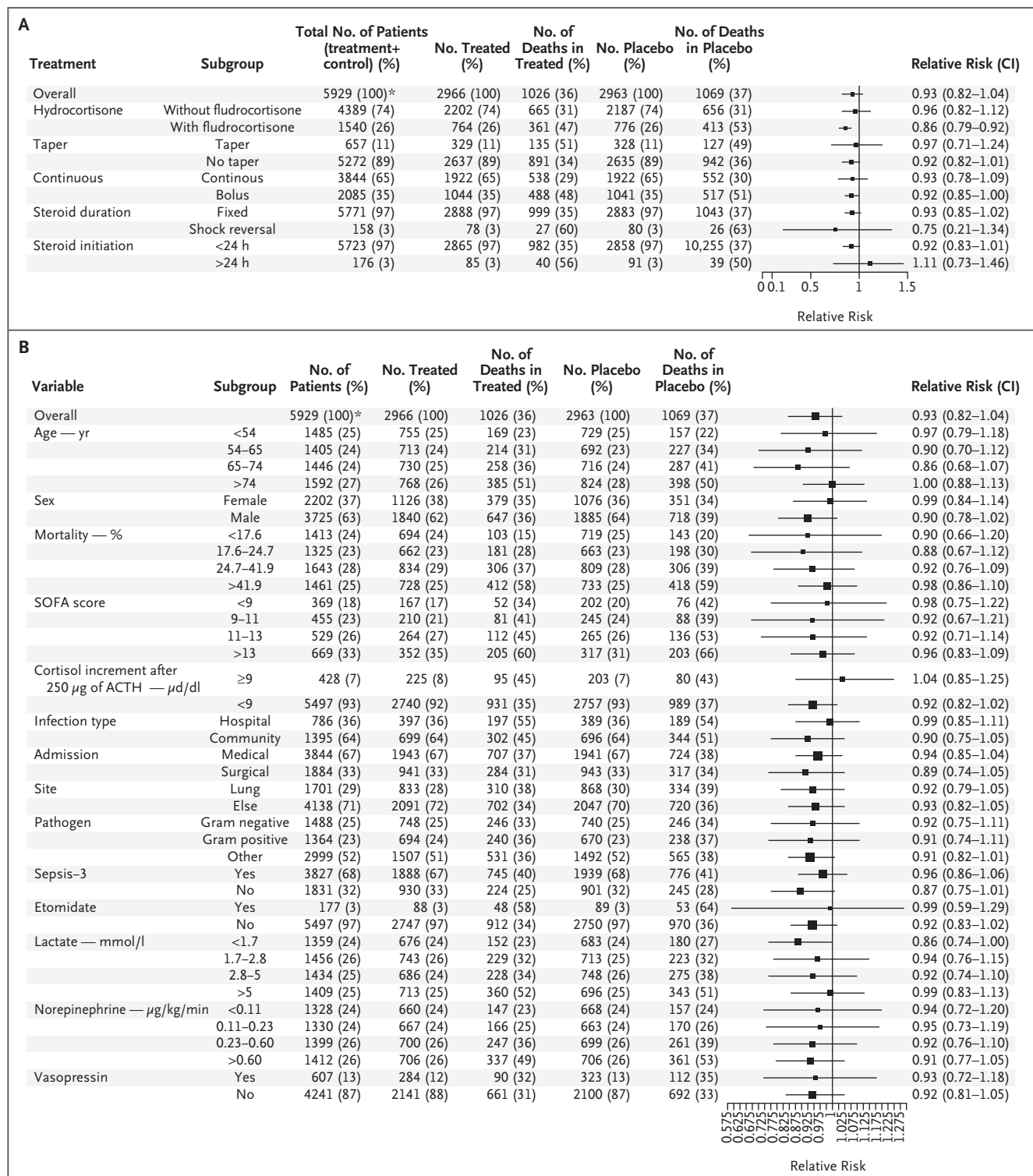
Figure 2. Forest Plot for the Association between Steroid and 90-Day Mortality.
