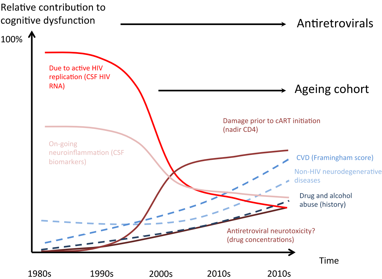
Figure 1. The hypothetical changing aetiology of cognitive impairment in those with HIV (and how it may be possible to assess their contribution in clinical studies).
