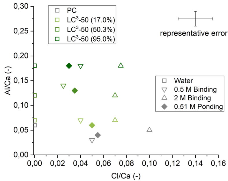
Figure 18 Chloride adsorption on C-A-S-H measured by SEM-EDX for binding isotherm samples (in water, 0.5 M and 2 M NaCl) and ponding test samples (0.51 M NaCl)
