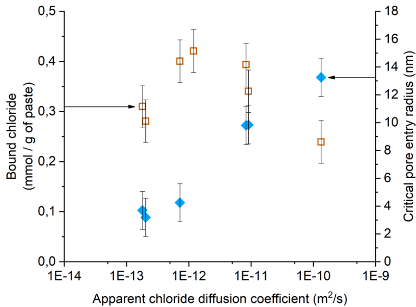
Figure 13. Correlation between the bound chloride, the critical pore entry radius with the apparent chloride diffusion coefficient.
