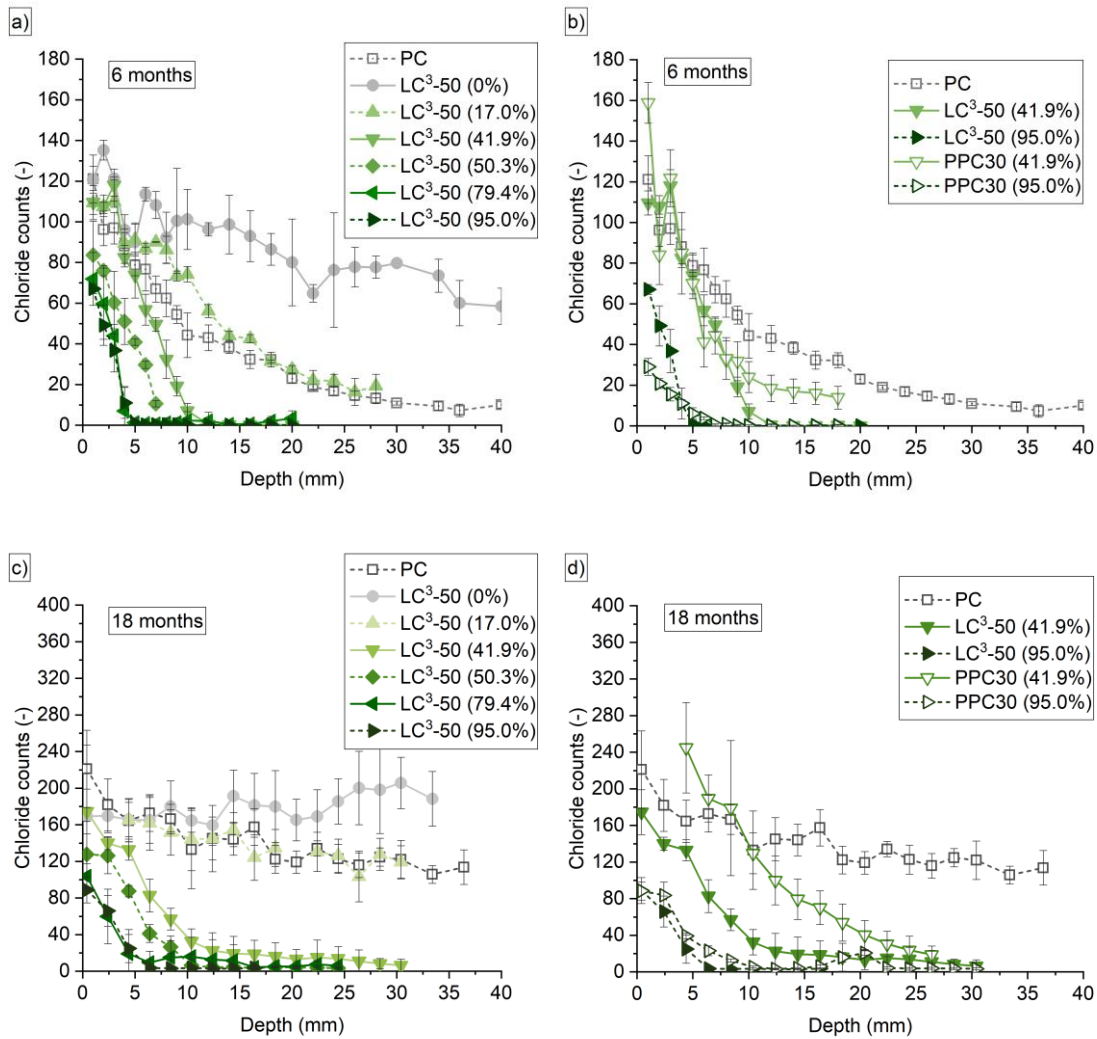
Figure 4 Profiles of total chloride for pastes measured using \mu -XRF after 6 (a,b) and 18 months (c,d) of exposure to 3 wt.% NaCl solution.
