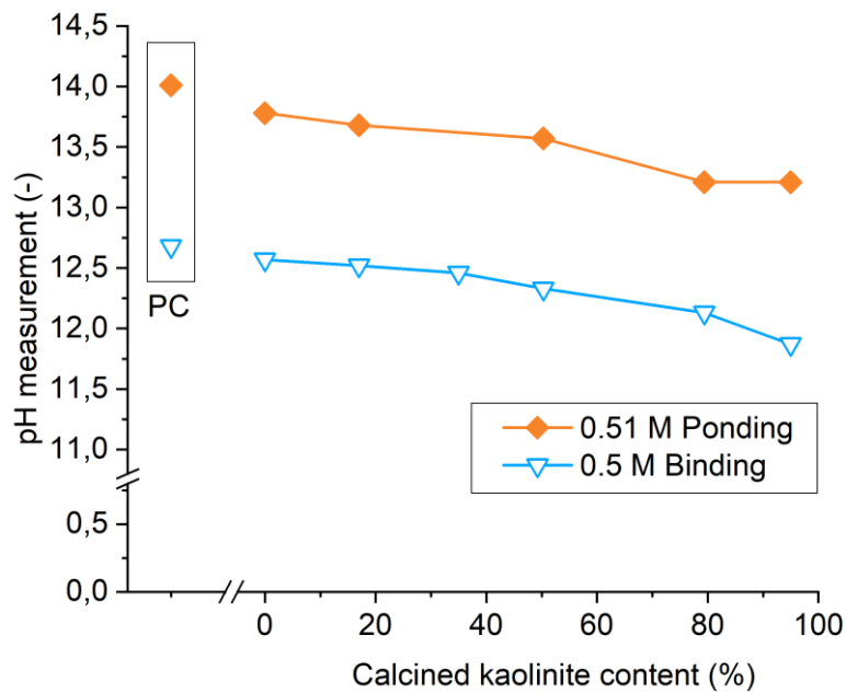
Figure 17 pH measurement of ponding test and binding test for similar NaCl concentration
