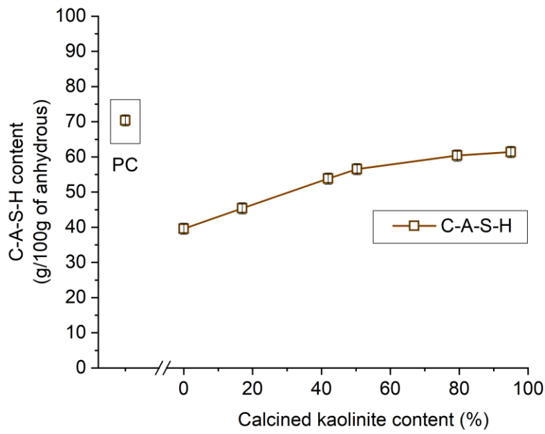
Figure 15 Amount of C-A-S-H for PC and the different LC 3 -50 blends
