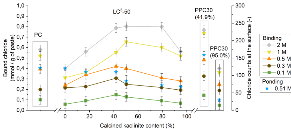
Figure 8 Total bound chloride as a function of clay grade in LC 3 -50 and PPC30 pastes after exposure to 0.1 to 2 M NaCl solutions
