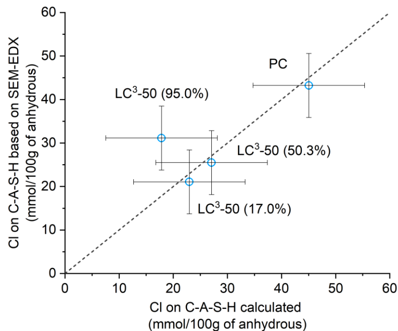
Figure 12 Amount of adsorbed chloride on C-A-S-H determined experimentally by SEM-EDX and calculated as the difference of the total bound chloride and the chloride in Friedel's salt
