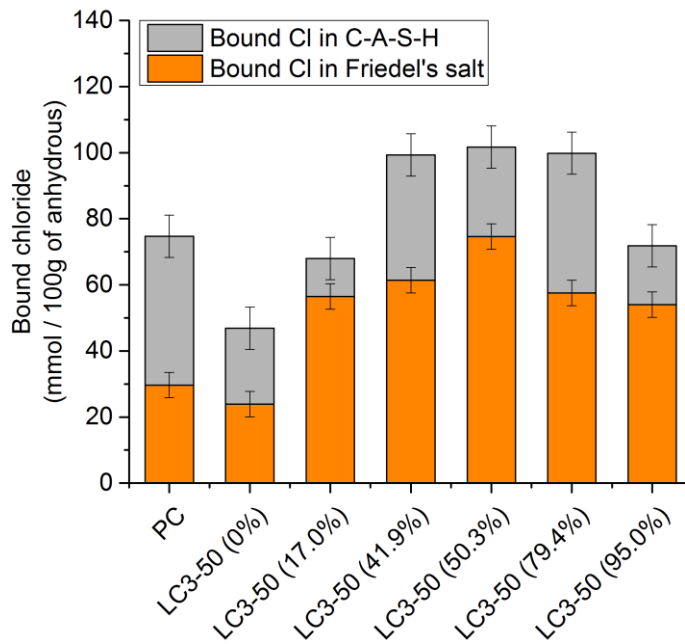
Figure 10 Distribution of bound chloride between C-A-S-H and Friedel's salt in PC and in the different LC 3 -50 pastes after exposure to 2 M NaCl solution
