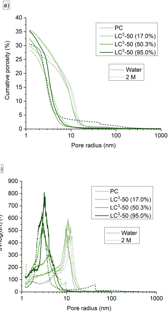
Figure 6 Porosity distribution of PC and LC3-50 (17.0%), (50.3%) and (95.0%) paste samples after 6 m exposure to water or 2 M NaCl solution
