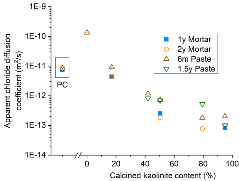
Figure 5 Apparent diffusion coefficients for PC and LC 3 -50 mortar and paste samples, calculated using Fick's law of diffusion
