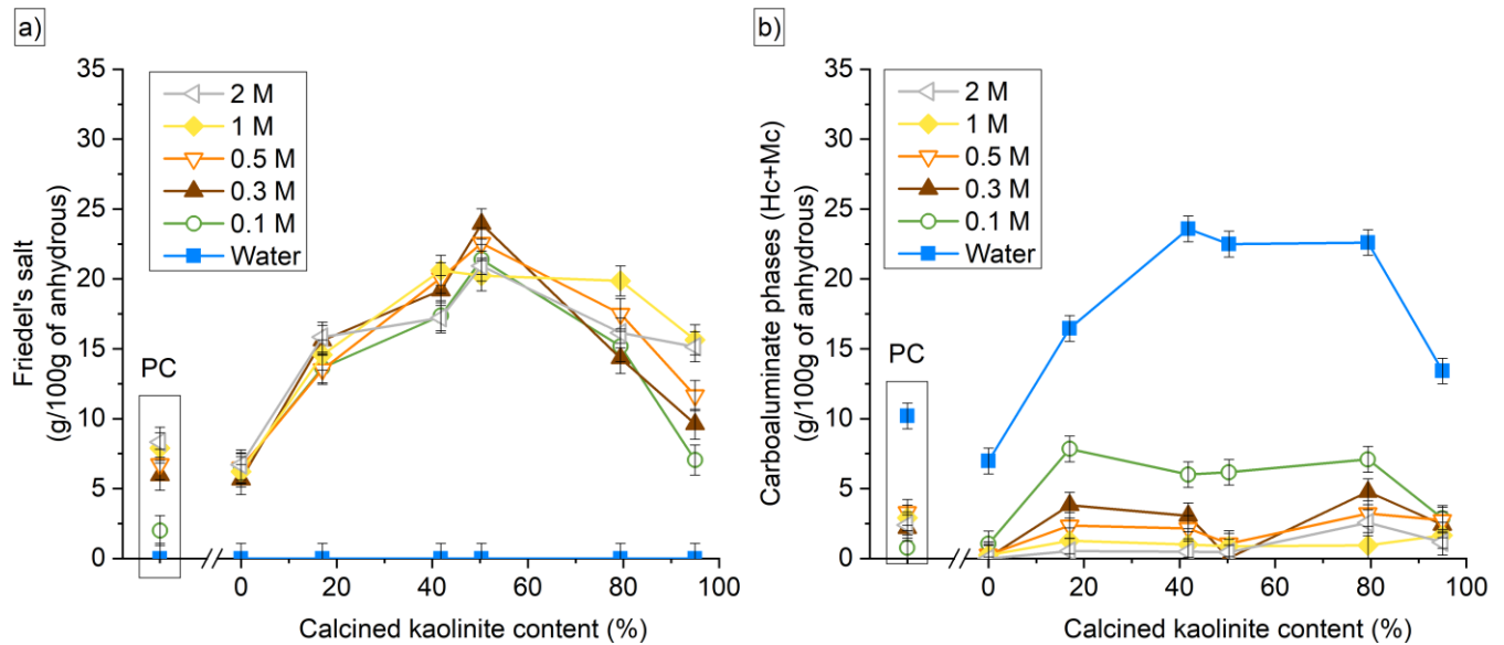
Figure 9 Amount of Friedel's salt (a) and carboaluminate (b) phases in PC and LC 3 -50 pastes
