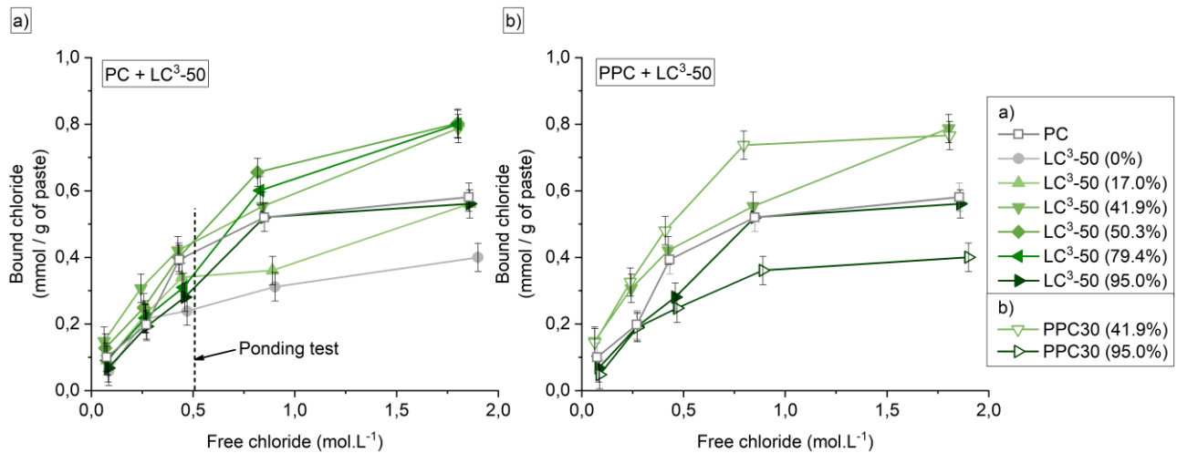
Figure 7 Binding isotherm curves for LC 3 -50 and PPC-30 pastes
