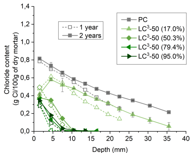
Figure 3 Total chloride profiles for PC and LC 3 mortars after 1 and 2 years of exposure to 3% NaCl ponding solution
