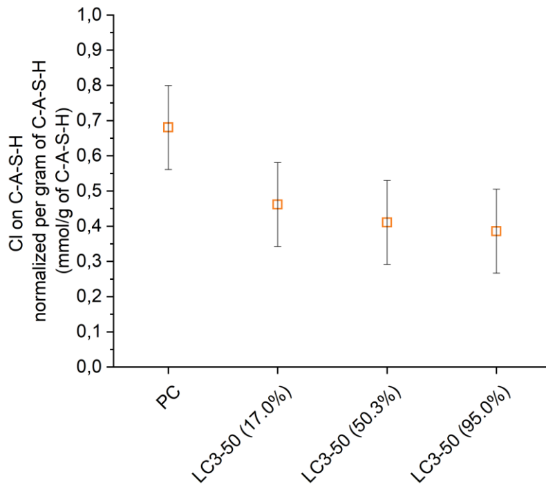
Figure 16 Chloride adsorption on C-A-S-H normalized per gram of C-A-S-H for PC and LC3-50 blends.
