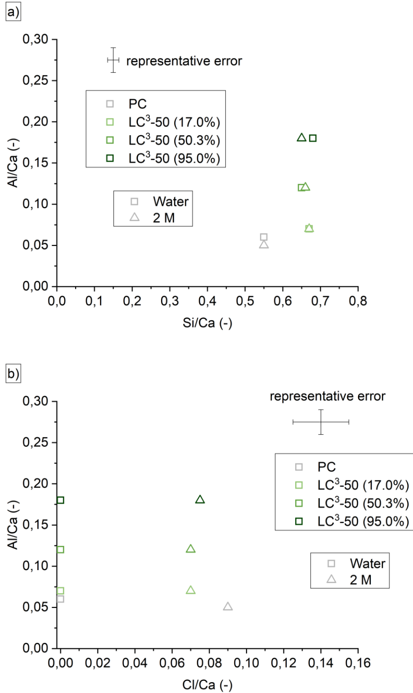
Figure 11 SEM-EDS analysis of PC and LC³ pastes, (a) showing that the Si/Ca and Al/Ca of C-A-S-H stays intact after exposure to chloride ions, and (b) indicating binding of chloride in C-A-S-H after exposure to 2 M NaCl solution
