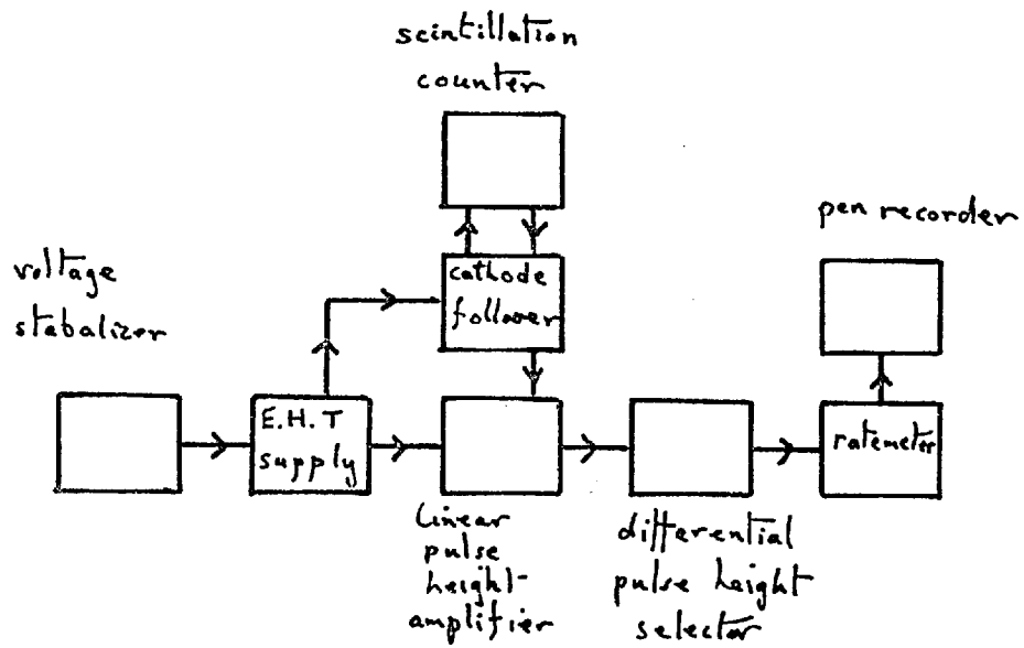
Fig. 3.6: Block diagram of counting apparatus.
