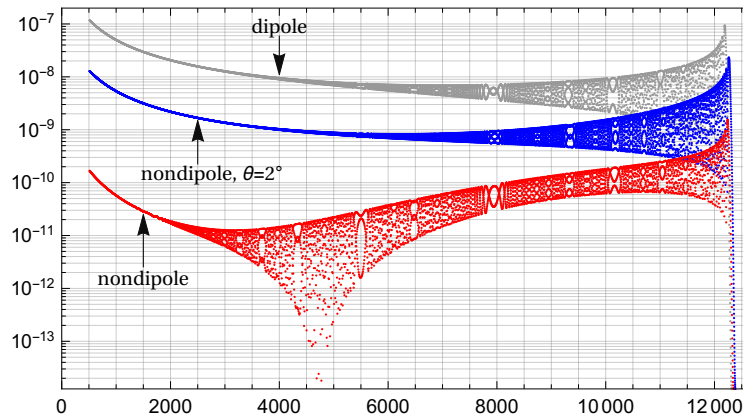
Figure 9.5: Above-threshold harmonic emission for a \text{Ne}^{6+} ion in an 800 nm field of intensity I = 10^{17} \text{ W/cm}^2 , calculated in the uniform approximation using the first pair of quantum orbits, and discarding z -polarized harmonics. For linear polarization, the dipole-approximation emission drops by two orders of magnitude when nondipole effects are included, but adding in even a small forwards ellipticity at \theta = 2^\circ can help recover the harmonic emission.
