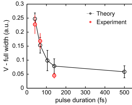
Figure 6.16: Variation of the width of the VLES V shape in Fig. 6.15 with respect to variations in the pulse length, showing good agreement between CTMC simulations and experiment. Figure excerpted from Ref. 166.
