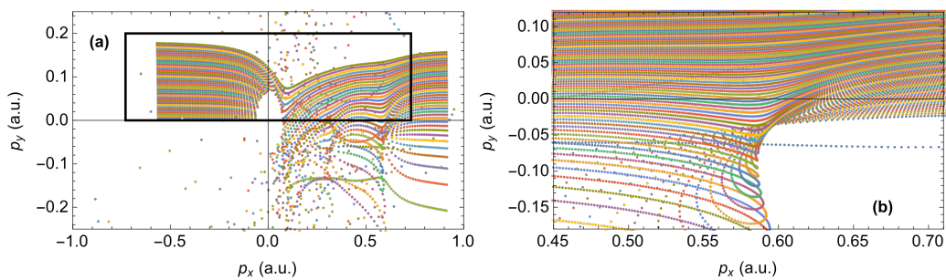
Figure 6.11: Dynamical map of electrons ionized from argon by a 1.5 \times 10^{14} \text{ W/cm}^2 field at 2 \mu\text{m} , taking a regular grid in momentum space to a complicated shape [177]. The decrease in width compared to the non-Coulomb case (black rectangle) showcases the known Coulomb focusing, but near the soft recollision at p_x \approx 0.61 \text{ a.u.} the trajectories are sent to an opposite transverse momentum p_y , forming the caustic shown in (b), which then accumulates electrons to form an LES peak in the photoelectron spectrum. Figure excerpted from Ref. 177.
