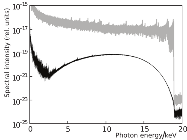
Figure 9.1: Quenching by the Lorentz force of the harmonic emission of helium under a six-cycle pulse at 8\mu\text{m} and 10^{15}\text{ W/cm}^2 , as compared to the same conditions under the dipole approximation, shown in gray. Figure excerpted from Ref. 299.
