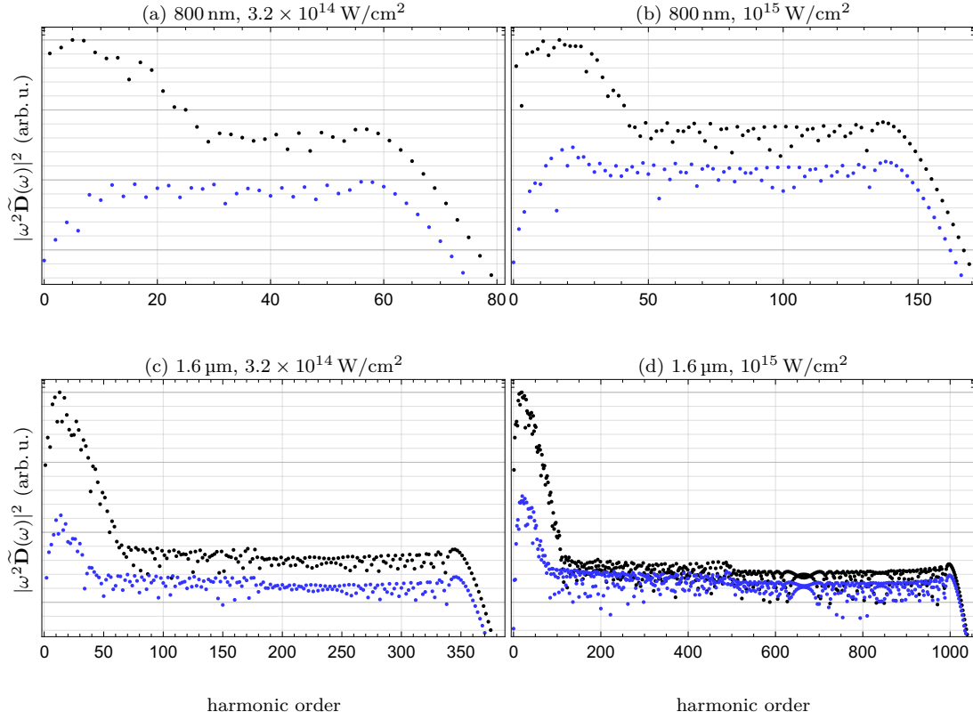
Figure 9.6: Harmonic spectra (● odd and ● even harmonics) produced in helium in the non-dipole regime for intensities of 3.2 \times 10^{14} and 10^{15} W/cm 2 and monochromatic fields of 800 nm and 1.6 \mu\text{m} at a beam half-angle of \theta = 4^\circ , on arbitrary scales and eliminating z -polarized harmonics. The intensity ratio between even and odd harmonics varies from \sim 10^{-3} for 800 nm drivers to \sim 10\% for strong mid-IR fields at 1.6 \mu\text{m} and 10^{15} W/cm 2 . The required sources are on the high end of intensity at the given wavelengths, but they are already accessible with current technology.
