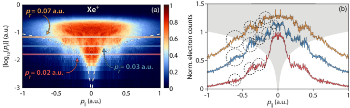
Figure 6.7: Momentum map (a) for the ionization of xenon in a 3.1\ \mu\text{m} pulse of intensity 4 \times 10^{13}\ \text{W}/\text{cm}^2 [167], showing clear LES but slightly muddled VLES V-shape and NZES peak. Line-outs at several different transverse momenta p_{\perp} produce longitudinal profiles with distinct LES peaks shown inside dashed circles in (b). The gray region in (b) is a rough approximation of the features excluded by the TOF acceptance cone, shown as the white dashed line in (a) as in Fig. 6.4. The data have been symmetrized about p_{\parallel} = 0 . Figure excerpted from Ref. 167.
