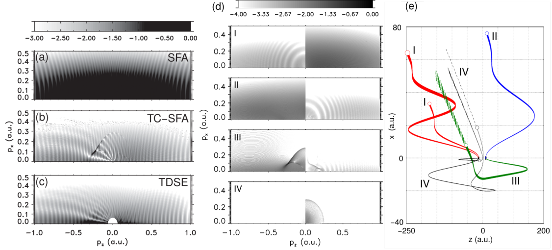
Figure 6.12: Photoelectron momentum distributions from argon ionized by a 2\mu\text{m} field at 10^{12}\text{W}/\text{cm}^2 [180], via standard SFA (a), a full TDSE simulation (c), and a CCSFA (here named TC-SFA) calculation (b). The CCSFA result provides a good match to the full TDSE, while still providing an intuitive trajectory picture. Specifically, the ‘cut’ at the LES range in (b) can be directly associated with a caustic, coming from trajectory type III as per (e), where the electron approaches the ion at low speed, changing the sign of its transverse momentum. Figure excerpted from Ref. 180.
