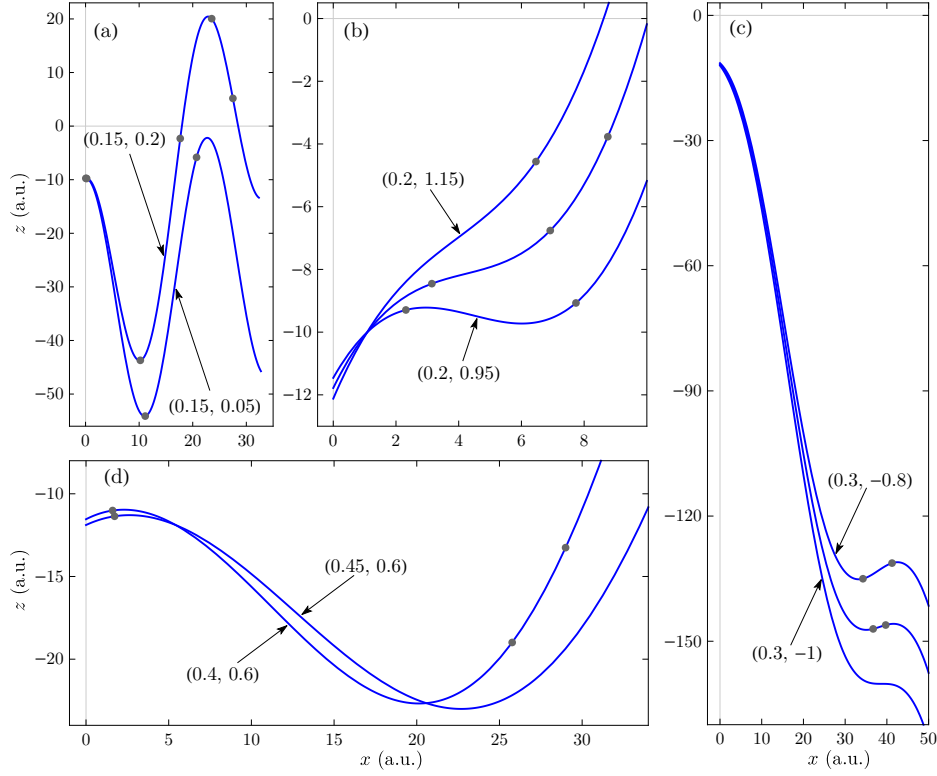
Figure 5.9: Classical trajectories from near the critical points marked a-d in Fig. 5.8, where the closest-approach roots of (5.15) can merge and disappear, indexed by their reduced momentum ( \omega p_x/F, \omega p_z/F ). The dots show closest-approach points, which satisfy (5.15) and for which the tangent to the trajectory is orthogonal to the radius vector. In the neighbourhood of a soft recollision, (a), an inward turning point turns into an outward turning point flanked by closest-approach points as the momentum increases. In (b) and (c) two turning points, a maximum and a minimum of \mathbf{r}_{cl}(t)^2 , merge and disappear as p_z goes past the oscillation amplitude F/\omega , either in the positive (b) or negative (c) direction, so v_z no longer changes sign and no turning points occur. Similarly, as the transverse momentum p_x increases in (d) the x component of the velocity becomes too great for the tangent to be orthogonal to the radius vector; at that point a maximum and minimum of \mathbf{r}_{cl}(t)^2 merge and disappear, leaving \mathbf{r}_{cl}(t)^2 to grow monotonically.
