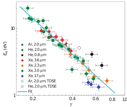
Figure 6.14: Scaling of the upper edge energy E_H of the LES structure as measured by Blaga et al. [157] for multiple target species and wavelengths, over varying intensities. The scaling is essentially universal, varying with the Keldysh parameter as E_H \propto \gamma^{-2} . Figure excerpted from Ref. 157.
