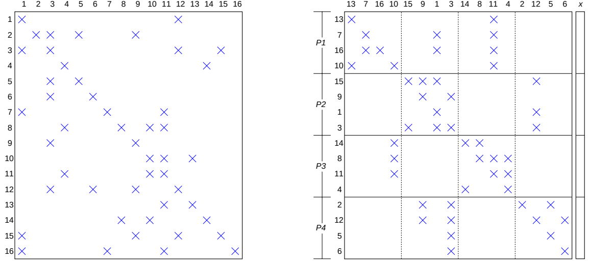
Fig. 1. A 16 \times 16 non-symmetric sparse matrix \mathbf{A} (left) and corresponding 4-way hypergraph partition (right) with corresponding partitions of a vector \mathbf{x} .
