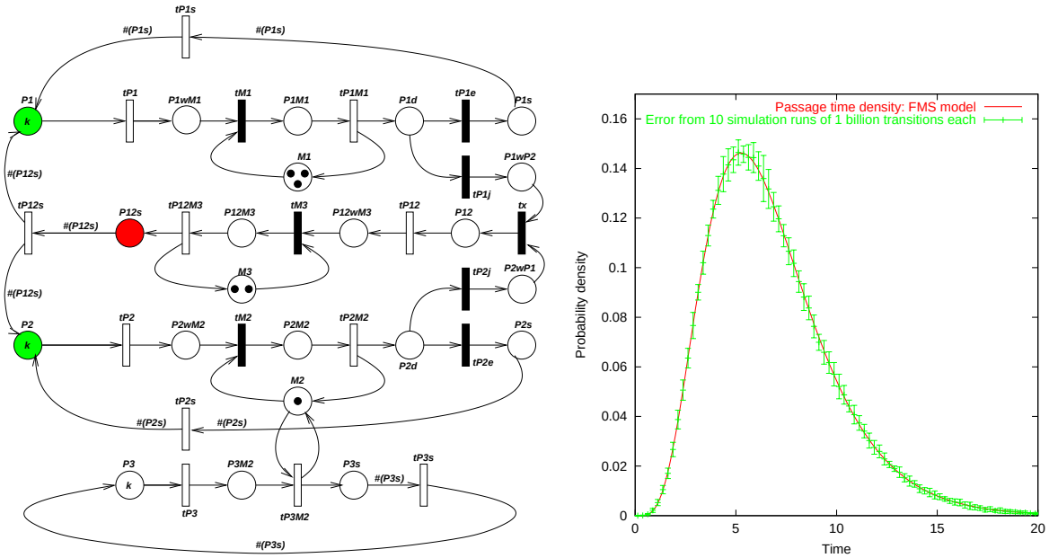
Fig. 3. The Flexible Manufacturing System (FMS) GSPN [15] (left) and corresponding numerical and simulated passage time densities for the time taken to produce a finished part of type P12 starting from states in which there are k = 7 unprocessed parts of types P1 and P2 (right).
