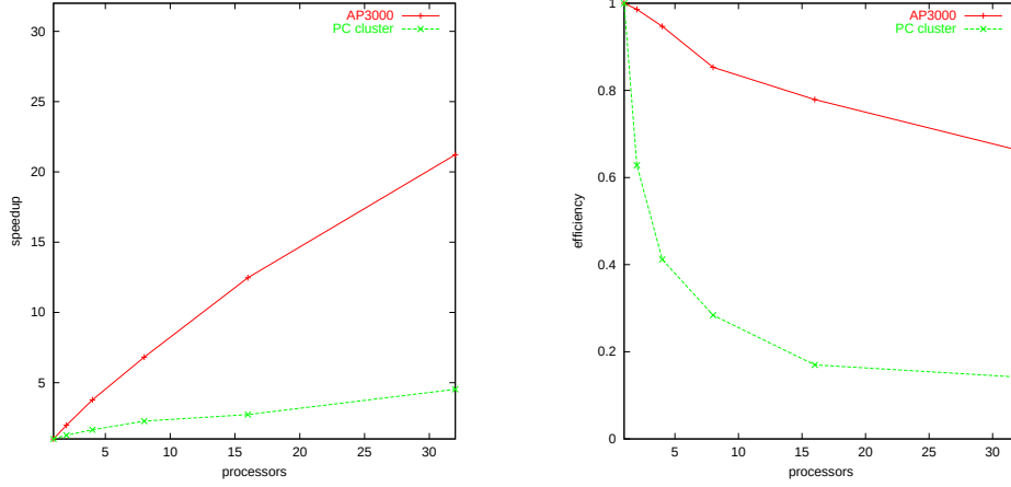
Fig. 4. Speedup (left) and efficiency (right) for the FMS model with k = 7 on the AP3000 and a PC cluster.
