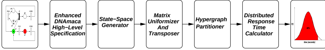
Fig. 2. HYDRA tool architecture.
