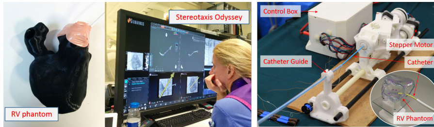
Fig. 5: The two robotic catheter experimental setups: (left) with the Stereotaxis Niobe ® and (right) with the new tele-operated robotic catheter. The top left of the RV phantom corresponds to the RV outflow and the top right corresponds to the tricuspid valve.
