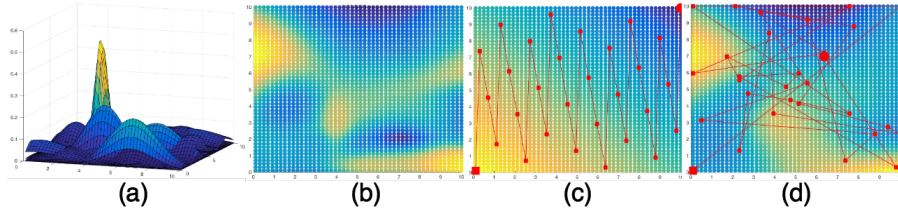
Fig. 3: Experiment setting on an example trial with 20 random Gaussian mixtures. (a) The randomly generated Gaussian mixtures. (b) The ground-truth values generated from (a). (c)(d) The mapping sequences from geometry method and the IE method and their estimated colour-coded grid values. The sequence starts from the red square and ending at the large red circle. The estimated values of (d) are closer to the ground-truth values in (b) than (c).
