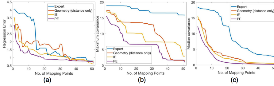
Fig. 6: The learning and uncertainty curves of different methods on dataset 11 for the expert mapping (blue), geometry with distance only (red), PE strategy (purple) and IE strategy (yellow). (a) shows the mean L1 error of the estimated values on all vertices. (b) and (c) show the maximum and median uncertainty over the unobserved vertices during mapping, respectively. In all, the IE method produced the fastest decrease in both the regression error and uncertainty.
