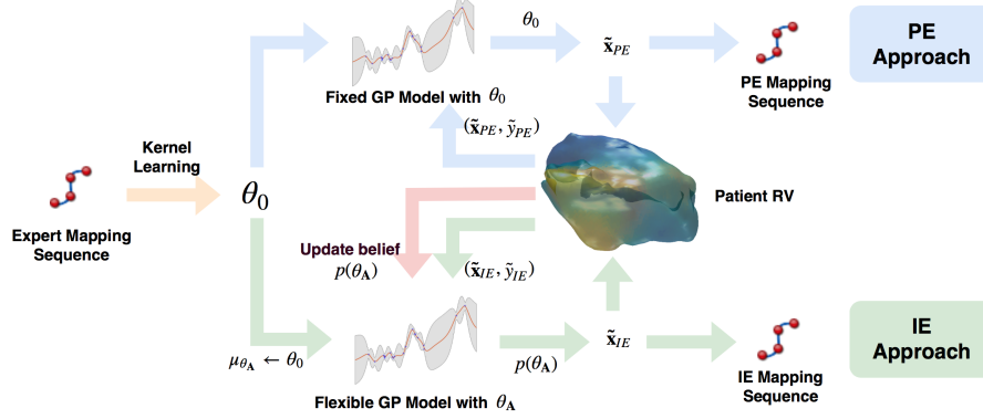
Fig. 2: Illustration of the PE and IE approaches. While both take new observations from the RV to output new mapping points from the GP, IE constantly refines the GP kernel hyperparameter \theta_A with the observation.
